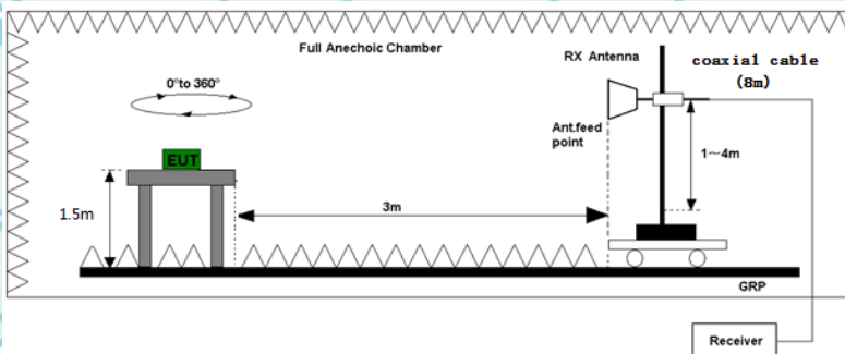
Above 1GHz
