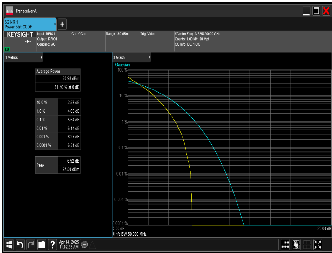
n78 SCS=30kHz DFT_QPSK BW=50MHz Channel=651666 RB=128 @0
