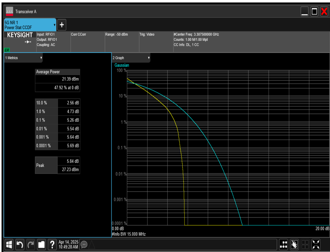
n78 SCS=30kHz DFT_QPSK BW=15MHz Channel=620500 RB=36 @0
