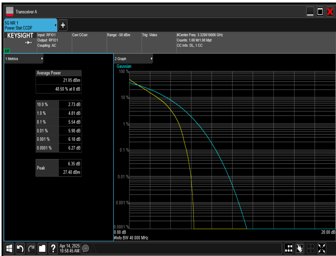
n78 SCS=30kHz DFT_QPSK BW=40MHz Channel=621334 RB=100@0
