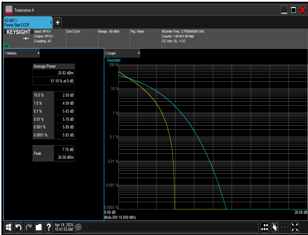
n78 SCS=30kHz DFT_QAM64 BW=90MHz Channel=636666 RB=240 @0
