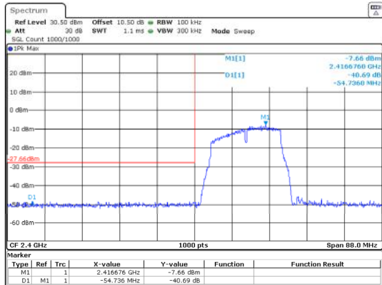
802.11g_2412MHz_Chain 1
