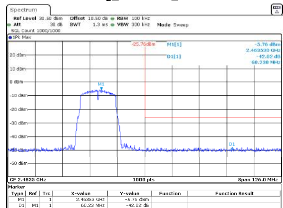
802.11g_2462MHz_Chain 0
