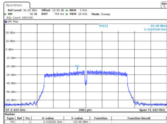
802.11n40_2422MHz_Chain 1
