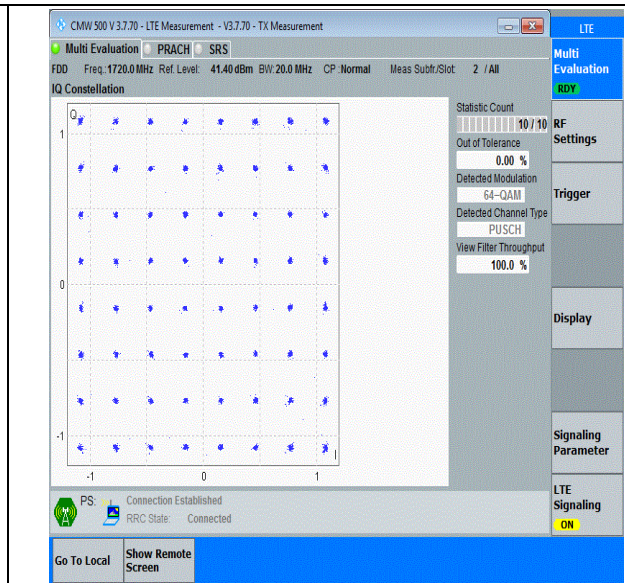
Band66-20MHz-64QAM-132072-100RB#0-PASS
