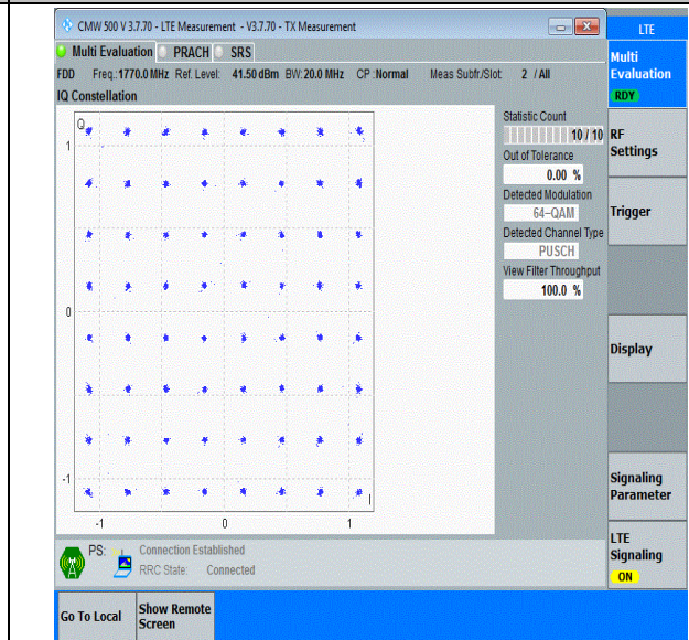
Band66-20MHz-64QAM-132572-100RB#0-PASS
