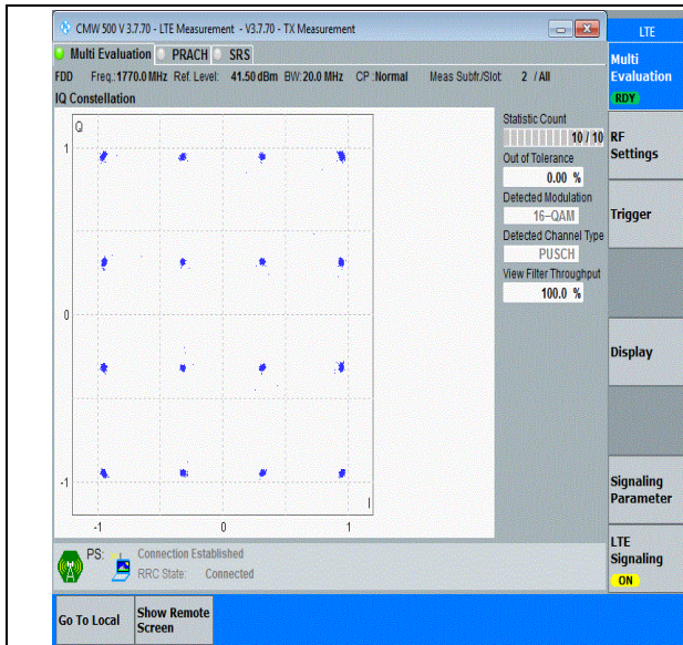
Band66-20MHz-16QAM-132572-100RB#0-PASS
