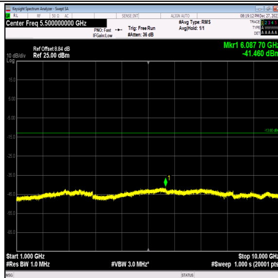
Band5-4233-4-1000~10000MHz-PASS
