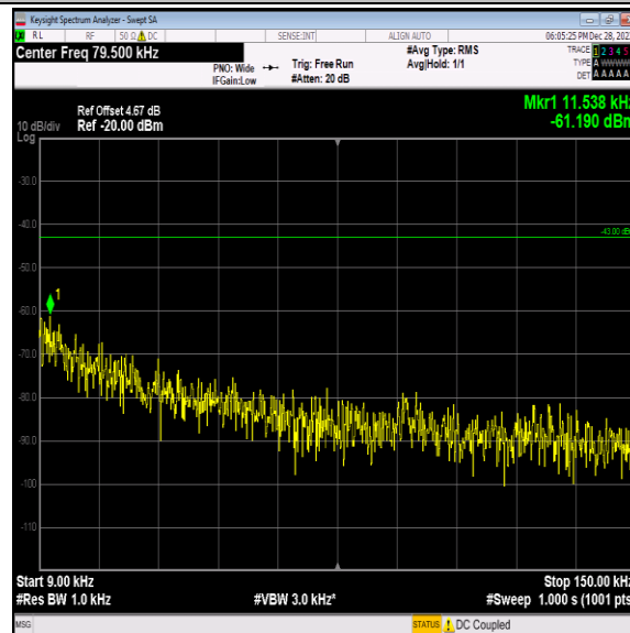
Band2-9262-5-0.009~0.15MHz-PASS
