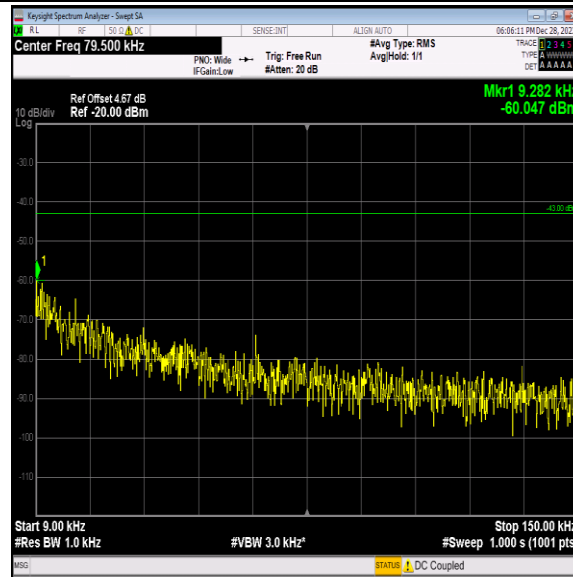
Band2-9400-5-0.009~0.15MHz-PASS
