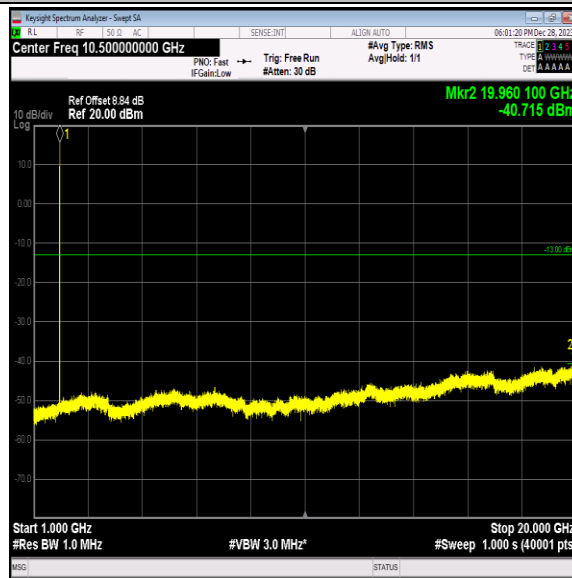
Band2-9538-3-1000~20000MHz-PASS
