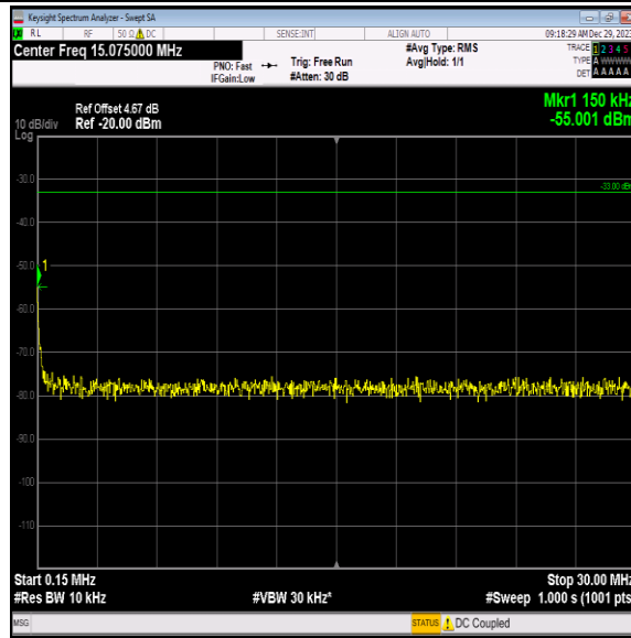
Band4-1312-3-0.15~30MHz-PASS
