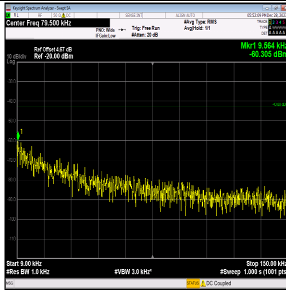
Band2-9400-1-0.009~0.15MHz-PASS
