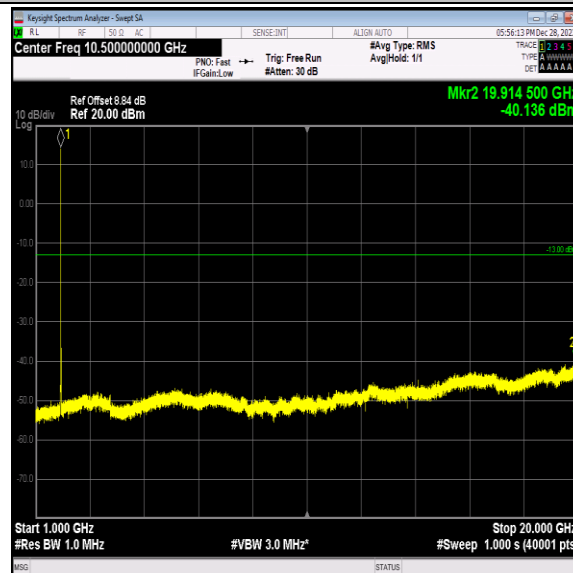
Band2-9400-2-1000~20000MHz-PASS
