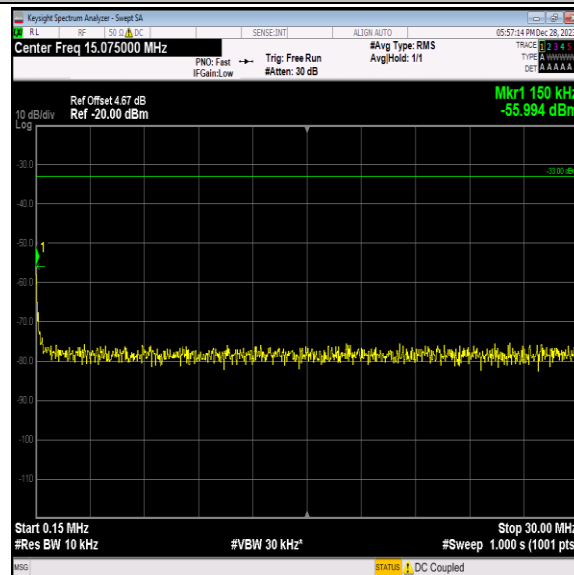
Band2-9538-2-0.15~30MHz-PASS
