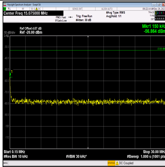
Band4-1312-4-0.15~30MHz-PASS
