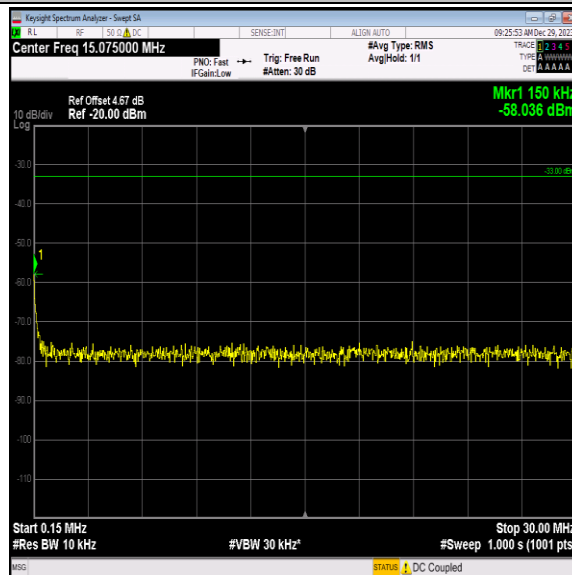
Band4-1312-5-0.15~30MHz-PASS
