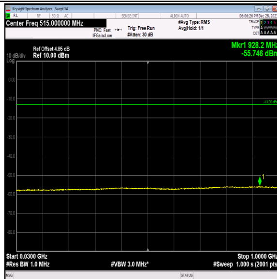
Band2-9400-5-30~1000MHz-PASS
