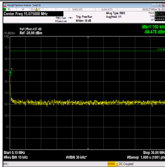
Band2-9538-1-0.15~30MHz-PASS
