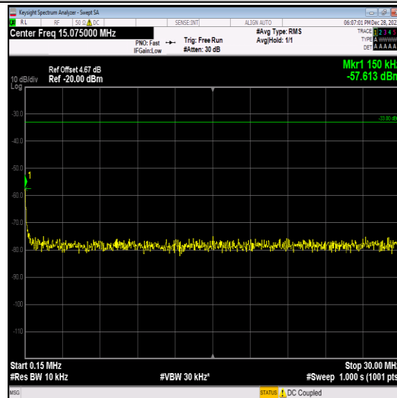
Band2-9538-5-0.15~30MHz-PASS
