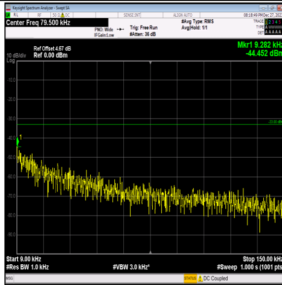
Band5-4233-4-0.009~0.15MHz-PASS
