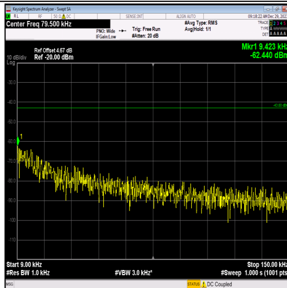
Band4-1312-3-0.009~0.15MHz-PASS
