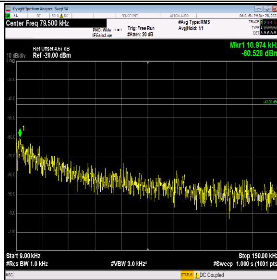
Band2-9262-4-0.009~0.15MHz-PASS
