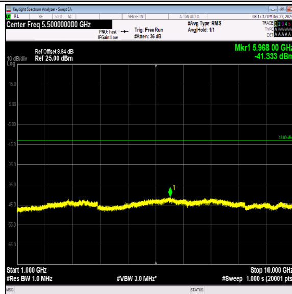
Band5-4233-3-1000~10000MHz-PASS
