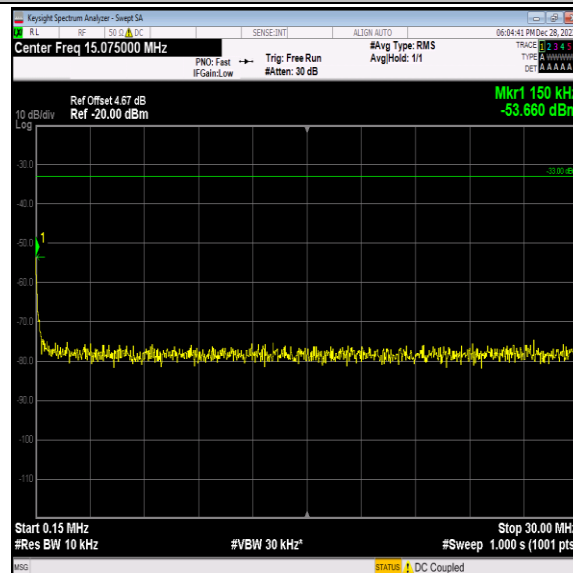
Band2-9538-4-0.15~30MHz-PASS
