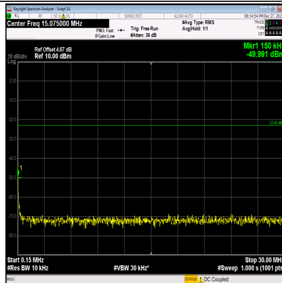
Band5-4233-2-0.15~30MHz-PASS
