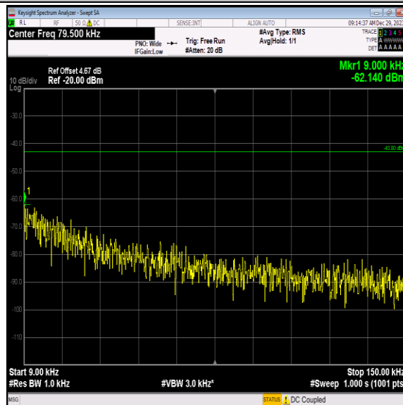
Band4-1312-2-0.009~0.15MHz-PASS
