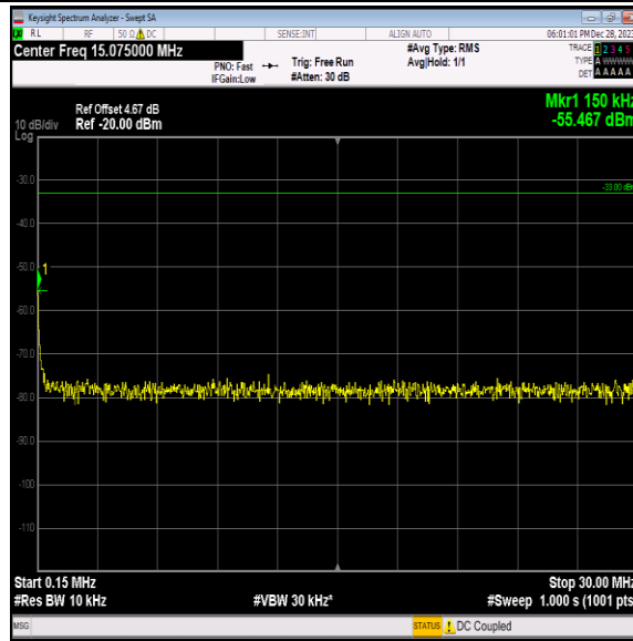
Band2-9538-3-0.15~30MHz-PASS
