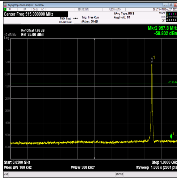
Band5-4233-3-30~1000MHz-PASS
