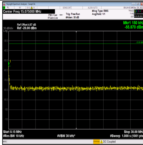
Band4-1312-2-0.15~30MHz-PASS
