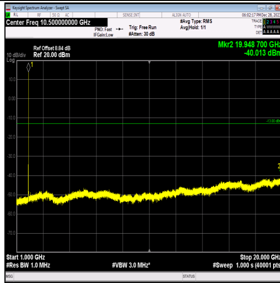
Band2-9262-4-1000~20000MHz-PASS
