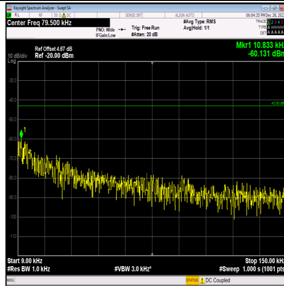
Band2-9538-4-0.009~0.15MHz-PASS
