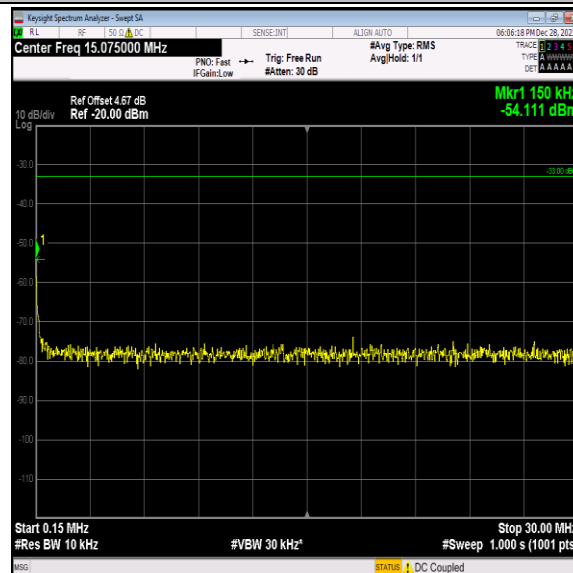
Band2-9400-5-0.15~30MHz-PASS
