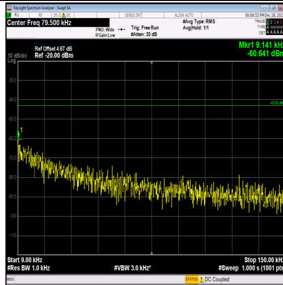
Band2-9538-5-0.009~0.15MHz-PASS
