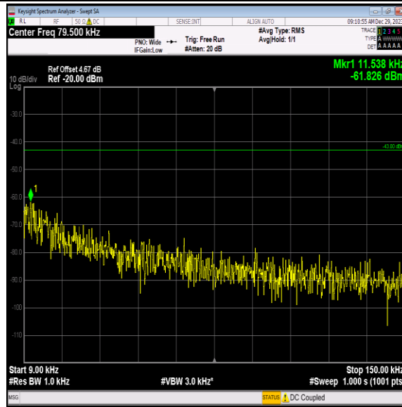
Band4-1312-1-0.009~0.15MHz-PASS
