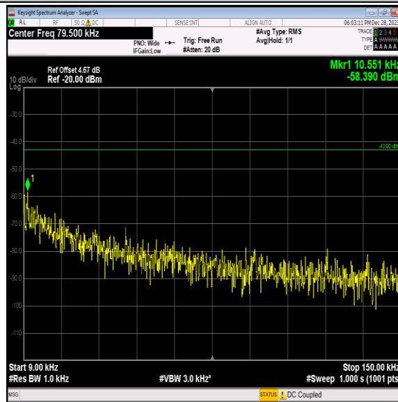
Band2-9400-4-0.009~0.15MHz-PASS
