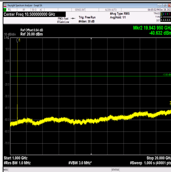
Band2-9262-5-1000~20000MHz-PASS
