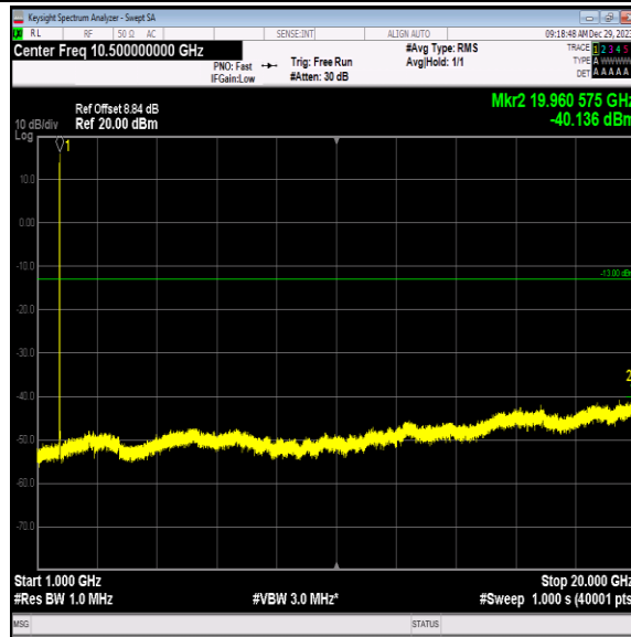
Band4-1312-3-1000~20000MHz-PASS
