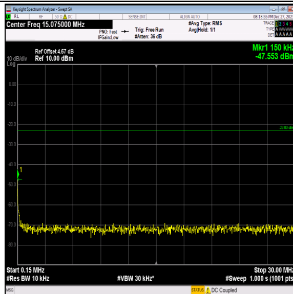
Band5-4233-4-0.15~30MHz-PASS
