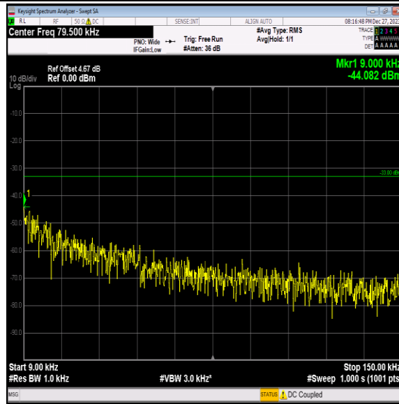
Band5-4233-3-0.009~0.15MHz-PASS
