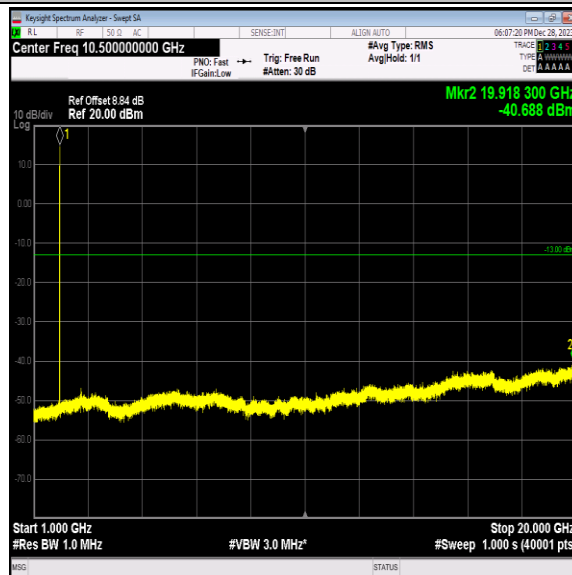
Band2-9538-5-1000~20000MHz-PASS
