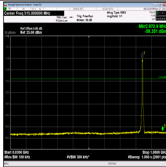
Band5-4233-2-30~1000MHz-PASS
