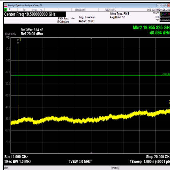
Band2-9400-1-1000~20000MHz-PASS
