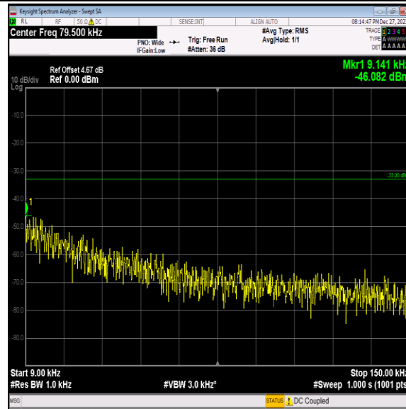
Band5-4233-2-0.009~0.15MHz-PASS
