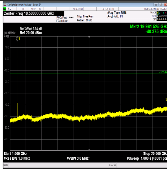
Band2-9400-5-1000~20000MHz-PASS
