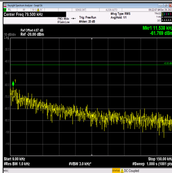
Band4-1312-4-0.009~0.15MHz-PASS
