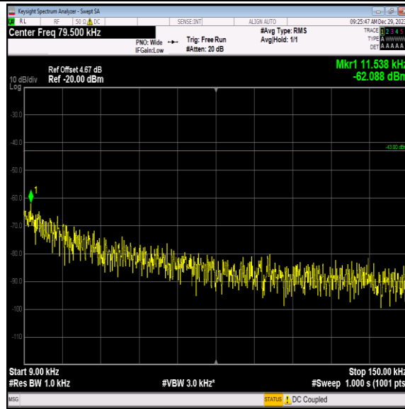
Band4-1312-5-0.009~0.15MHz-PASS
