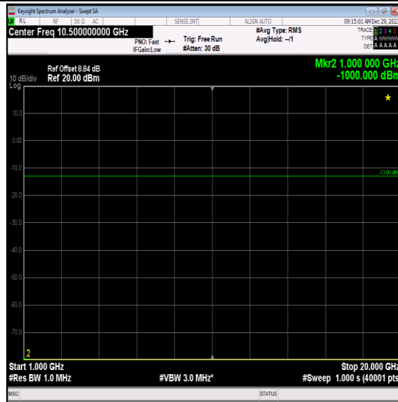
Band4-1312-2-1000~20000MHz-PASS
