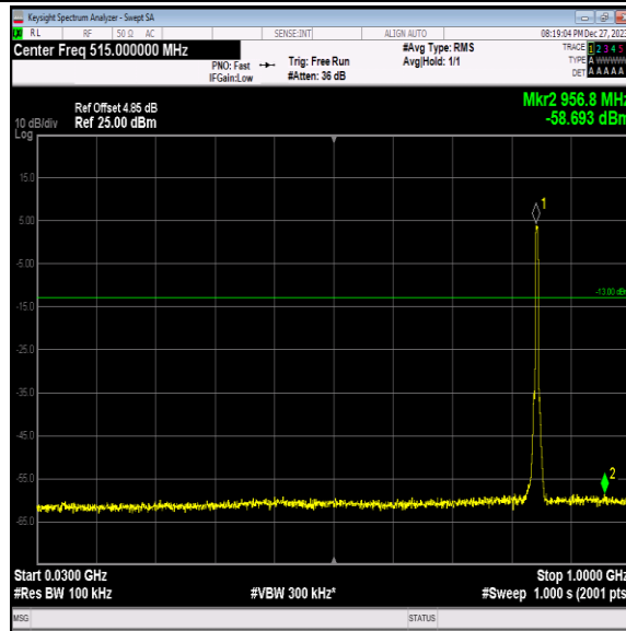
Band5-4233-4-30~1000MHz-PASS
