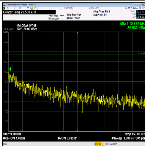
Band2-9538-3-0.009~0.15MHz-PASS
