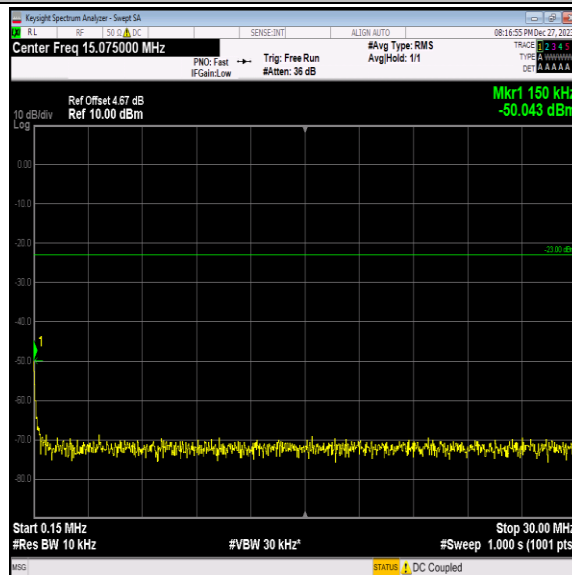
Band5-4233-3-0.15~30MHz-PASS
