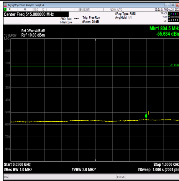
Band2-9262-1-30~1000MHz-PASS
