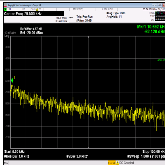
Band2-9262-2-0.009~0.15MHz-PASS
