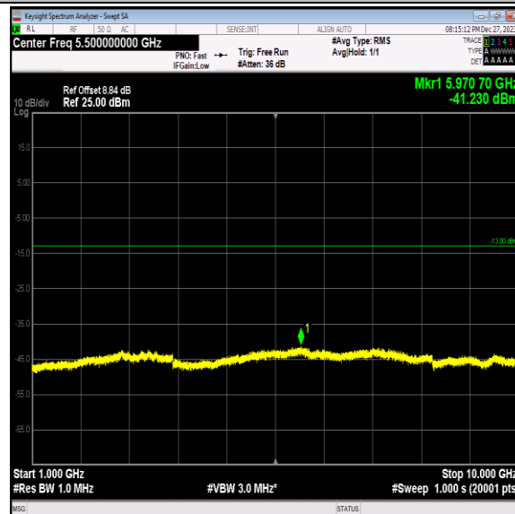
Band5-4233-2-1000~10000MHz-PASS
