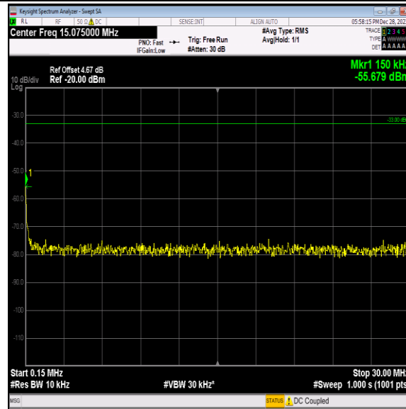
Band2-9262-3-0.15~30MHz-PASS
