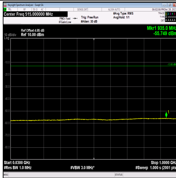
Band2-9262-4-30~1000MHz-PASS
