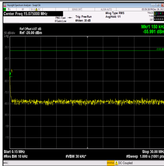
Band2-9400-3-0.15~30MHz-PASS
