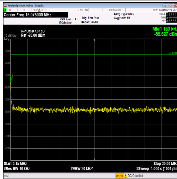
Band4-1312-1-0.15~30MHz-PASS
