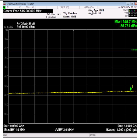
Band2-9538-4-30~1000MHz-PASS
