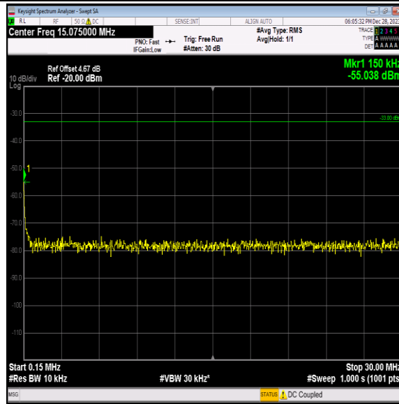
Band2-9262-5-0.15~30MHz-PASS
