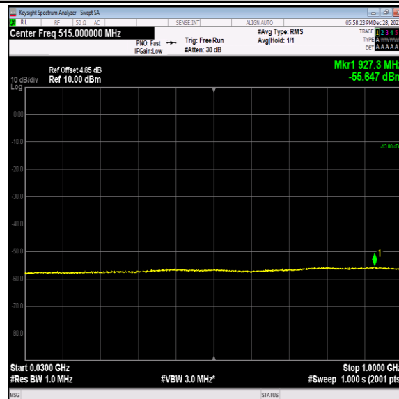
Band2-9262-3-30~1000MHz-PASS
