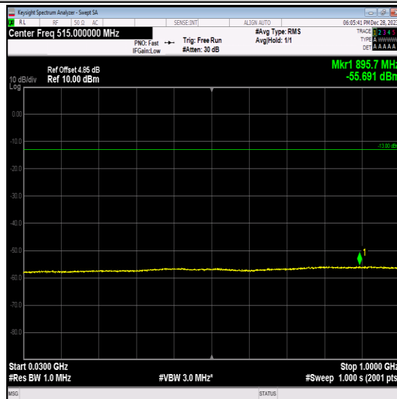
Band2-9262-5-30~1000MHz-PASS
