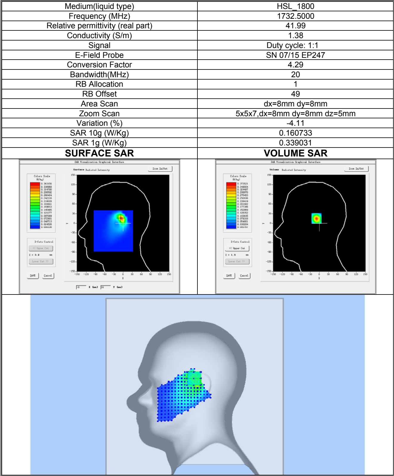
Plot 16:LTE BAND 4, Middle channel (Right Head Tilt) Product Description:Mobile Phone Test Date: 2019-12-24
