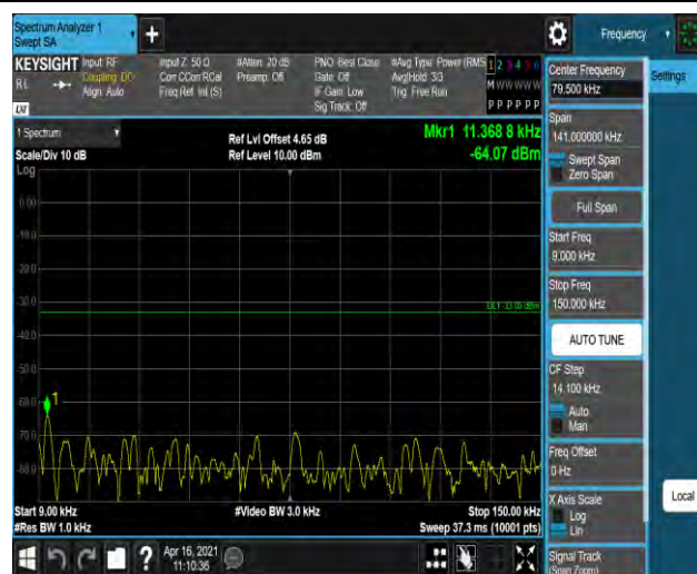
EGPRS850-128-8-0.009~0.15MHz
