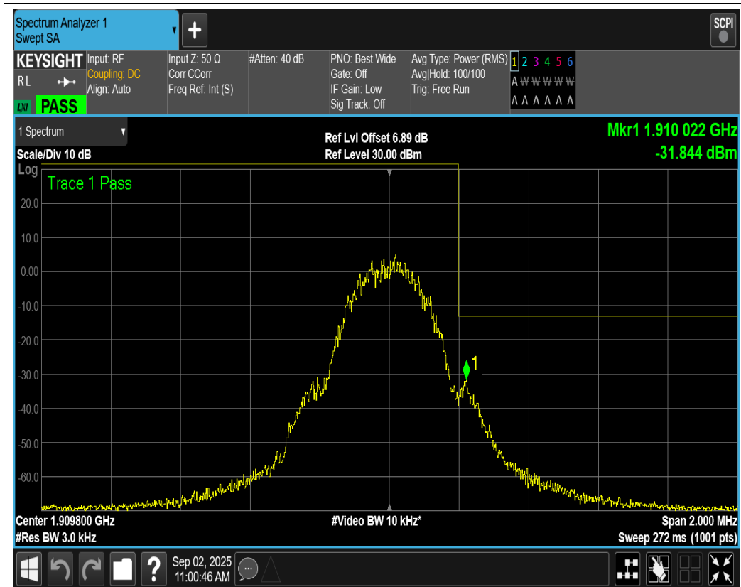
GSM1900 Channel=810
