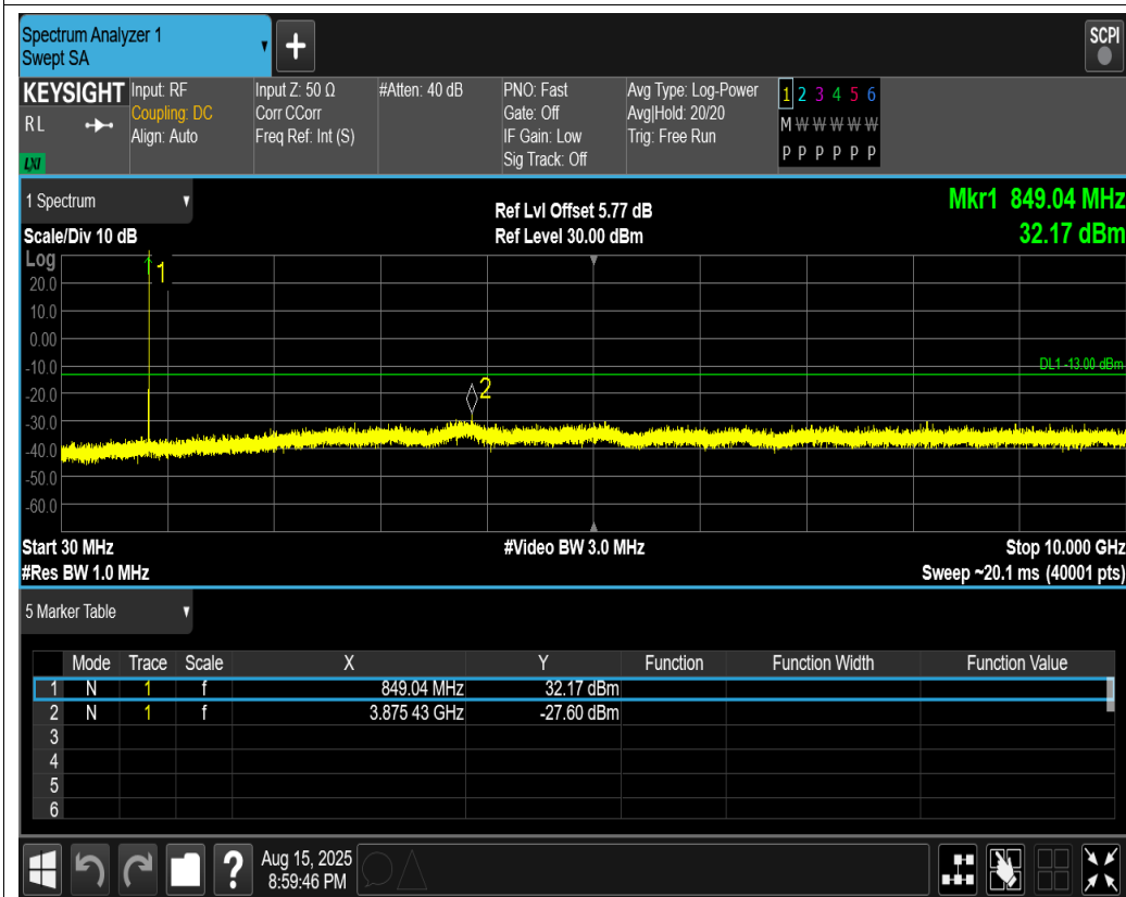
GPRS850 Channel=251
