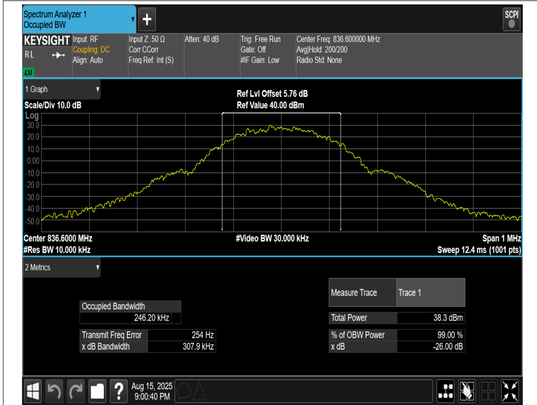
EGPRS850 Channel=190
