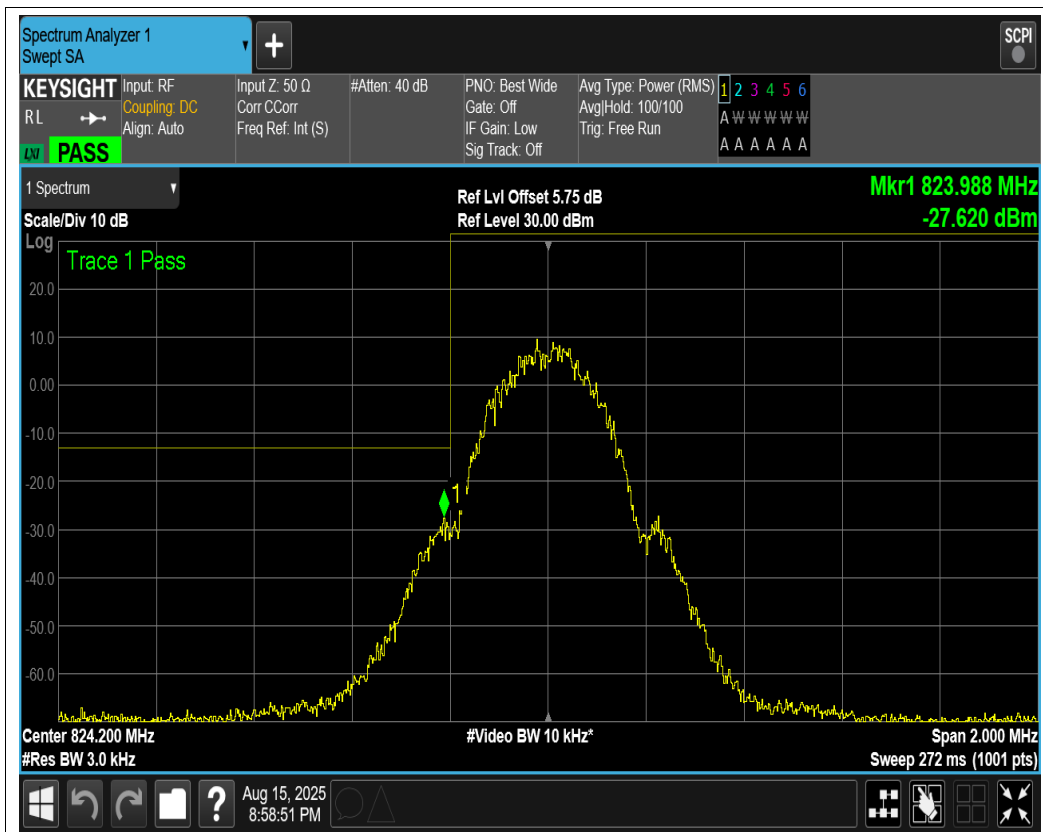
GPRS850 Channel=128
