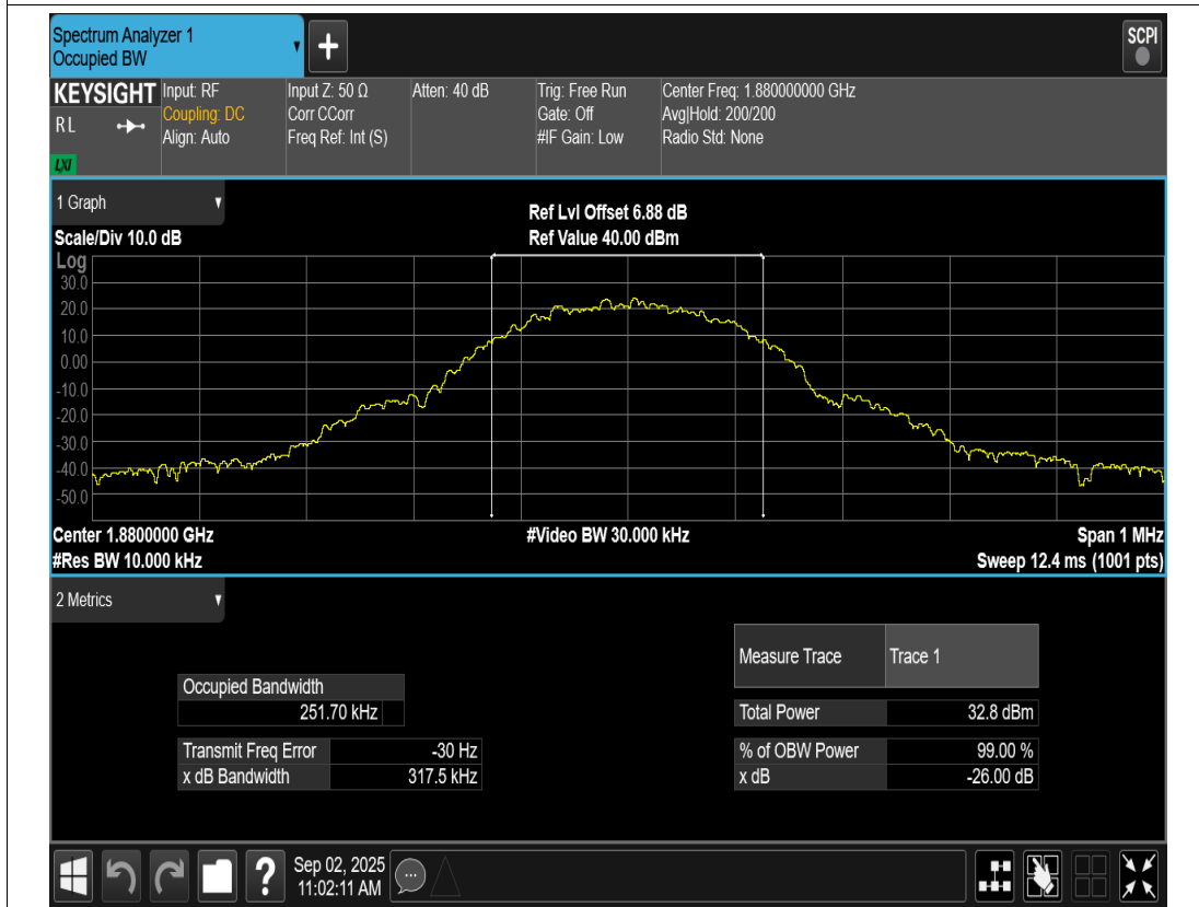
GPRS1900 Channel=661
