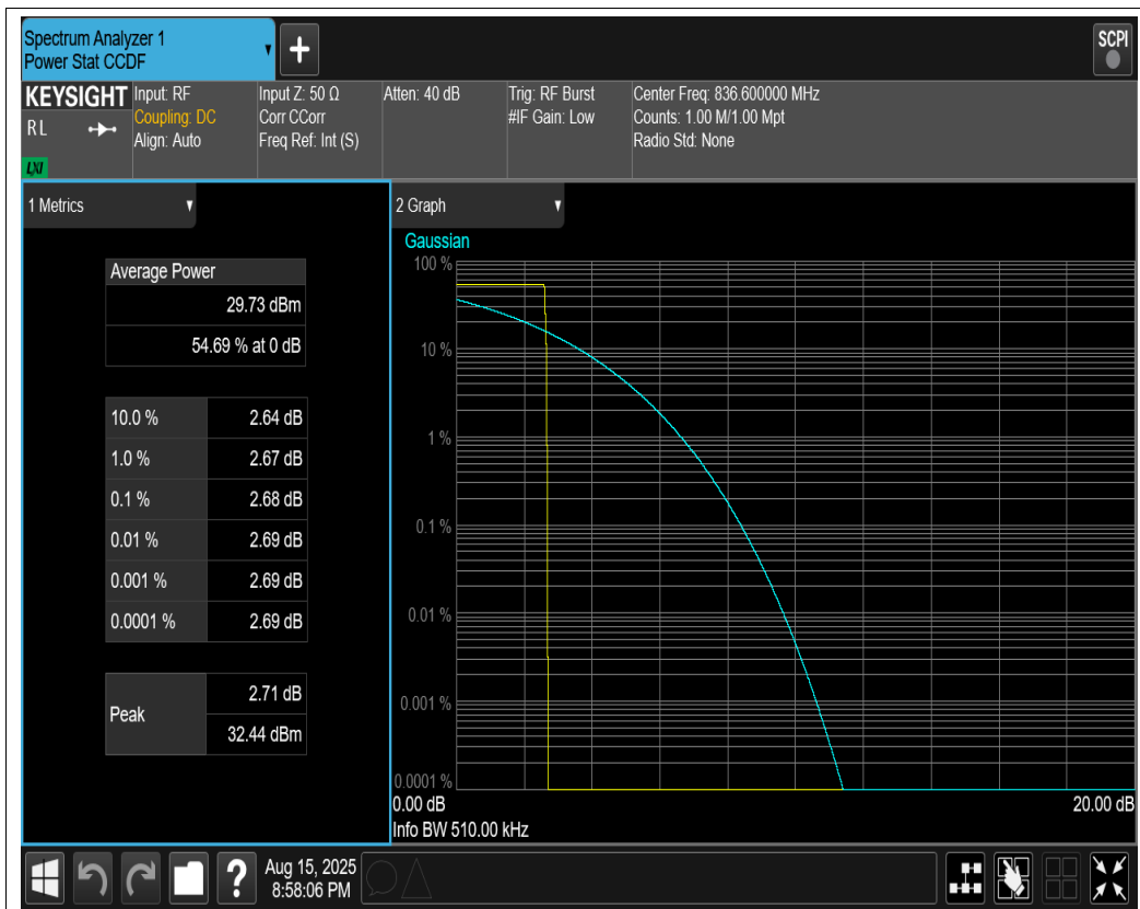
GPRS850 Channel=190
