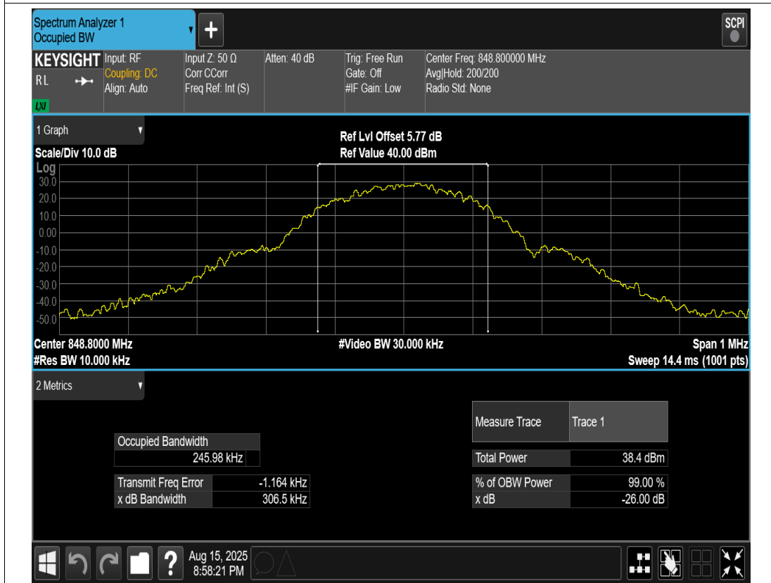
GPRS850 Channel=251
