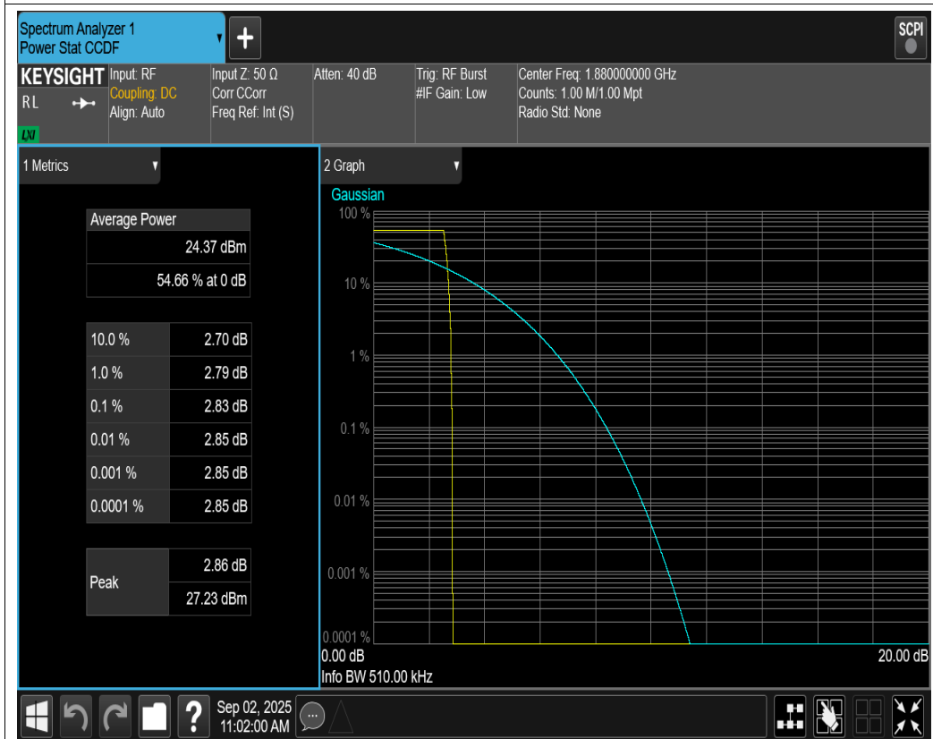
GPRS1900 Channel=661
