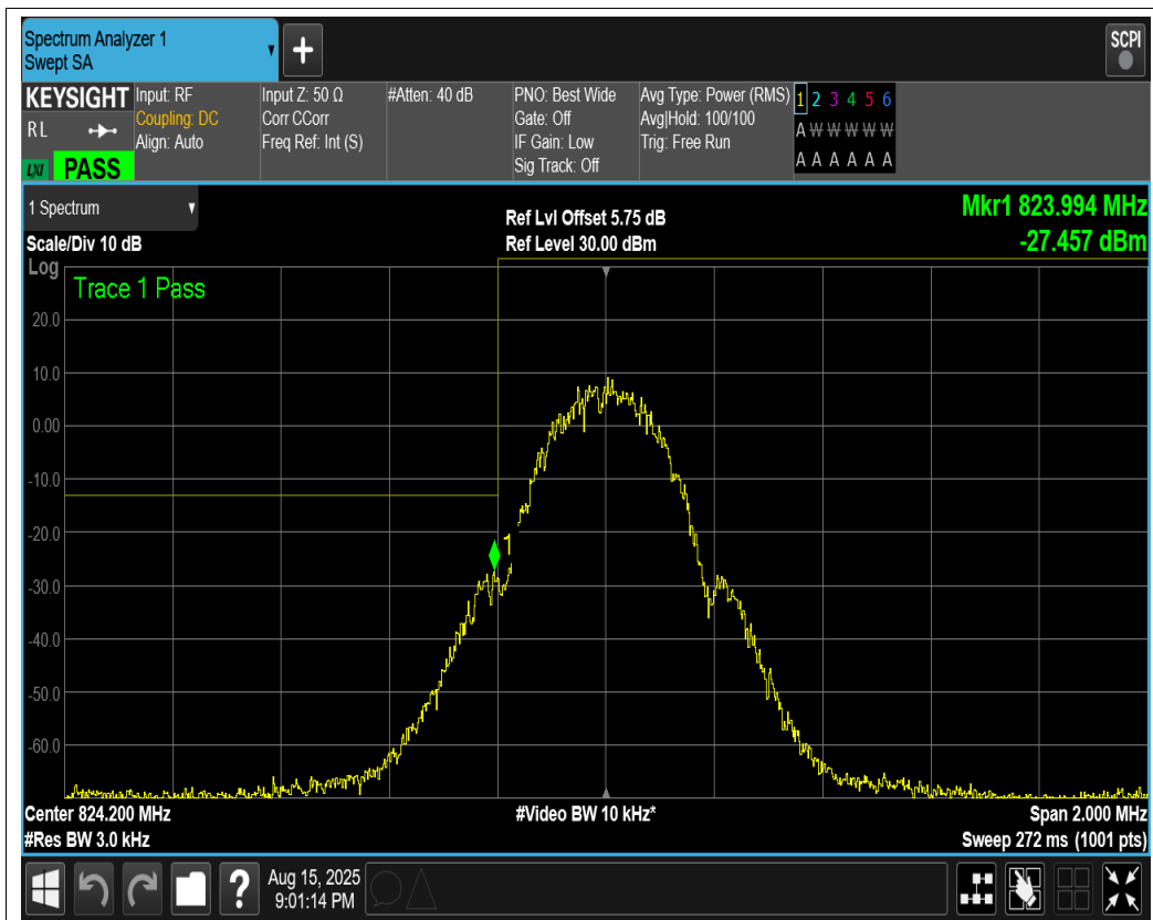
EGPRS850 Channel=128
