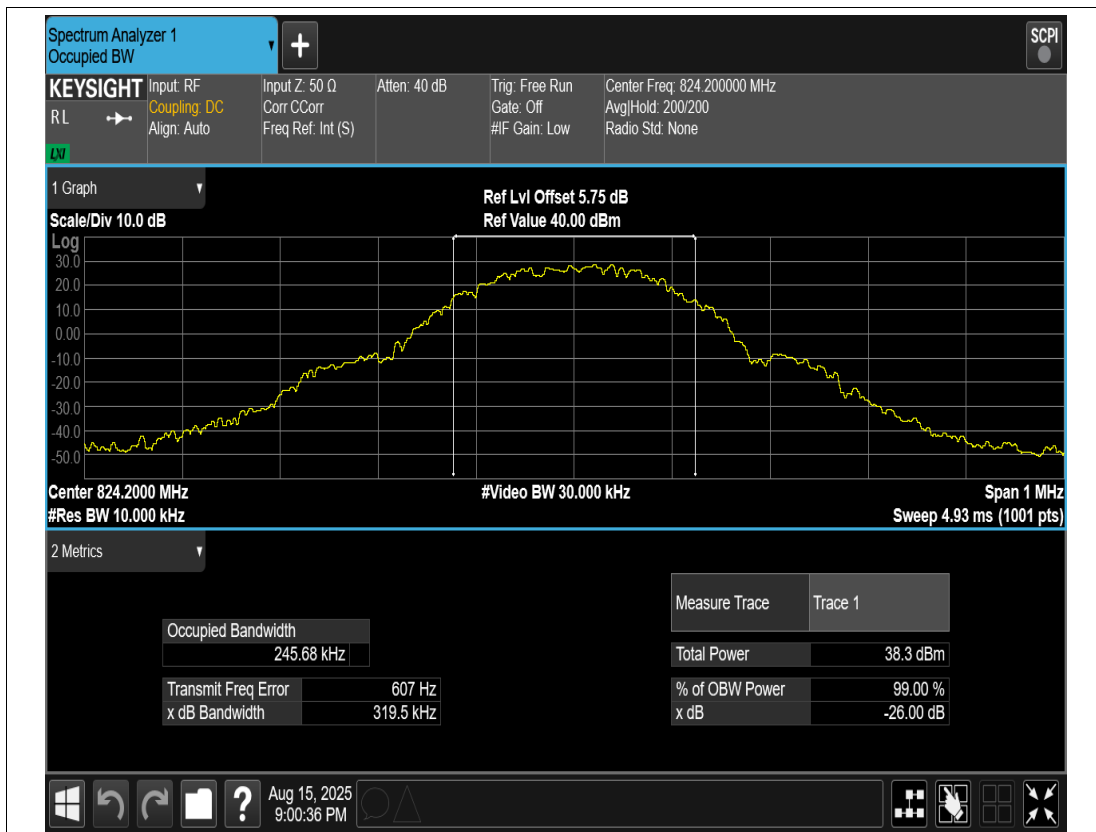
EGPRS850 Channel=128
