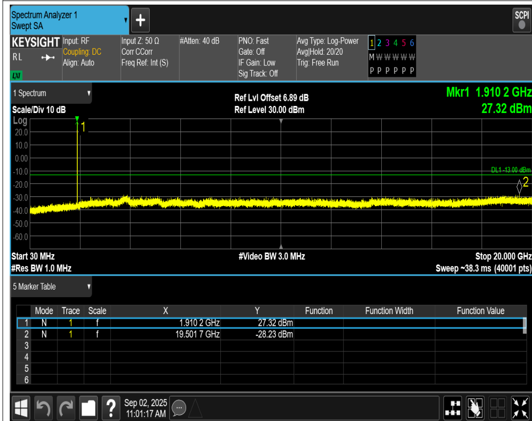
GSM1900 Channel=810
