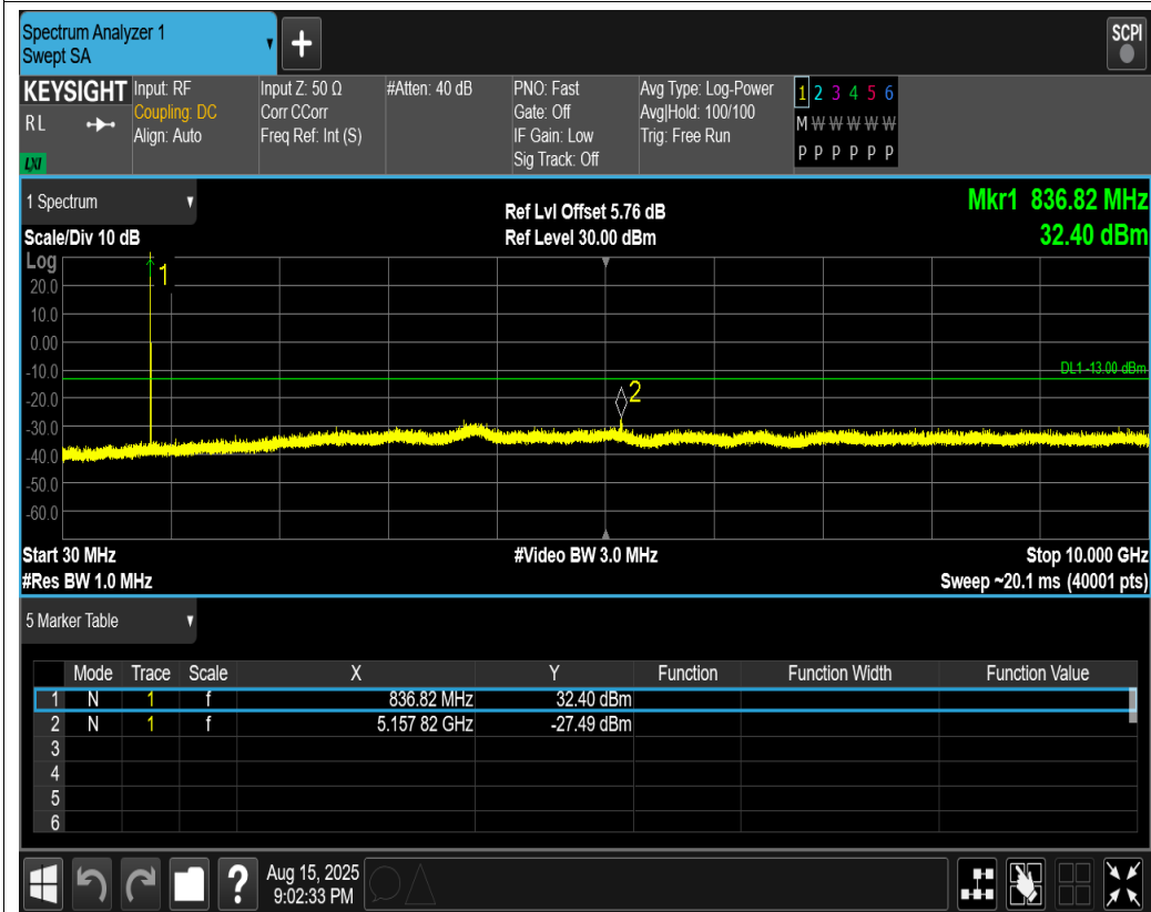
EGPRS850 Channel=190
