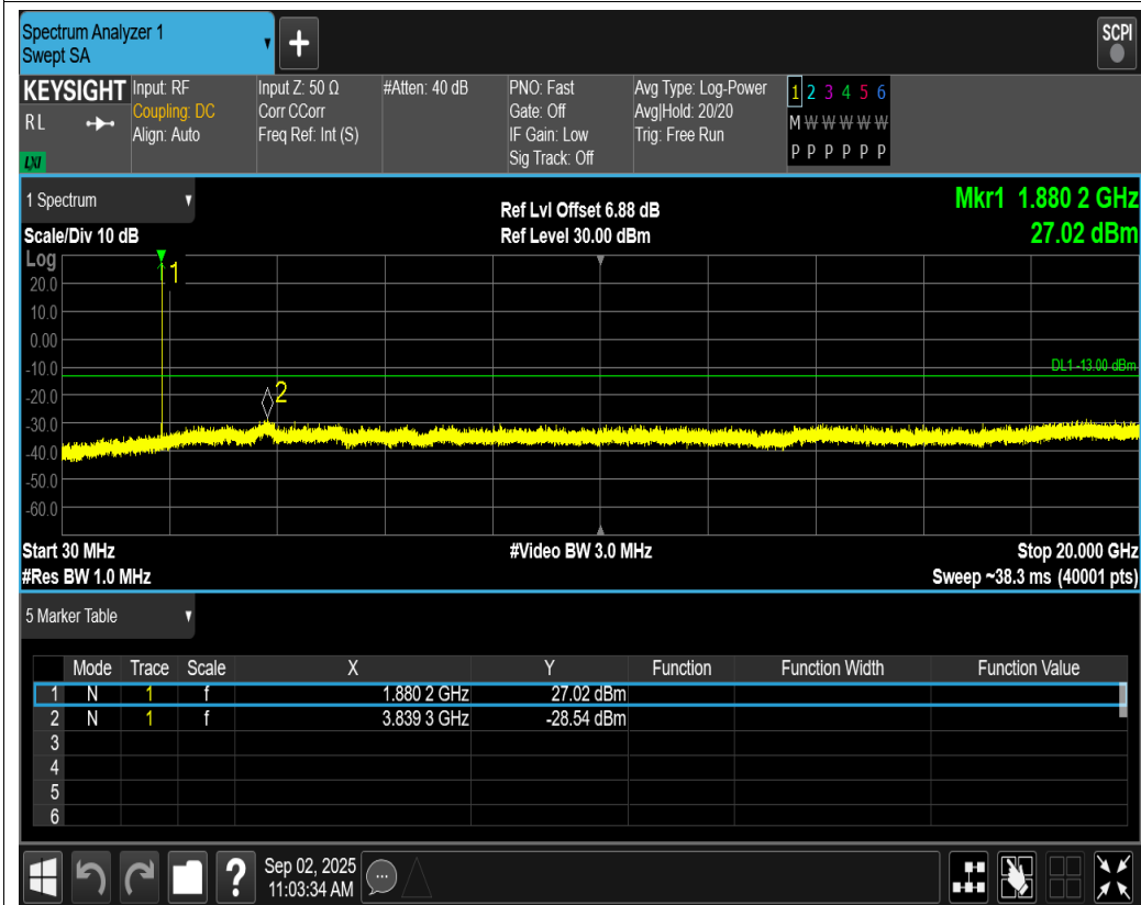
GPRS1900 Channel=661
