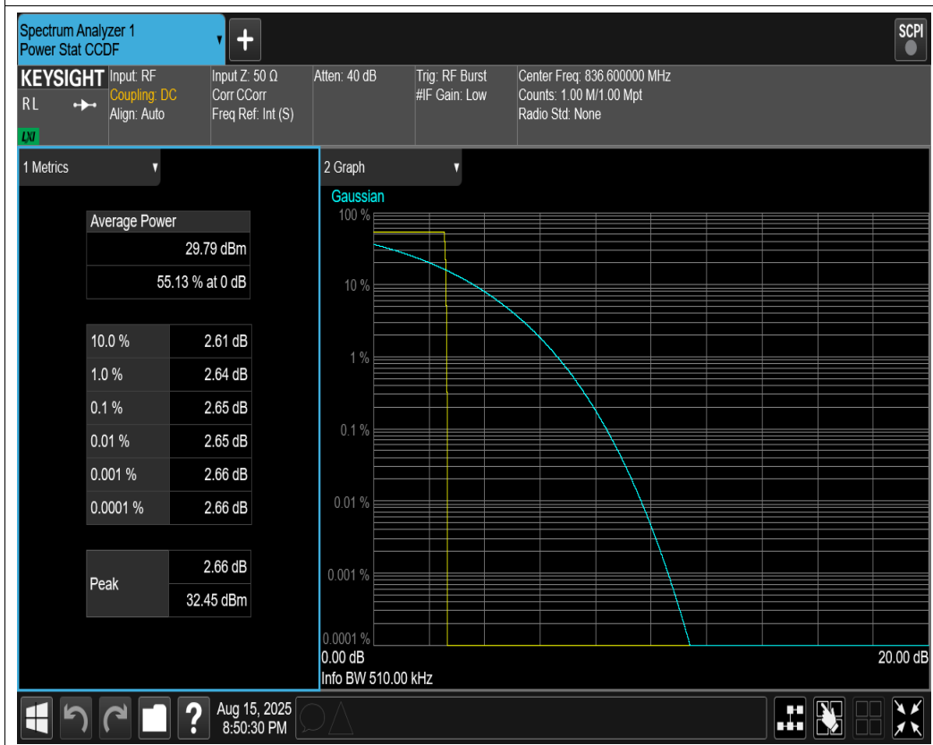
GSM850 Channel=190
