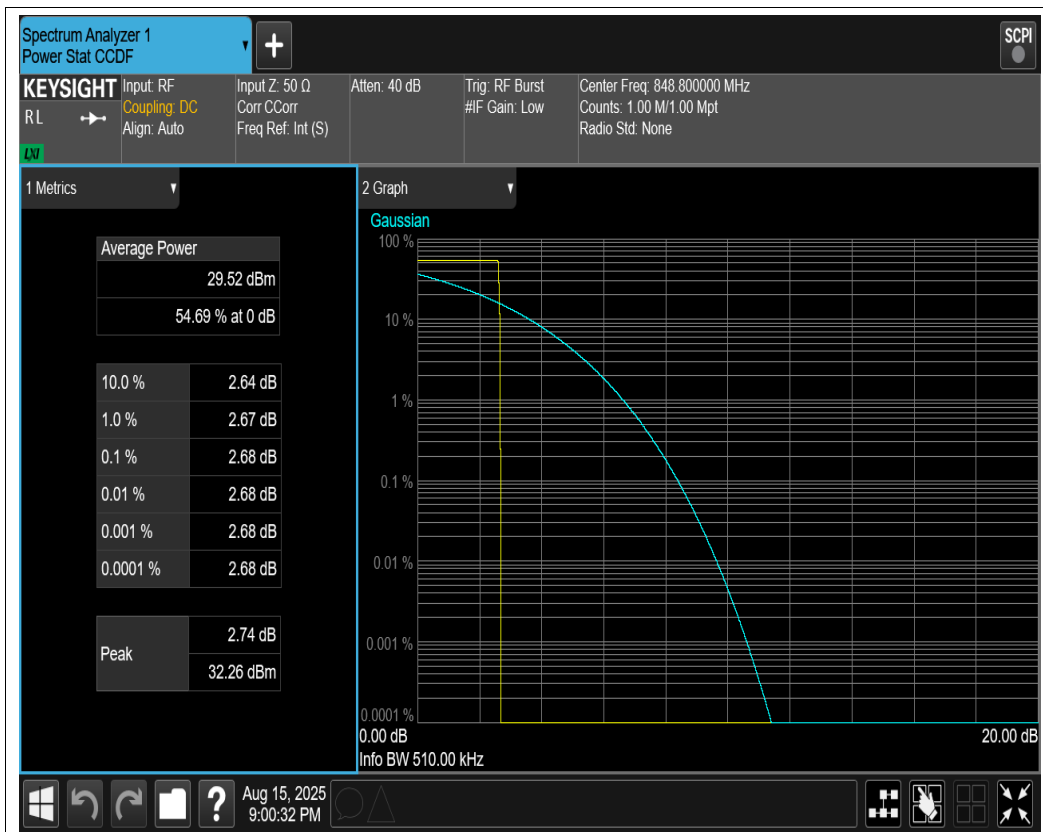
EGPRS850 Channel=251
