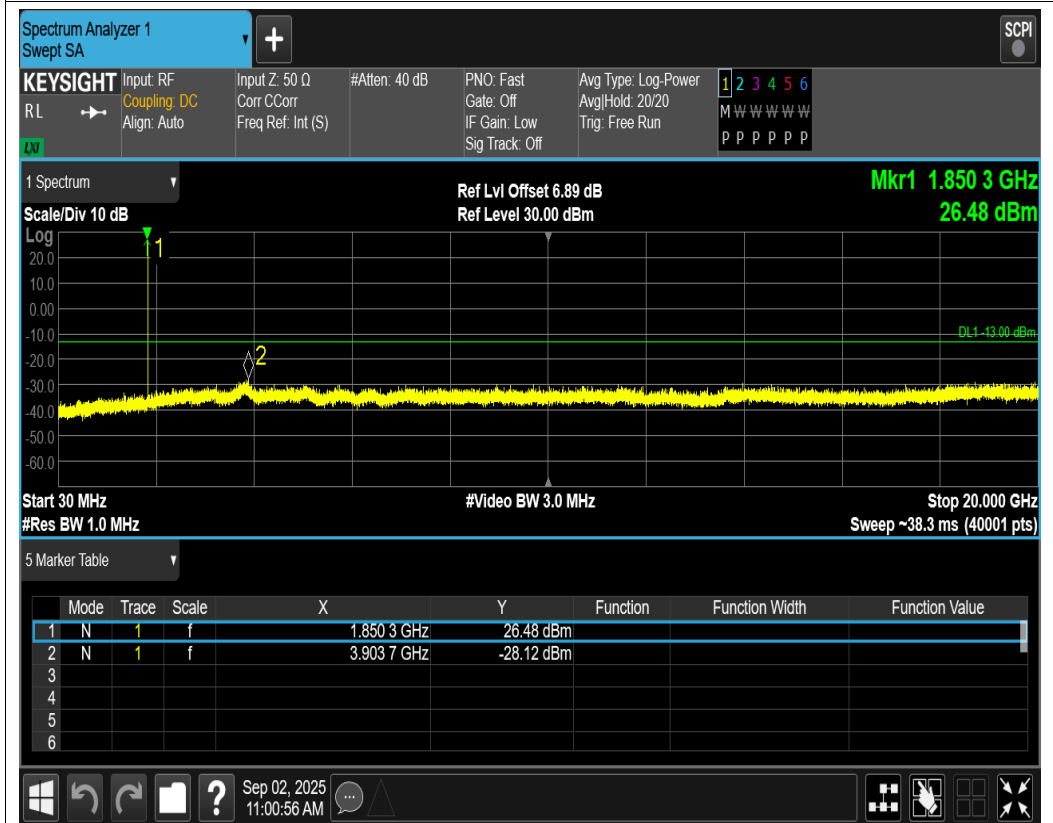
GSM1900 Channel=512
