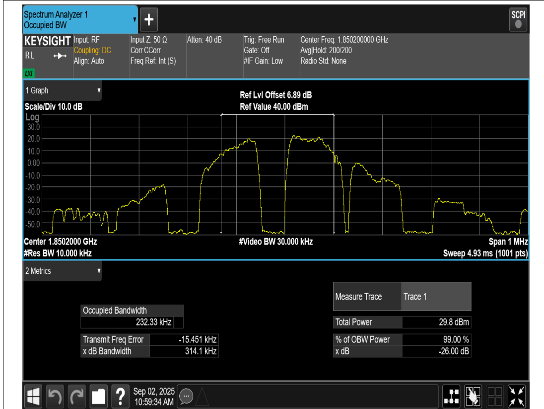
GSM1900 Channel=512
