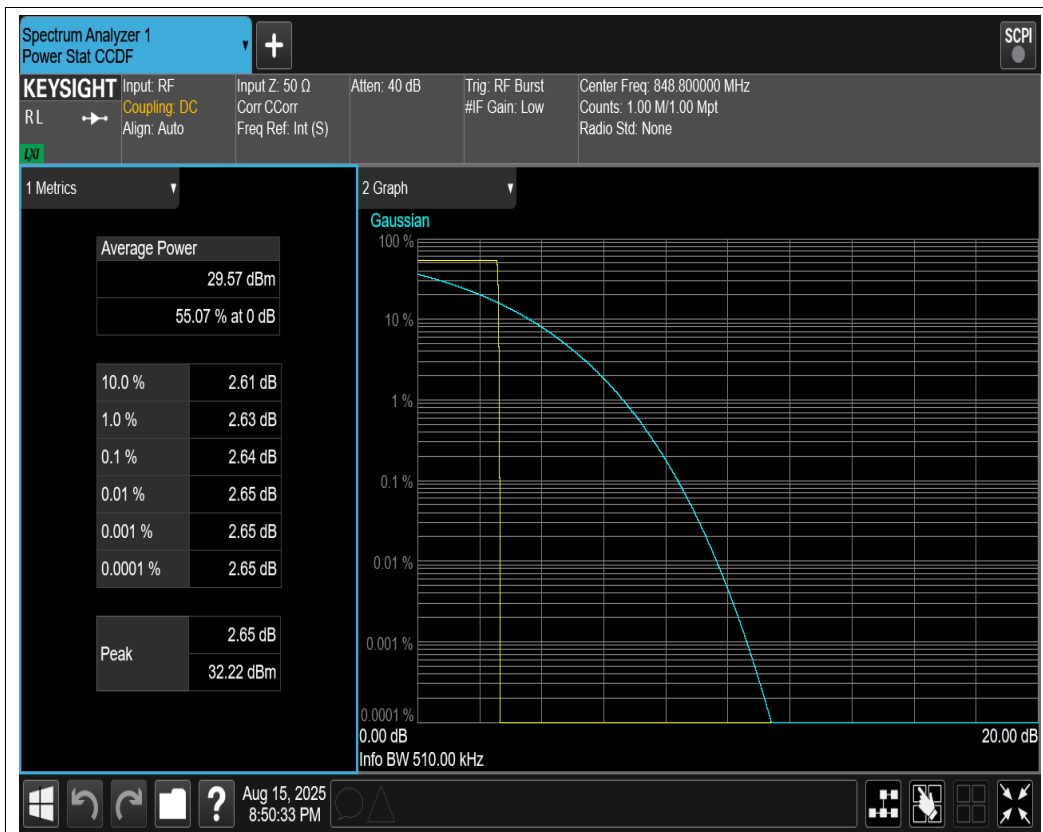
GSM850 Channel=251
