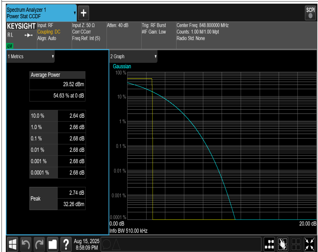
GPRS850 Channel=251
