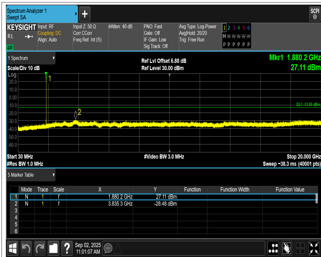
GSM1900 Channel=661
