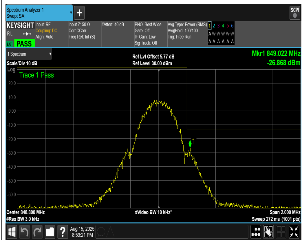
GPRS850 Channel=251
