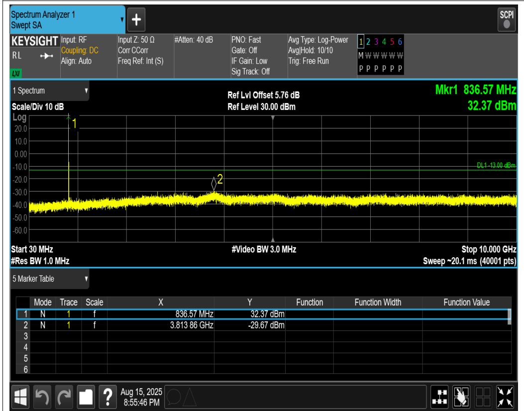
GSM850 Channel=190
