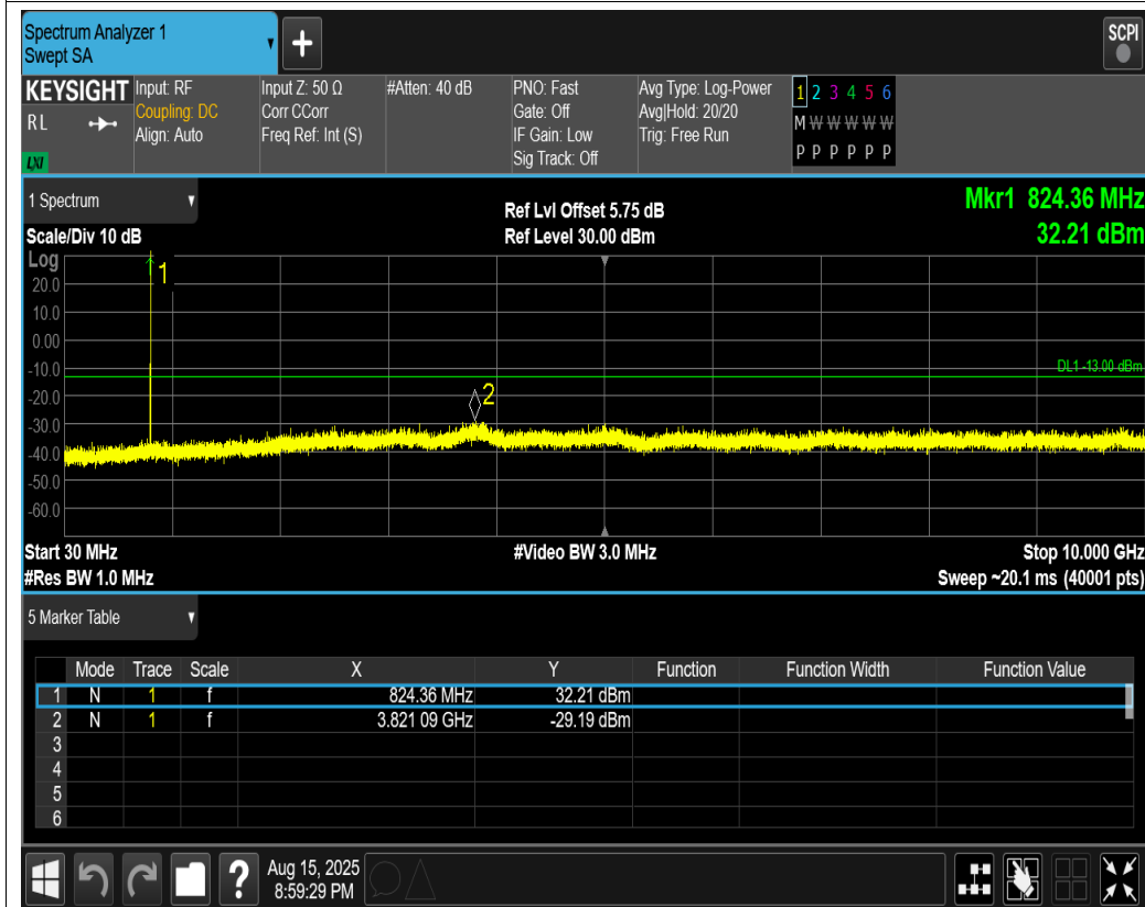
GPRS850 Channel=128
