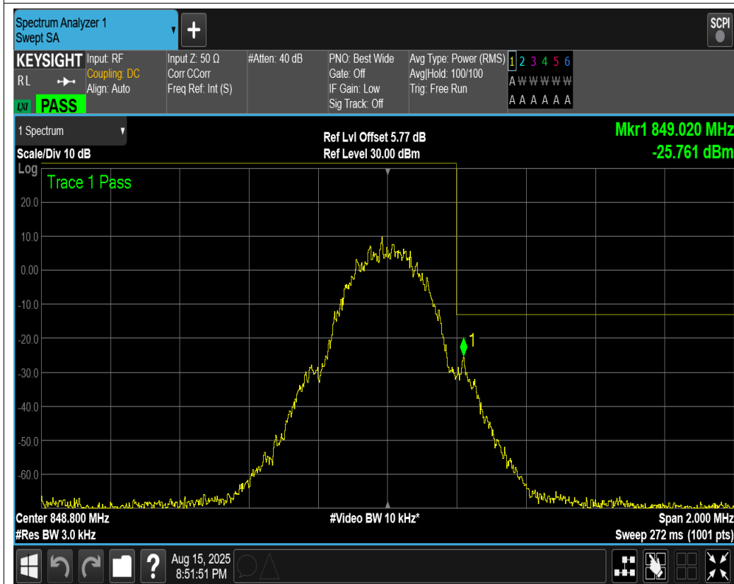
GSM850 Channel=251
