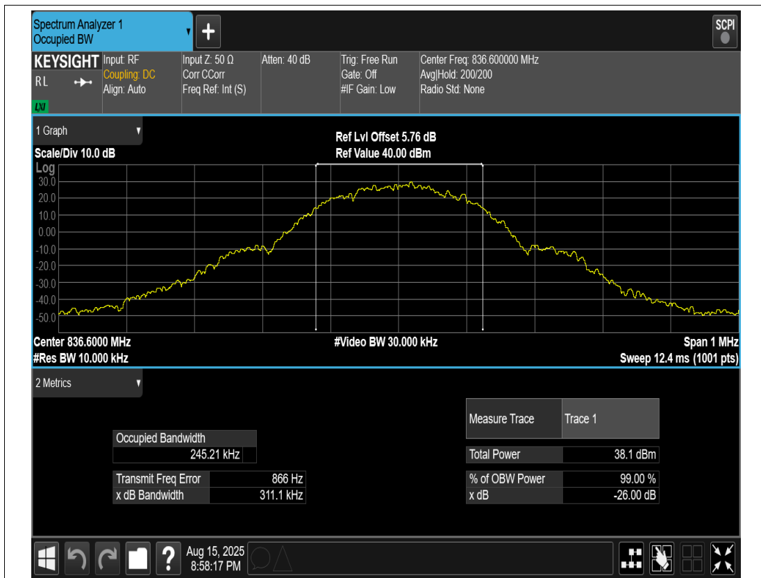
GPRS850 Channel=190
