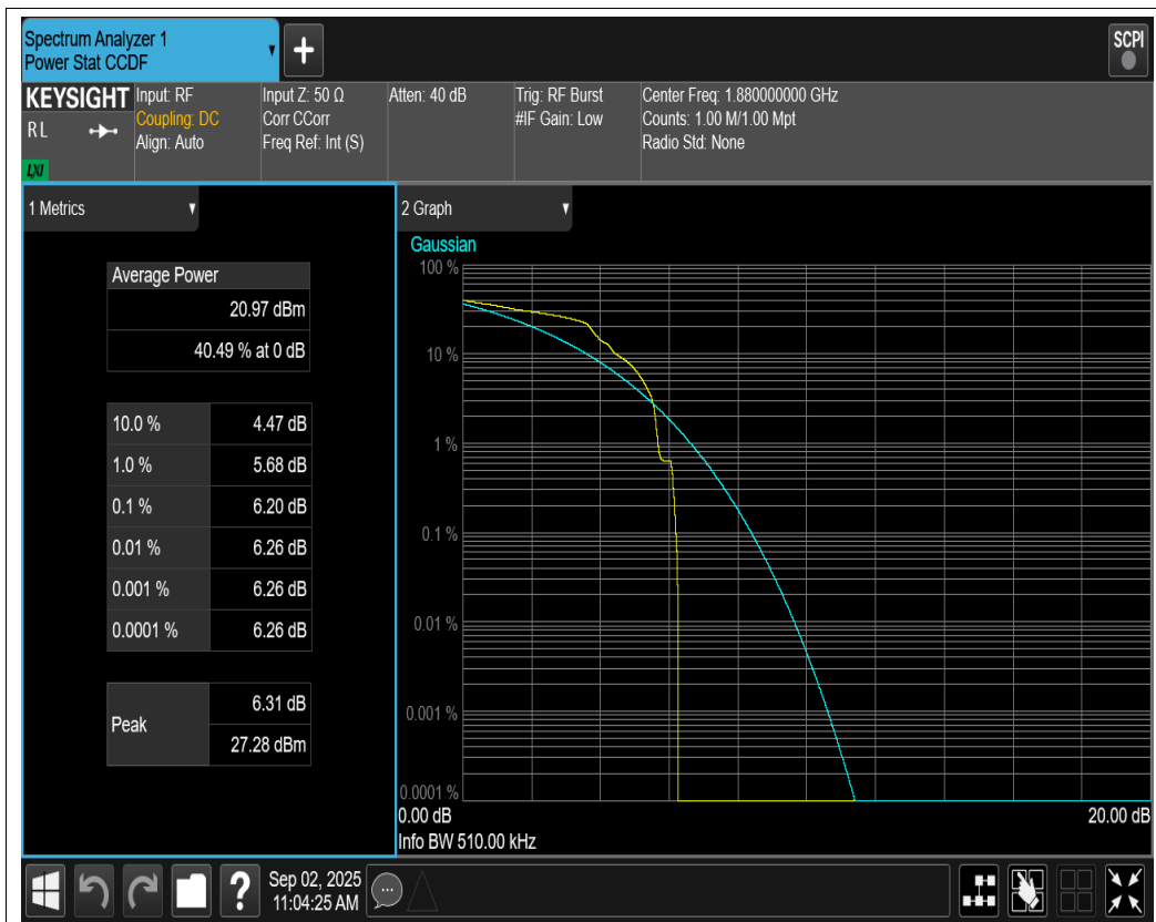
EGPRS1900 Channel=661
