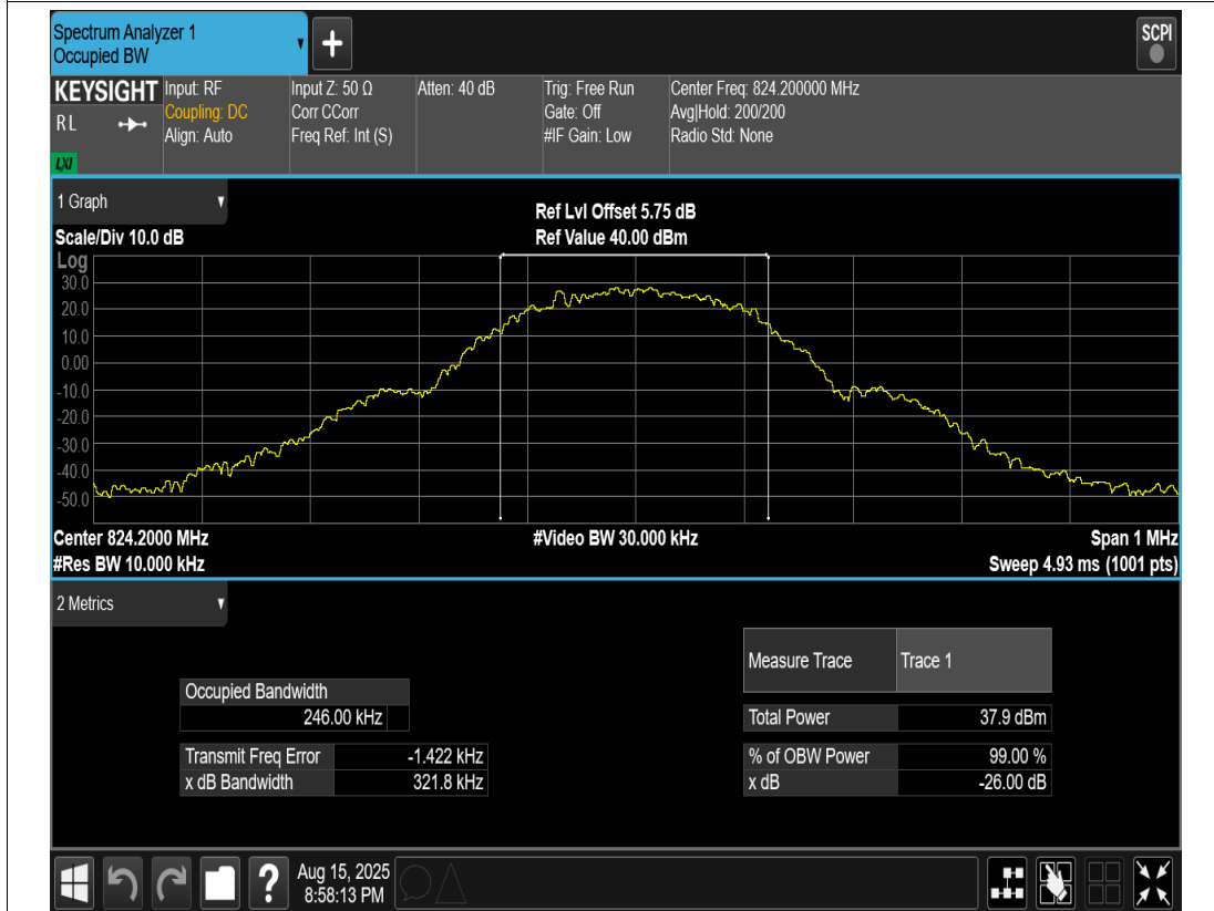
GPRS850 Channel=128
