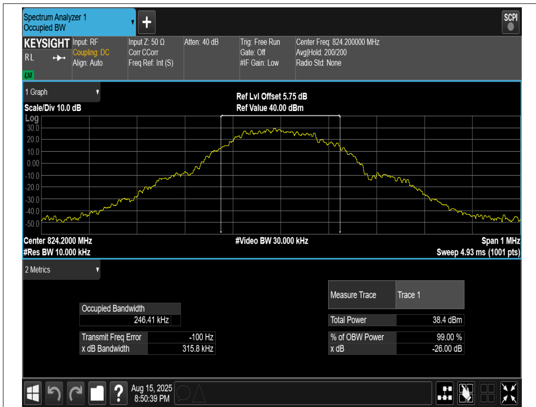
GSM850 Channel=128
