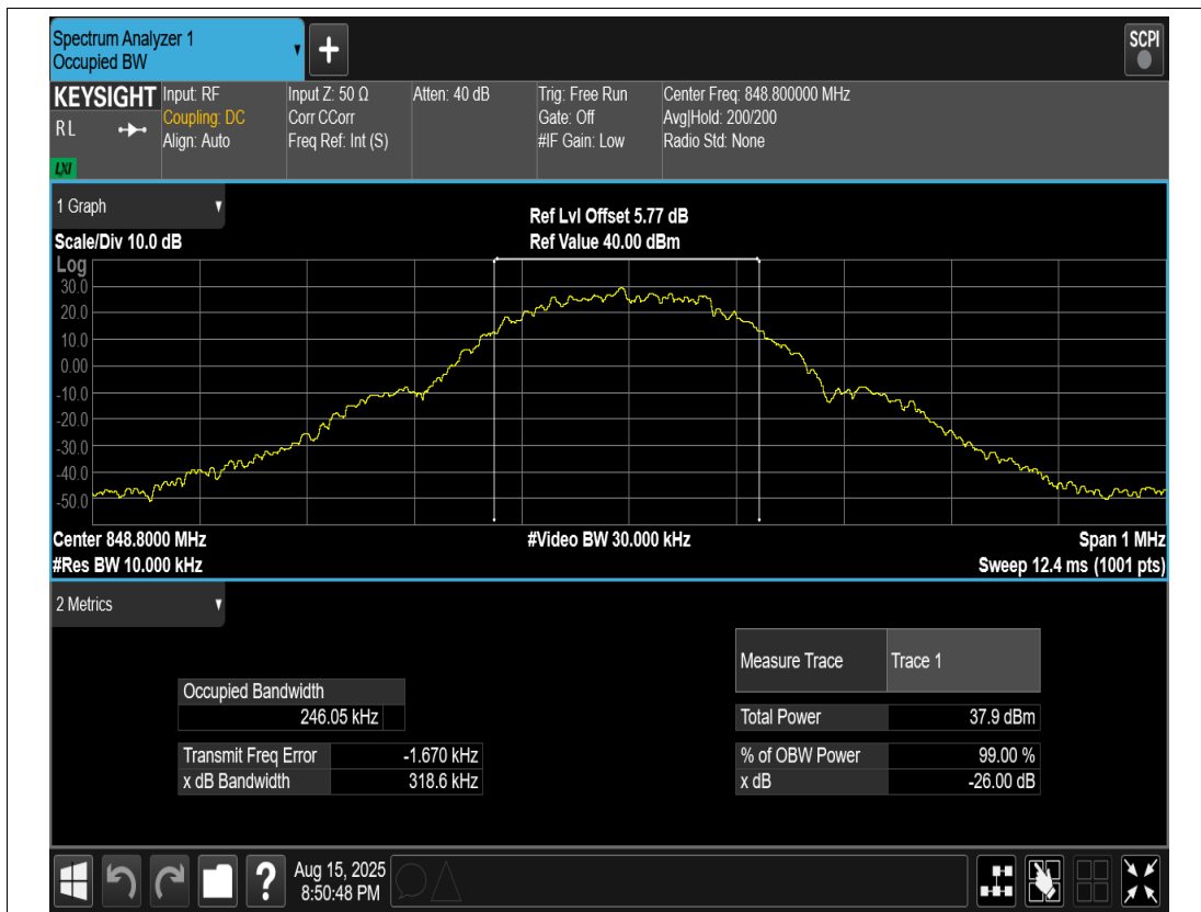
GSM850 Channel=251
