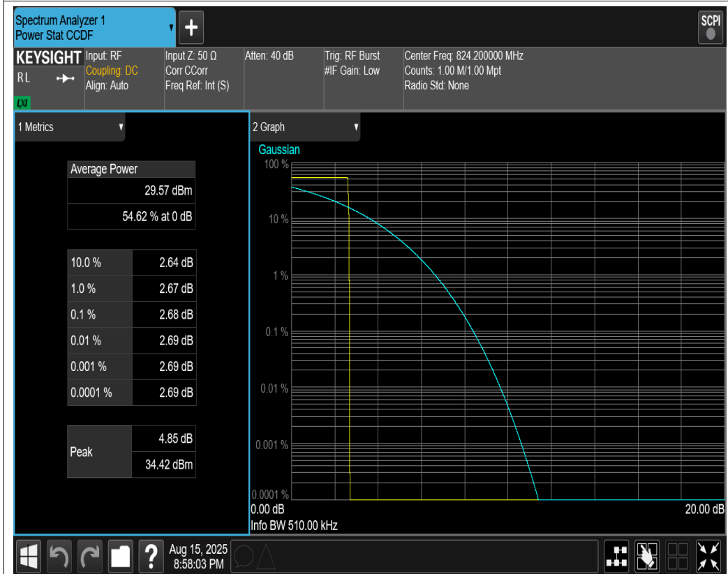
GPRS850 Channel=128
