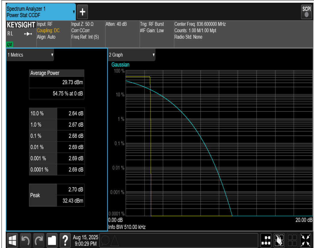
EGPRS850 Channel=190
