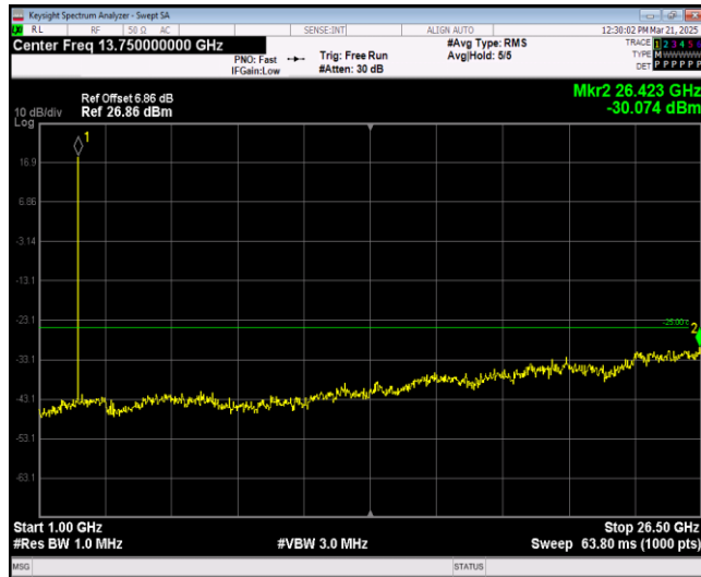
Band7-5MHz-64QAM-21100-1RB#0-Range2:1000~2 6500MHz
