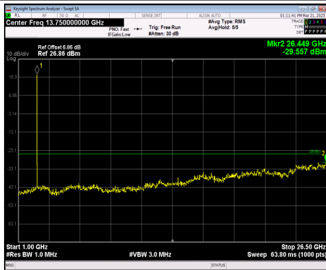
Band7-20MHz-16QAM-20850-1RB#0-Range2:1000~ 26500MHz
