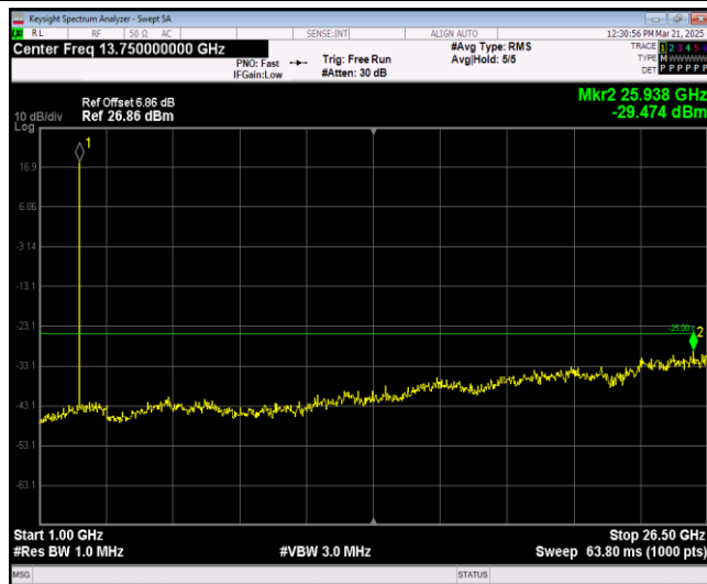
Band7-5MHz-64QAM-21425-1RB#0-Range2:1000~2 6500MHz
