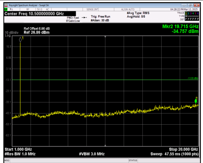
Band2-1.4MHz-64QAM-18900-1RB#0-Range2:1000~20000MHz
