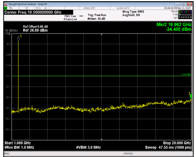
Band4-1.4MHz-64QAM-20393-1RB#0-Range2:1000~20000MHz
