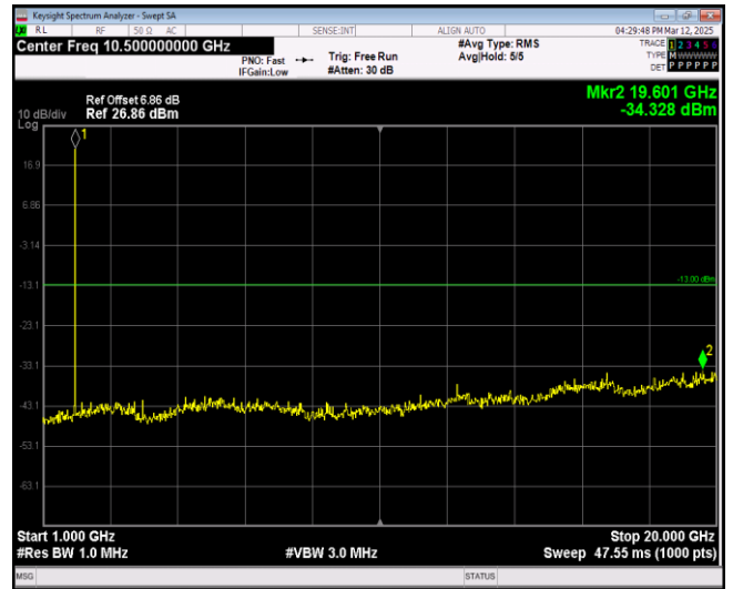
Band2-1.4MHz-64QAM-18607-1RB#0-Range2:1000~20000MHz
