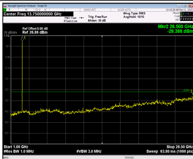
Band38-5MHz-16QAM-37775-1RB#0-Range2:1000~ 26500MHz
