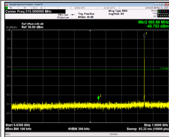
Band5-1.4MHz-16QAM-20407-1RB#0-Range1:30~10 00MHz
