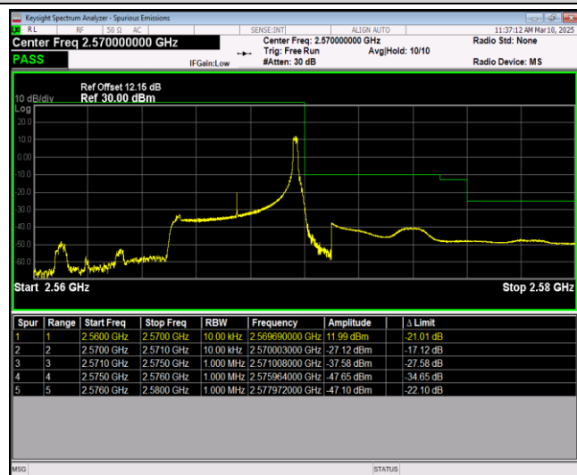
Band7-5MHz-16QAM-20775-1RB#0
