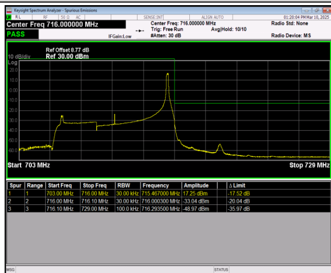
Band17-5MHz-QPSK-23755-1RB#0
