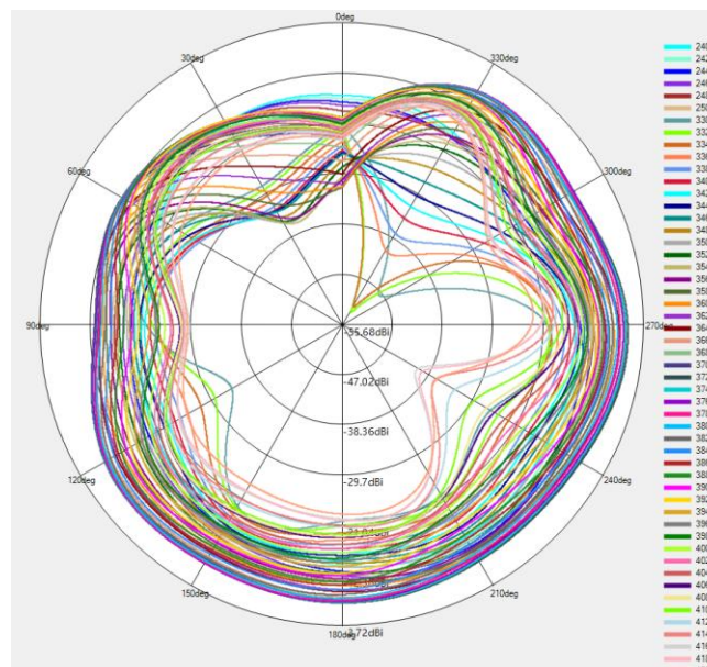
WIFI-2.4G & BT & n77/n78 \Theta=90^\circ
