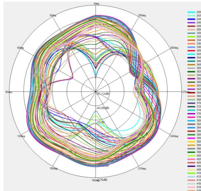
WIFI-2.4G & BT & n77/n78 \Phi=90^\circ
