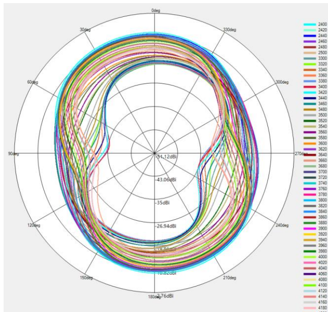
WIFI-2.4G & BT & n77/n78 Phi=0deg
