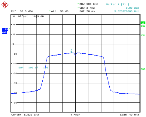
n20_5825MHz_Chain 0 -9.00dBm/MHz
