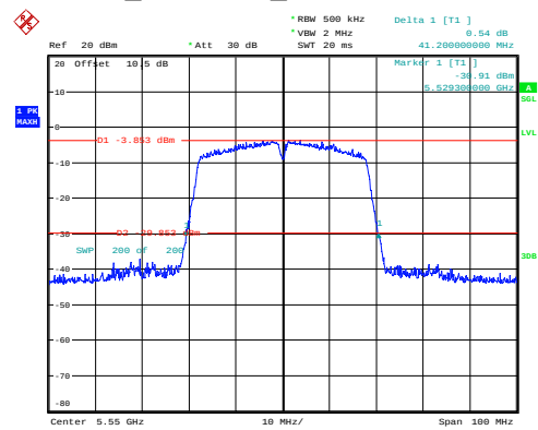
n40_5550MHz_Chain 0 41.200MHz
