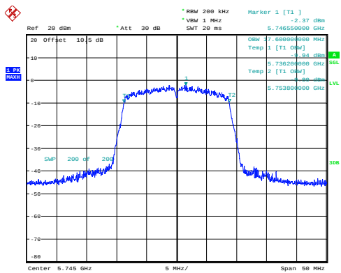
n20_5745MHz_Chain 0 17.600MHz
