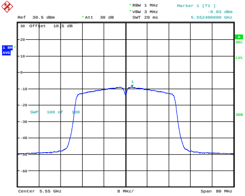
n40_5550MHz_Chain 0 -9.03dBm/MHz
