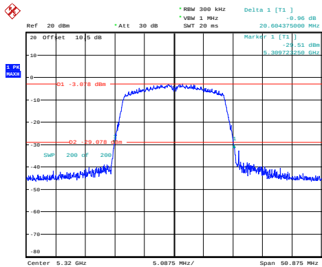
n20_5320MHz_Chain 0 20.604MHz
