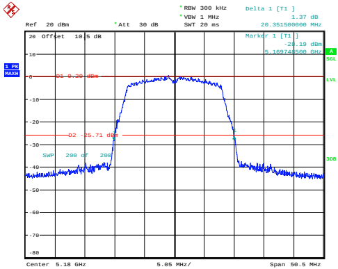
a_5180MHz_Chain 0 20.352MHz
