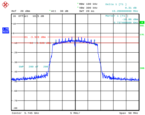
n20_5745MHz_Chain 0 15.200MHz
