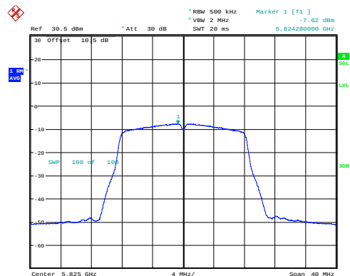
a_5825MHz_Chain 0 -7.62dBm/MHz
