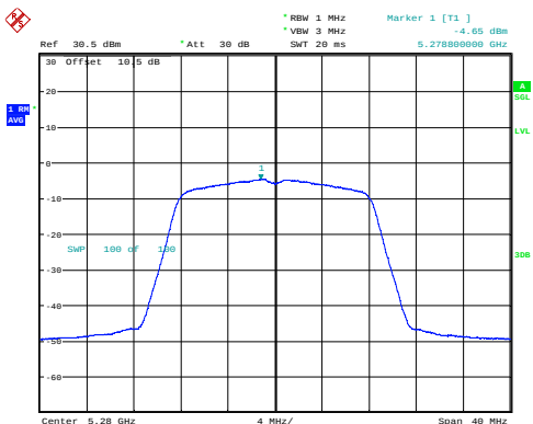
a_5280MHz_Chain 0 -4.65dBm/MHz
