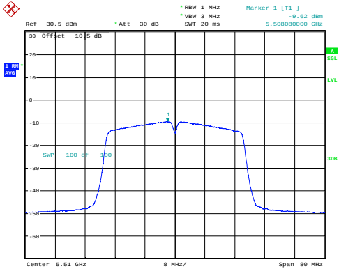
n40_5510MHz_Chain 0 -9.62dBm/MHz
