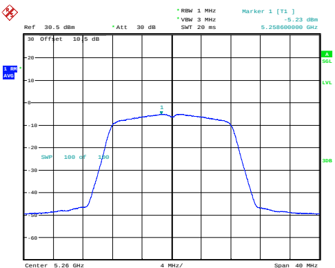
a_5260MHz_Chain 0 -5.23dBm/MHz
