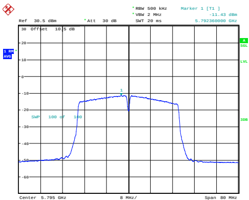
n40_5795MHz_Chain 0 -11.43dBm/MHz
