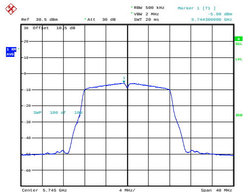
a_5745MHz_Chain 0 -5.99dBm/MHz
