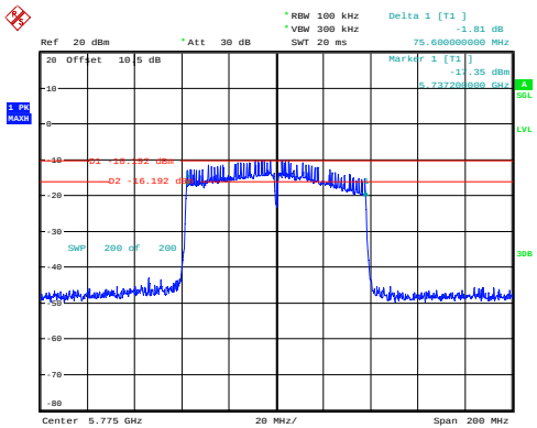
ac80_5775MHz_Chain 0 75.600MHz
