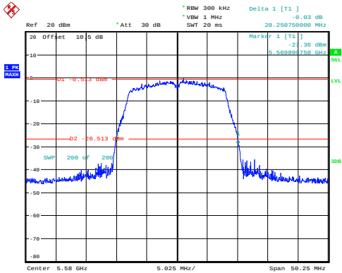
a_5580MHz_Chain 0 20.251MHz
