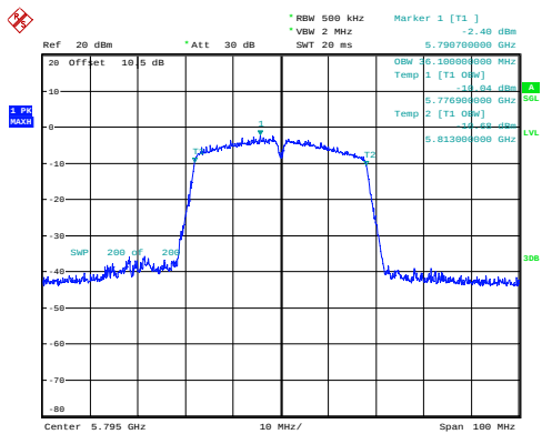
n40_5795MHz_Chain 0 36.100MHz
