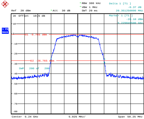
a_5240MHz_Chain 0 20.351MHz
