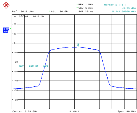
a_5240MHz_Chain 0 -3.99dBm/MHz
