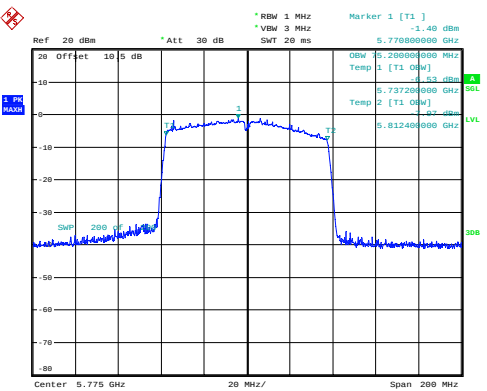
ac80_5775MHz_Chain 0 75.200MHz
