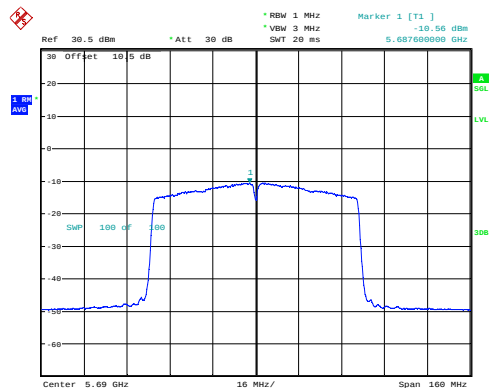
ac80_5690MHz_Chain 0 -10.56dBm/MHz
