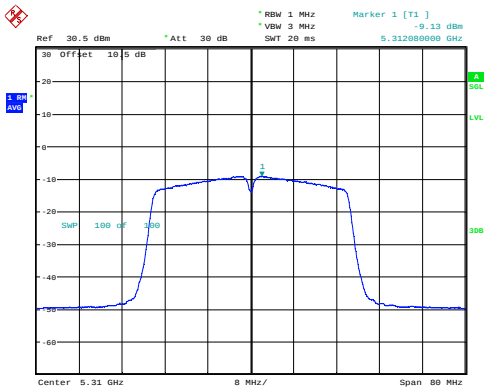
n40_5310MHz_Chain 0 -9.13dBm/MHz
