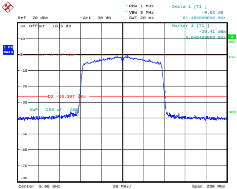
ac80_5690MHz_Chain 0 81.400MHz
