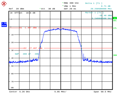
a_5260MHz_Chain 0 20.251MHz
