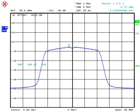
n20_5580MHz_Chain 0 -5.73dBm/MHz
