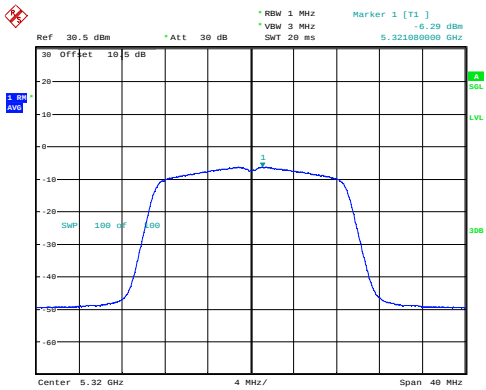
n20_5320MHz_Chain 0 -6.29dBm/MHz
