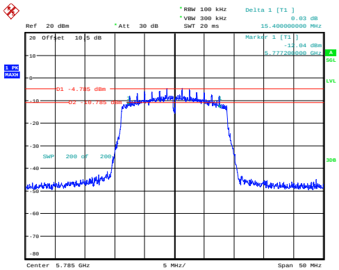
n20_5785MHz_Chain 0 15.400MHz
