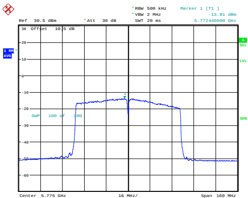
ac80_5775MHz_Chain 0 -13.81dBm/MHz
