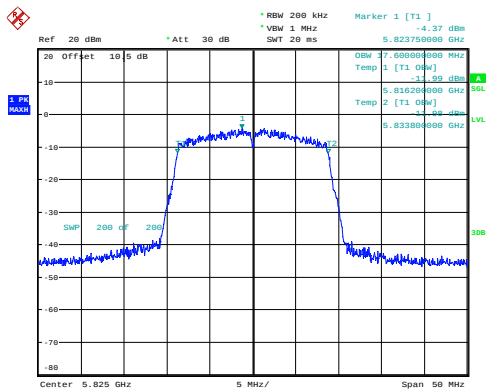
n20_5825MHz_Chain 0 17.600MHz
