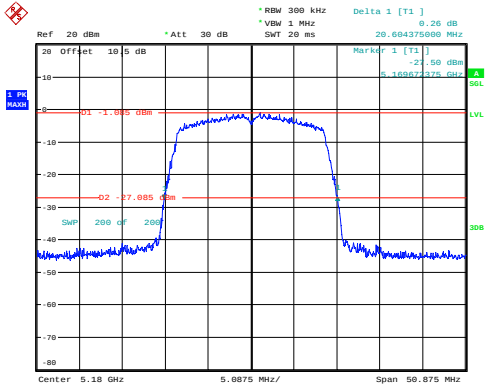
n20_5180MHz_Chain 0 20.604MHz
