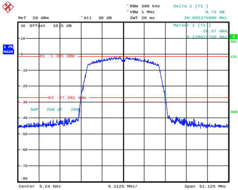
n20_5240MHz_Chain 0 20.603MHz
