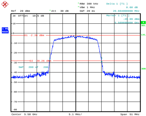
n20_5580MHz_Chain 0 20.604MHz
