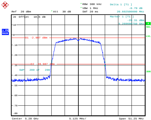
n20_5280MHz_Chain 0 20.603MHz
