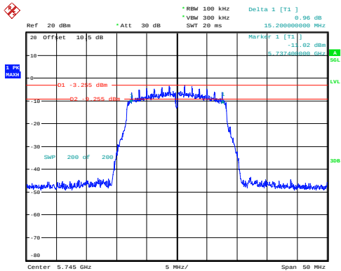
a_5745MHz_Chain 0 15.200MHz
