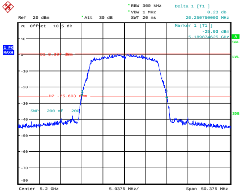
a_5200MHz_Chain 0 20.251MHz
