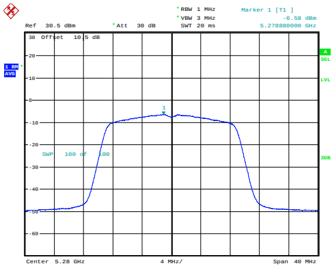
n20_5280MHz_Chain 0 -6.58dBm/MHz
