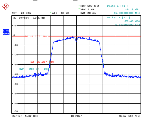
n40_5670MHz_Chain 0 41.300MHz
