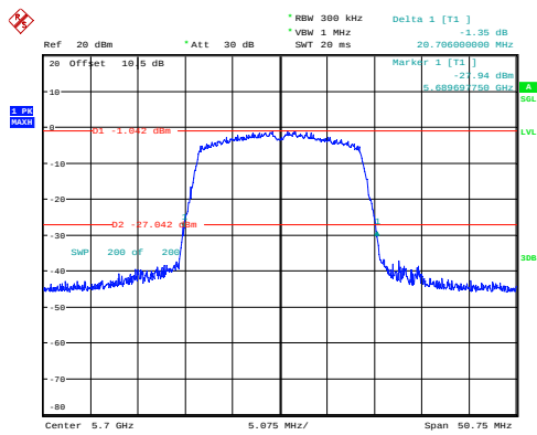
n20_5700MHz_Chain 0 20.706MHz
