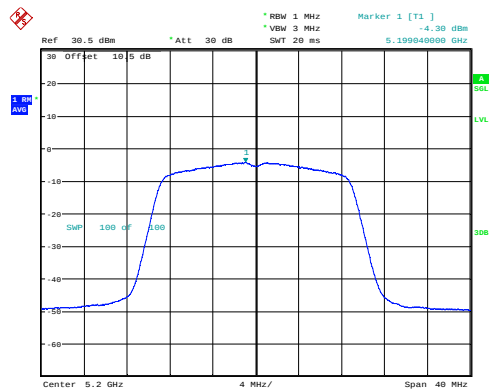
n20_5200MHz_Chain 0 -4.30dBm/MHz
