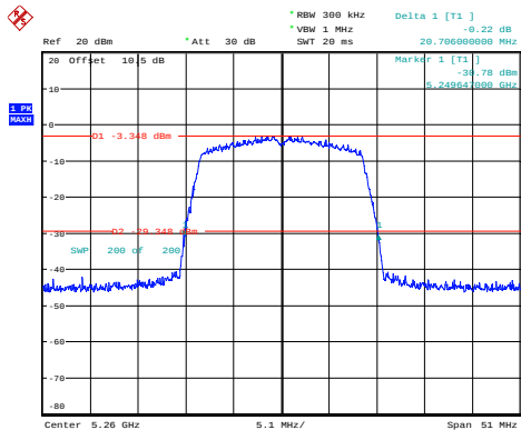
n20_5260MHz_Chain 0 20.706MHz
