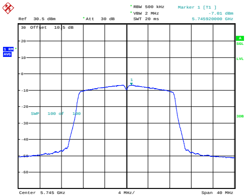
n20_5745MHz_Chain 0 -7.01dBm/MHz
