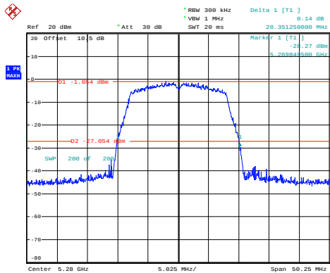
a_5280MHz_Chain 0 20.351MHz
