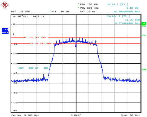
a_5785MHz_Chain 0 15.200MHz
