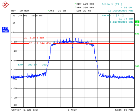
n20_5825MHz_Chain 0 15.200MHz
