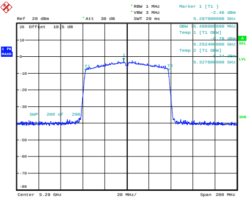
ac80_5290MHz_Chain 0 75.400MHz
