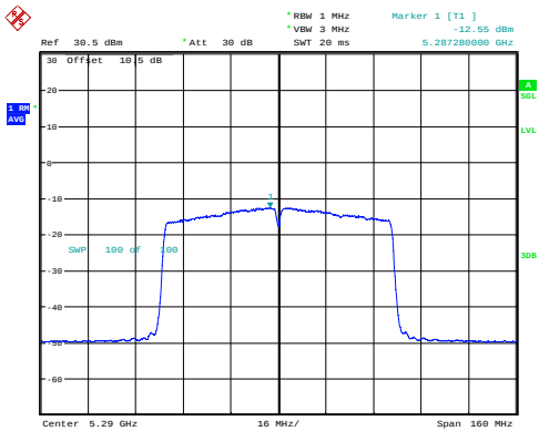
ac80_5290MHz_Chain 0 -12.55dBm/MHz
