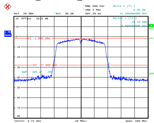
n40_5710MHz_Chain 0 41.300MHz
