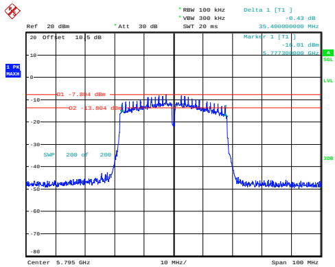
n40_5795MHz_Chain 0 35.400MHz
