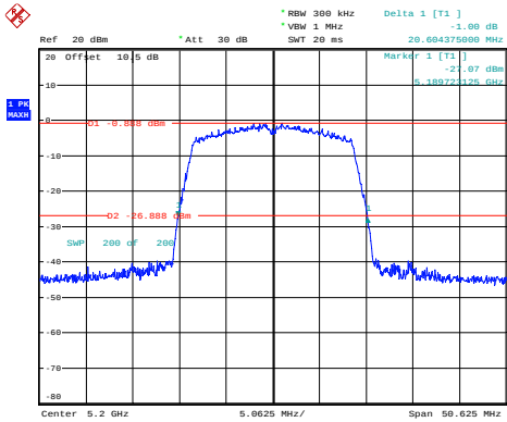
n20_5200MHz_Chain 0 20.604MHz
