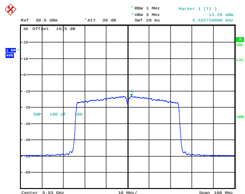
ac80_5530MHz_Chain 0 -13.29dBm/MHz
