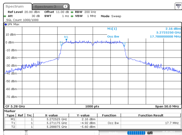
n20_5280MHz_Chain 0
