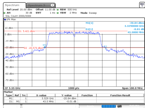
n40_5550MHz_Chain 0
