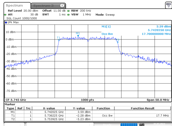
n20_5745MHz_Chain 0
