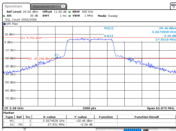
n20_5580MHz_Chain 0
