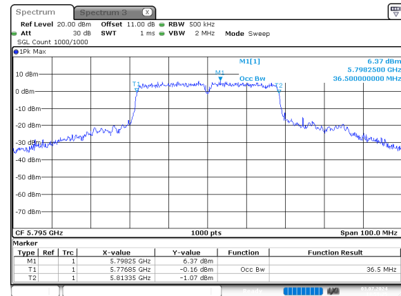
n40_5795MHz_Chain 0
