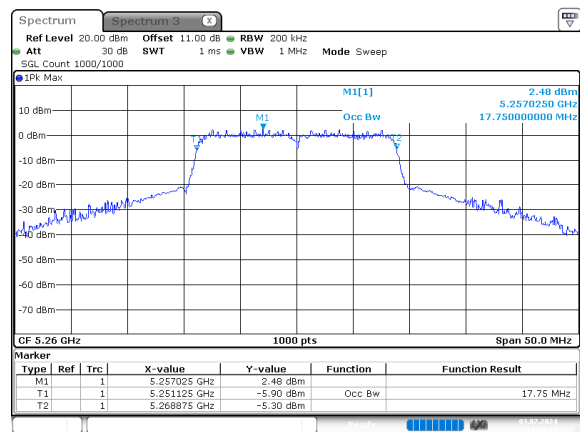
n20_5260MHz_Chain 0
