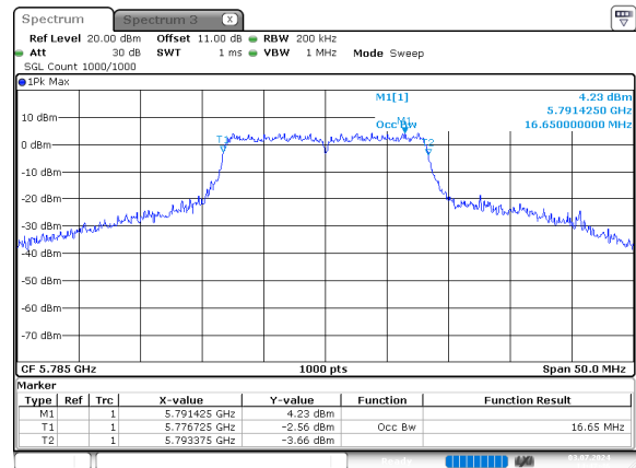
a_5785MHz_Chain 0
