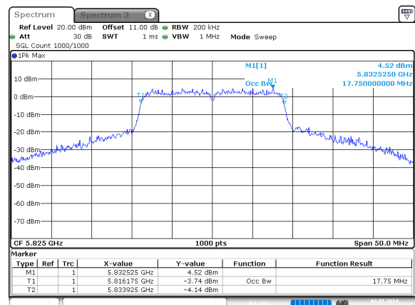
n20_5825MHz_Chain 0
