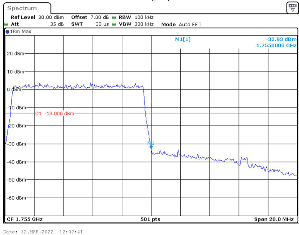
Band 4_10 MHz_High_QPSK_RB50#0
