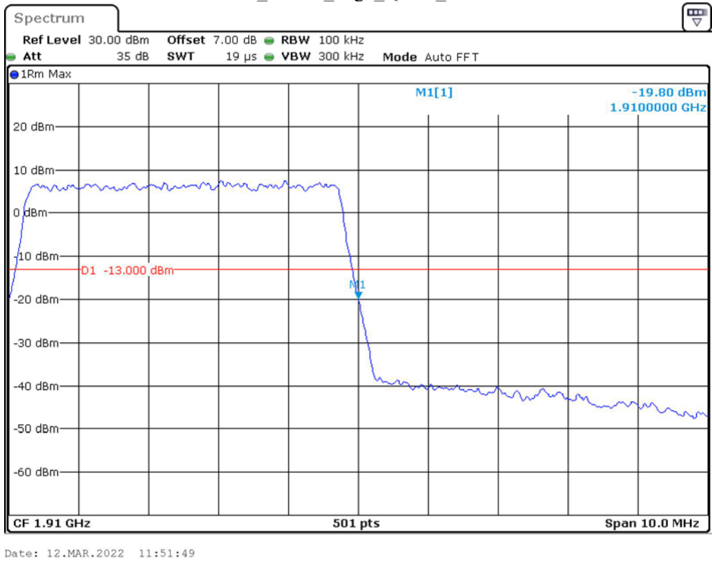
Band 2_5 MHz_High_QPSK_RB25#0
