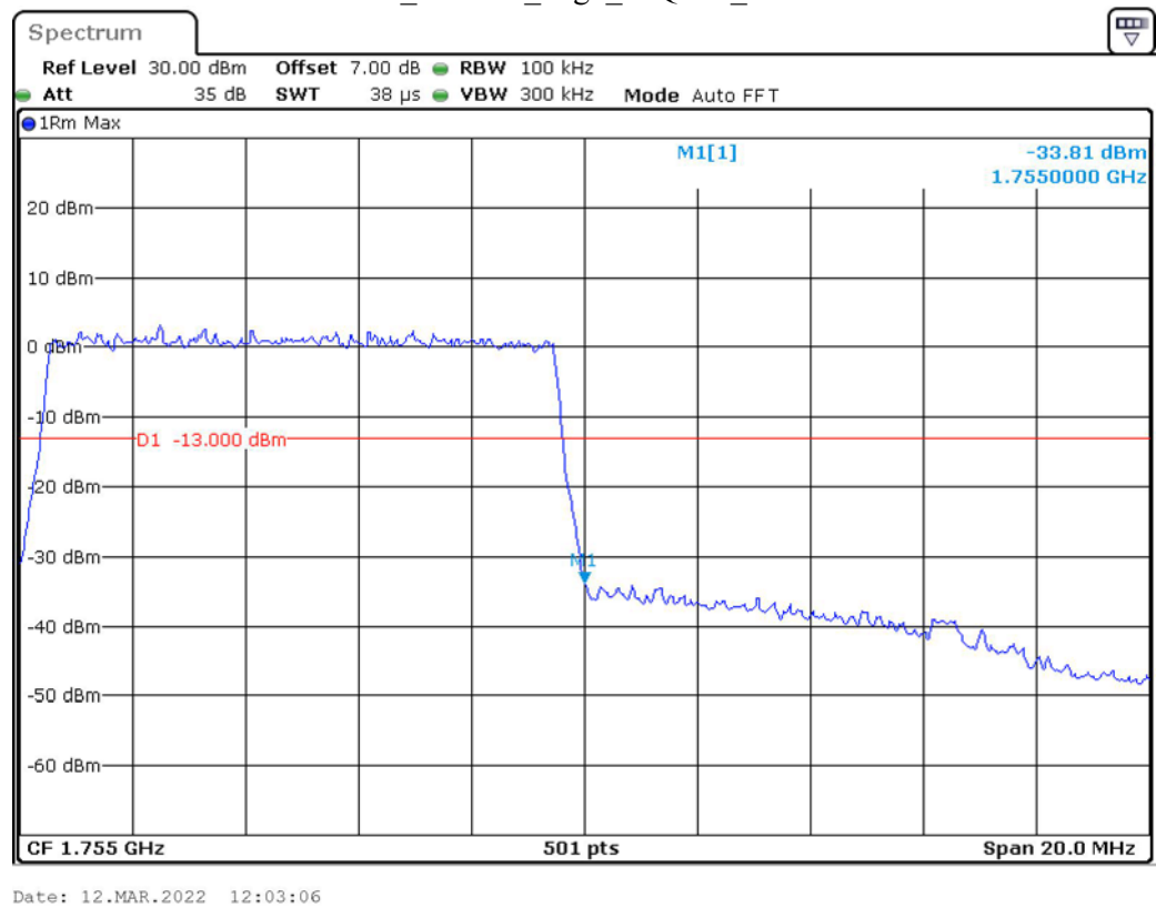
Band 4_10 MHz_High_16QAM_RB50#0
