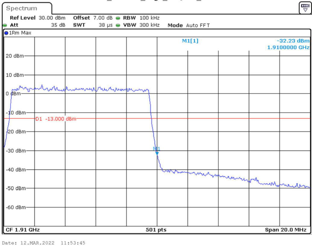
Band 2_10 MHz_High_16QAM_RB50#0
