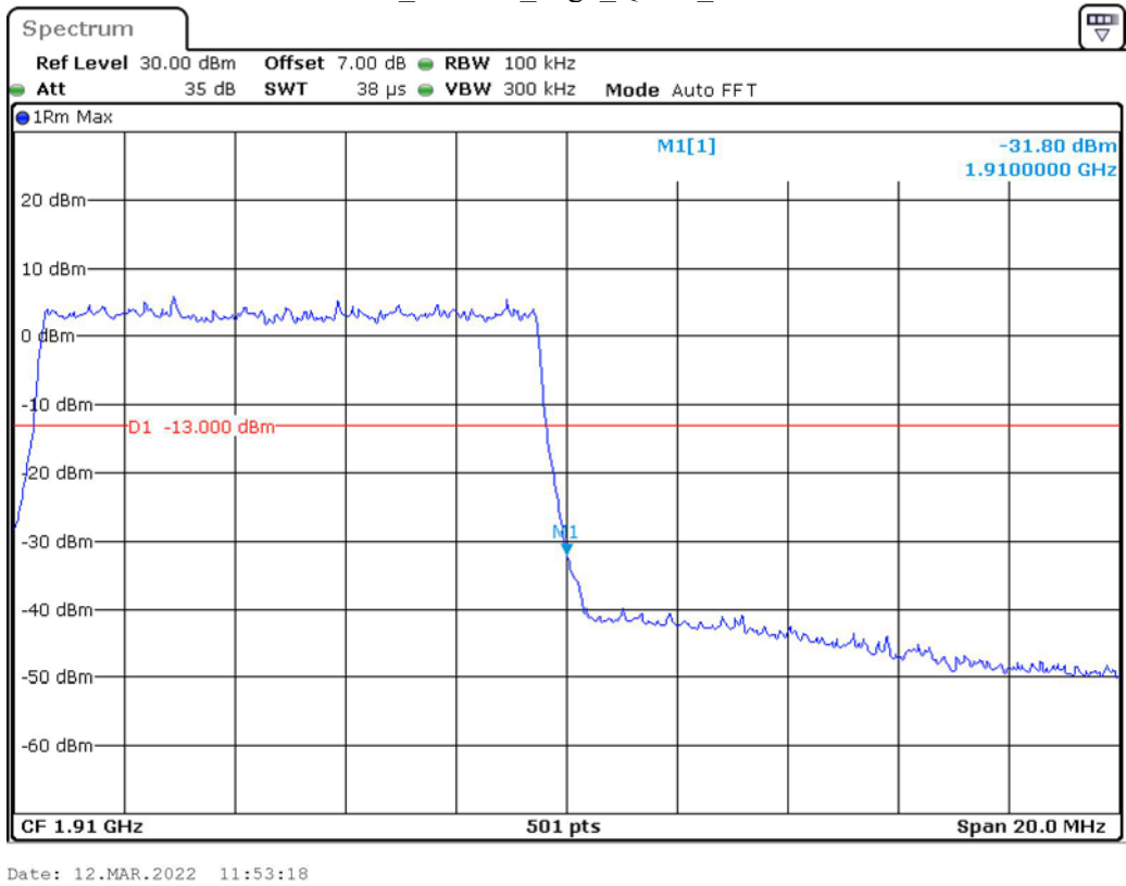
Band 2_10 MHz_High_QPSK_RB50#0
