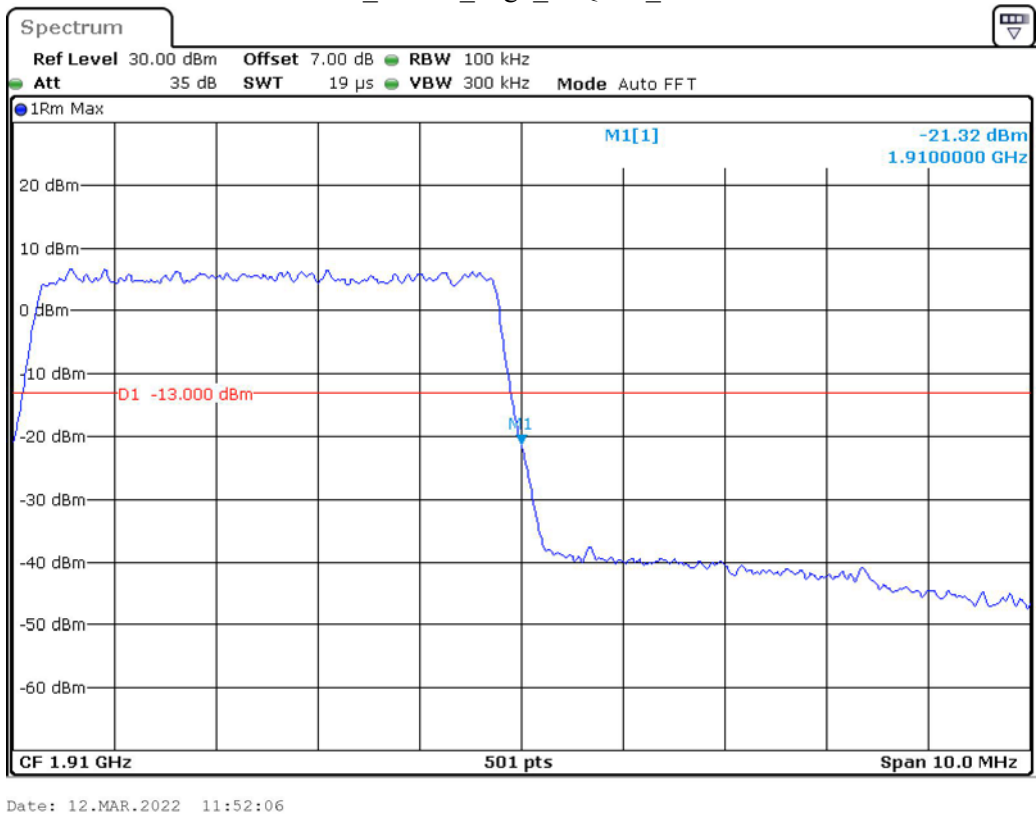
Band 2_5 MHz_High_16QAM_RB25#0
