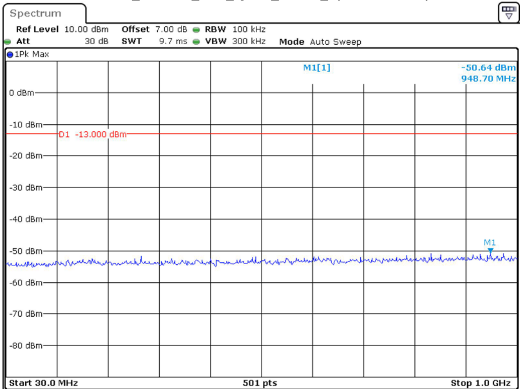
Band 2_1.4 MHz_Low_QPSK_RB6#0_1(30MHz-1GHz)
