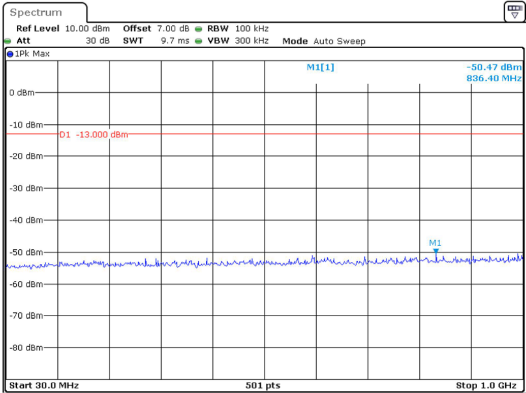
Band 2_10 MHz_High_QPSK_RB50#0_1(30MHz-1GHz)
