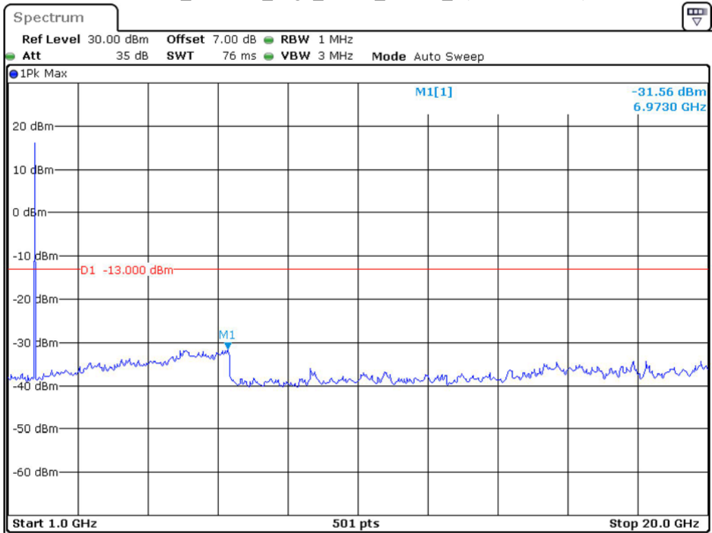
Band 4_1.4 MHz_High_QPSK_RB6#0_2(1GHz-20GHz)
