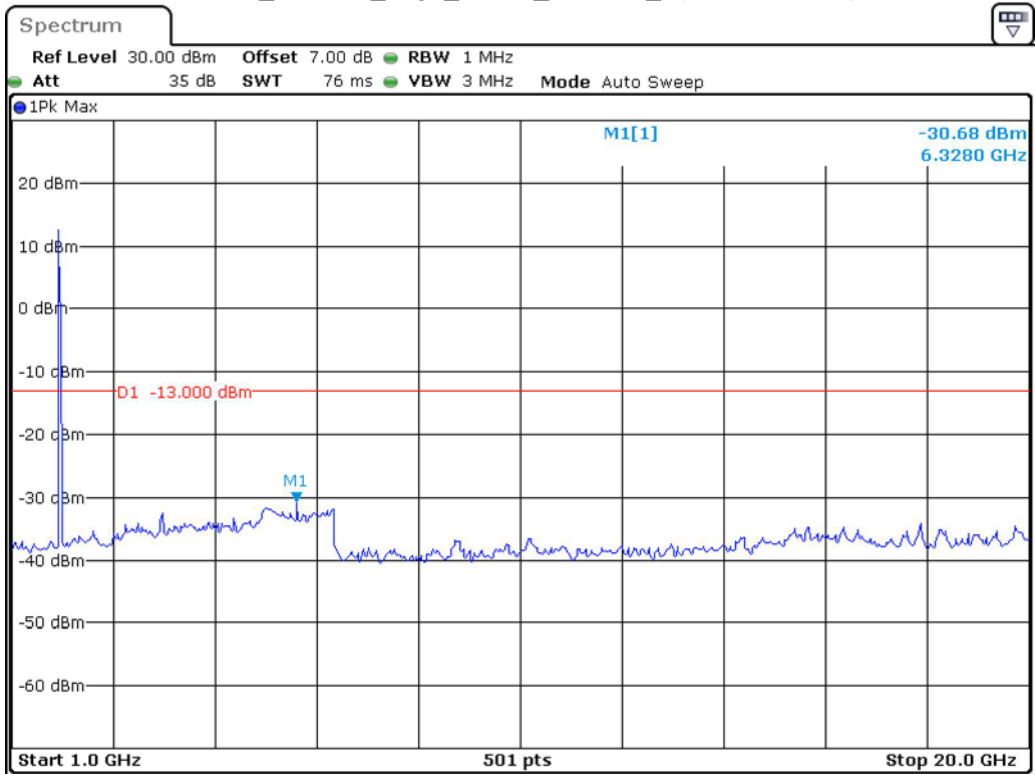
Band 2_10 MHz_High_QPSK_RB50#0_2(1GHz-20GHz)
