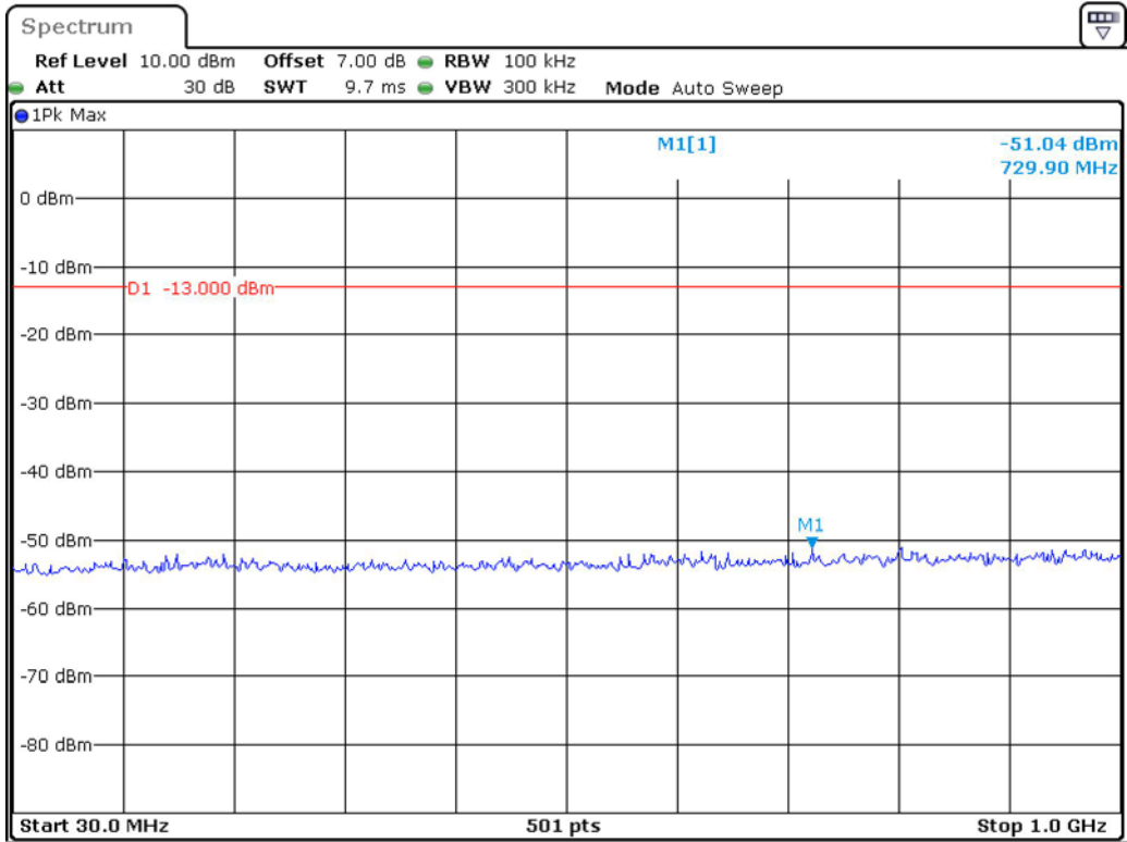
Band 4_1.4 MHz_High_QPSK_RB6#0_1(30MHz-1GHz)
