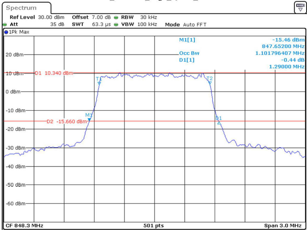
Band 5_1.4 MHz_High_QPSK_RB6#0
