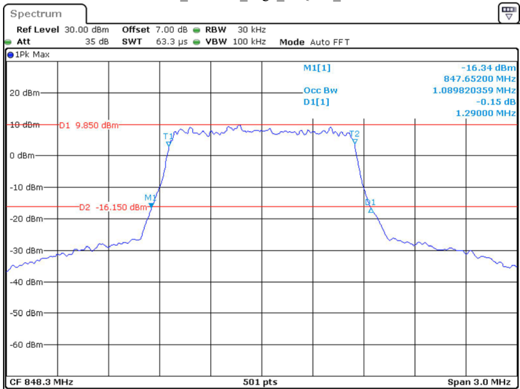
Band 5_1.4 MHz_High_16QAM_RB6#0
