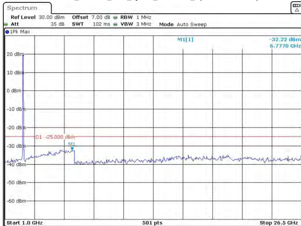
Band 38_20 MHz_Low_QPSK_RB100#0_2(1GHz-26.5GHz)
