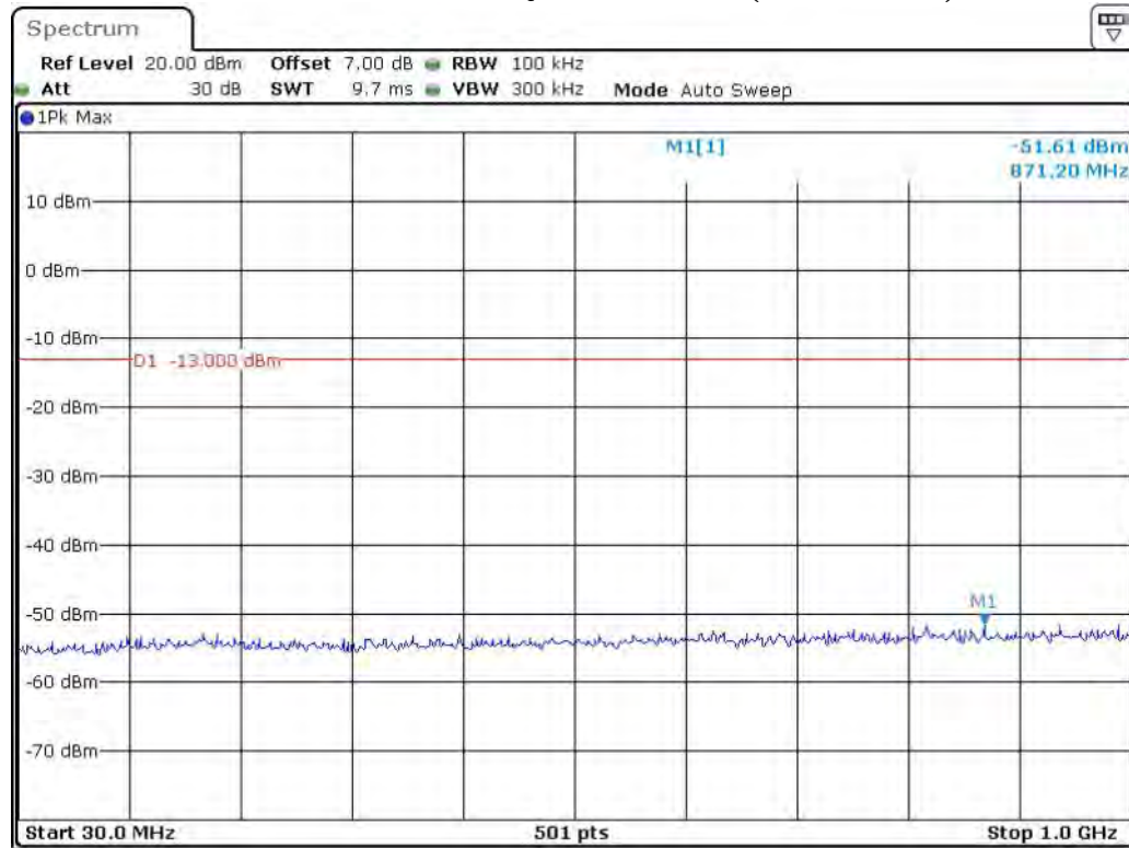
Band 2_3 MHz_Middle_QPSK_RB15#0_1(30MHz-1GHz)
