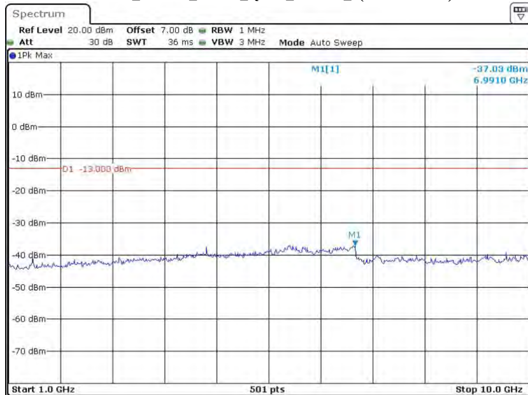
Band 17_10 MHz_Middle_QPSK_RB50#0_2(1GHz-10GHz)
