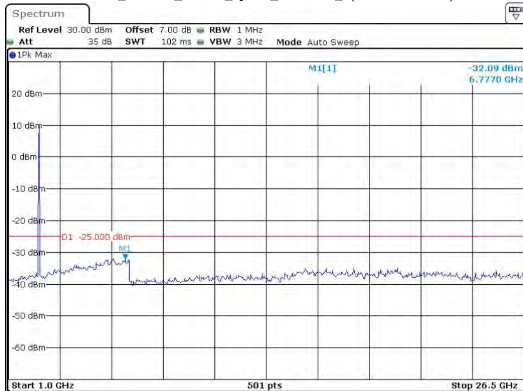
Band 7_20 MHz_Middle_QPSK_RB100#0_2(1GHz-26.5GHz)
