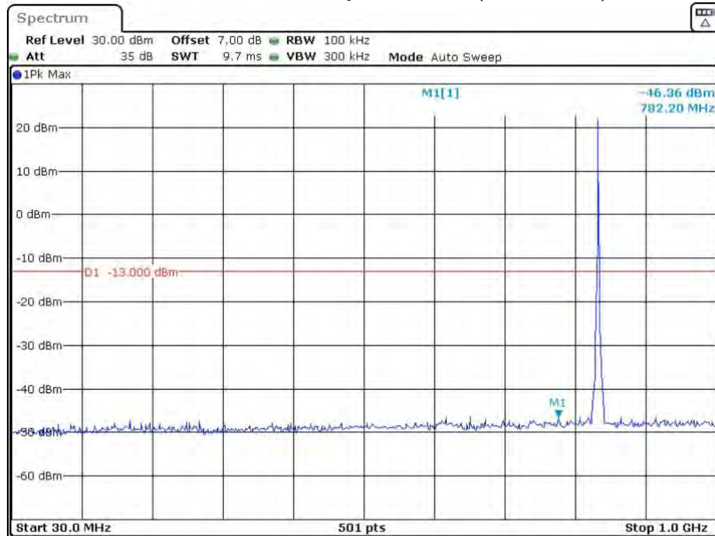
Band 5_1.4 MHz_Middle_QPSK_RB6#0_1(30MHz-1GHz)
