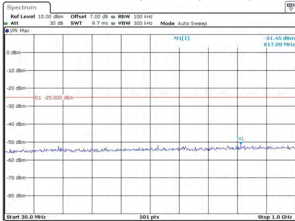
Band 7_15 MHz_Middle_QPSK_RB75#0_1(30MHz-1GHz)
