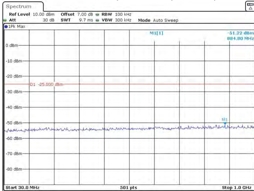
Band 38_20 MHz_Low_QPSK_RB100#0_1(30MHz-1GHz)
