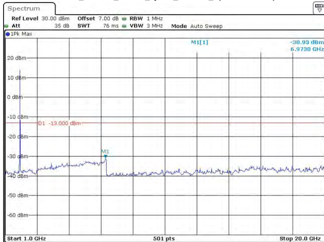
Band 2_10 MHz_Middle_QPSK_RB50#0_2(1GHz-20GHz)
