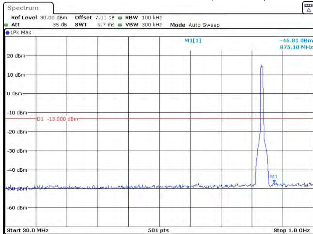
Band 5_10 MHz_Middle_QPSK_RB50#0_1(30MHz-1GHz)
