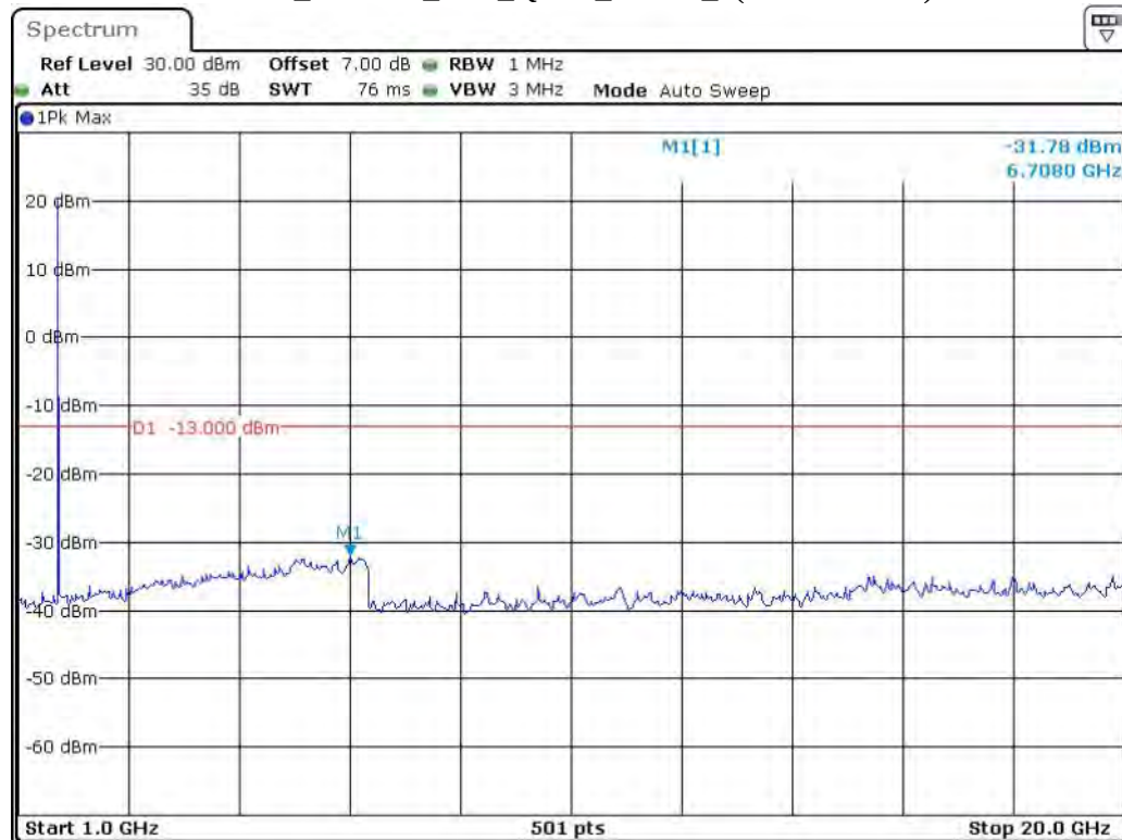
Band 4_1.4 MHz_Low_QPSK_RB6#0_2(1GHz-20GHz)
