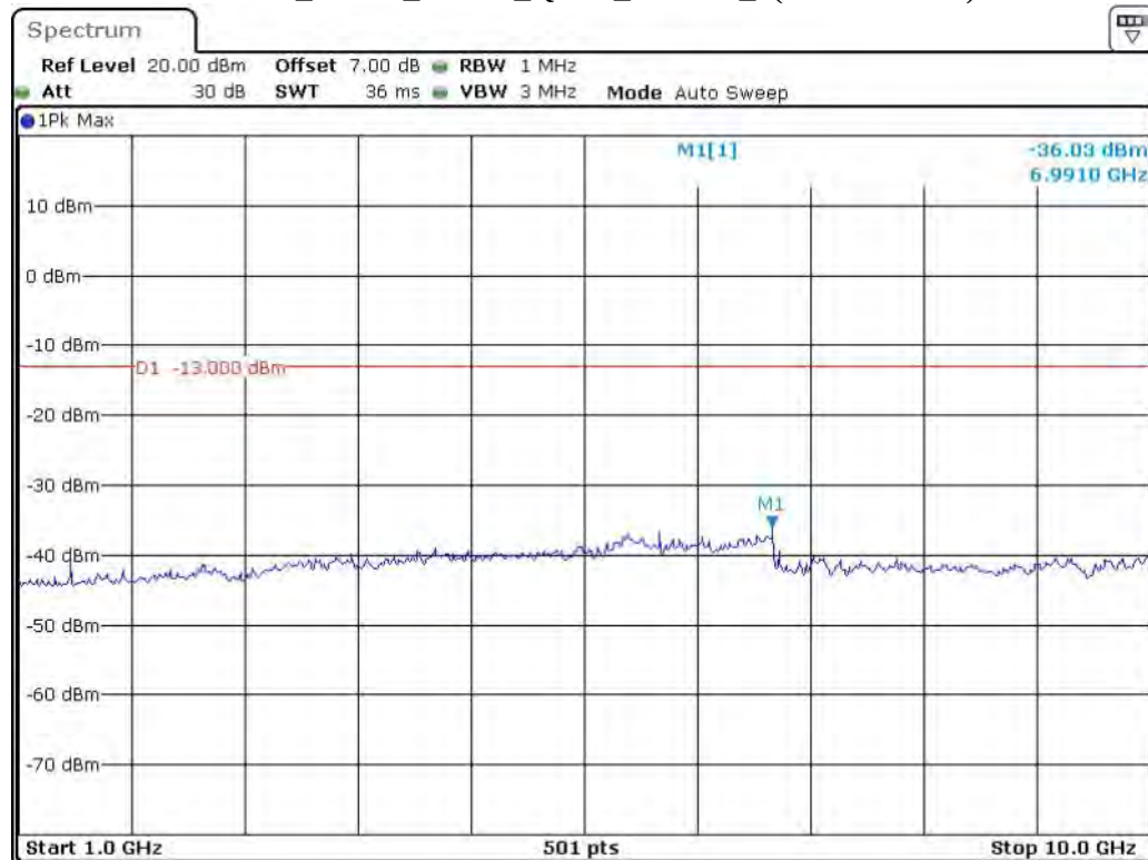
Band 17_5 MHz_Middle_QPSK_RB25#0_2(1GHz-10GHz)
