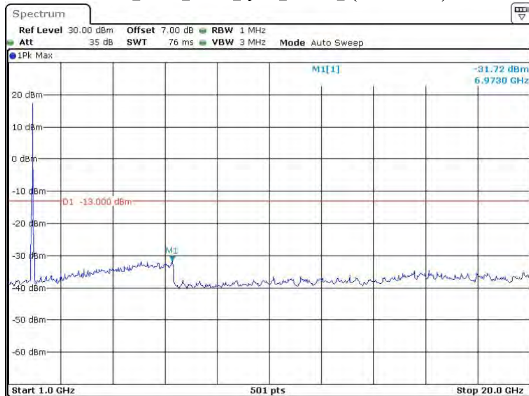
Band 2_3 MHz_Middle_QPSK_RB15#0_2(1GHz-20GHz)
