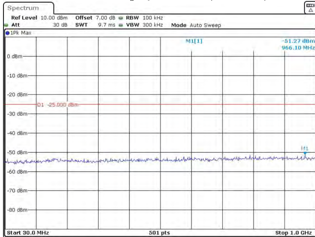
Band 38_15 MHz_High_QPSK_RB75#0_1(30MHz-1GHz)
