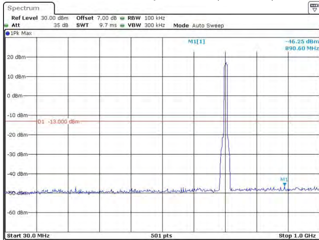
Band 17_10 MHz_Middle_QPSK_RB50#0_1(30MHz-1GHz)
