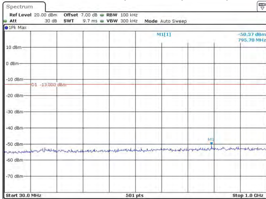
Band 4_20 MHz_Middle_QPSK_RB100#0_1(30MHz-1GHz)
