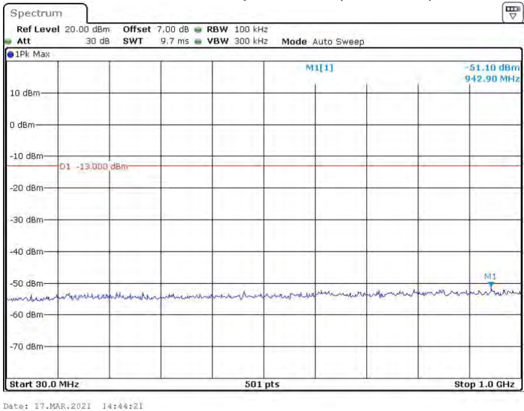
Band 2_1.4 MHz_Low_QPSK_RB6#0_1(30MHz-1GHz)
