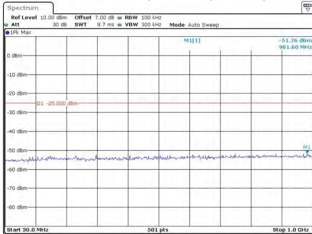
Band 7_10 MHz_Middle_QPSK_RB50#0_1(30MHz-1GHz)
