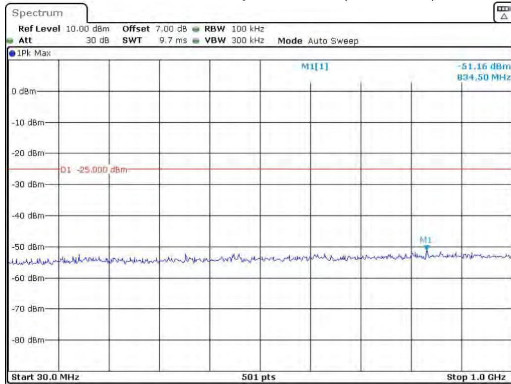
Band 38_5 MHz_Middle_QPSK_RB25#0_1(30MHz-1GHz)
