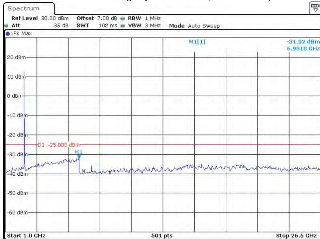
Band 7_10 MHz_High_QPSK_RB50#0_2(1GHz-26.5GHz)
