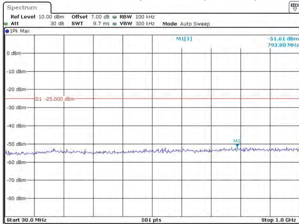
Band 7_20 MHz_Middle_QPSK_RB100#0_1(30MHz-1GHz)
