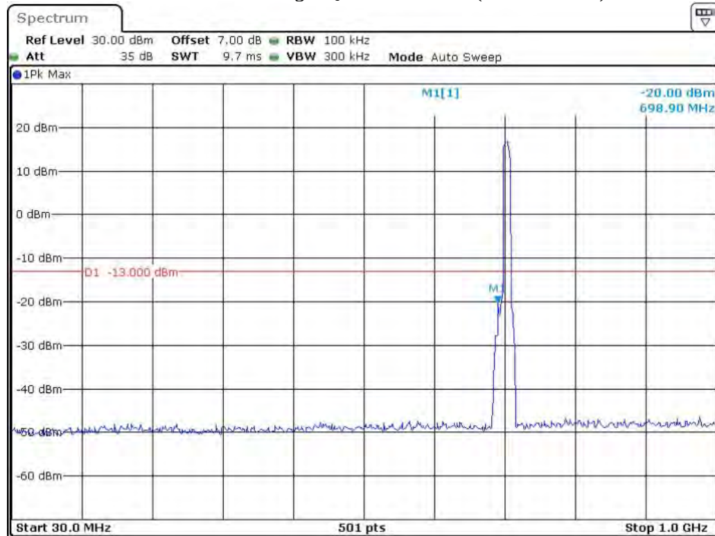
Band 17_10 MHz_High_QPSK_RB50#0_1(30MHz-1GHz)
