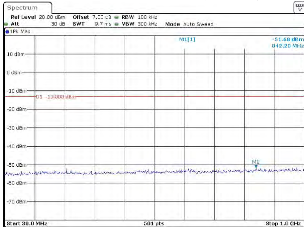
Band 2_10 MHz_Middle_QPSK_RB50#0_1(30MHz-1GHz)
