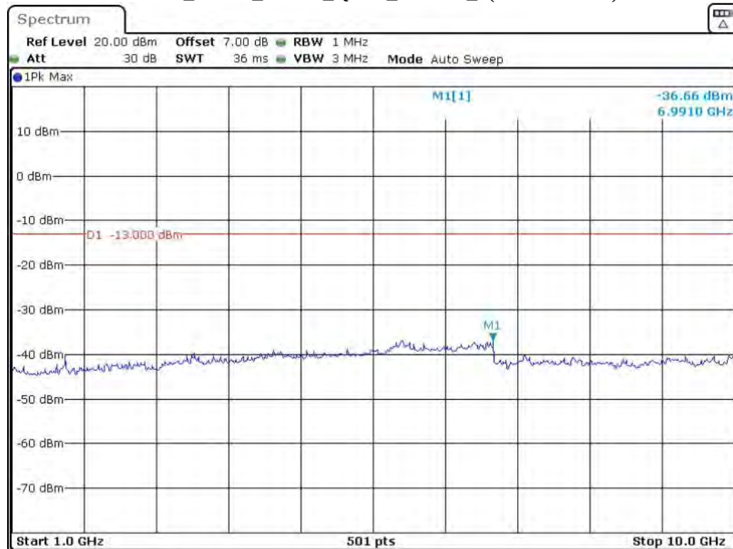
Band 5_3 MHz_Middle_QPSK_RB15#0_2(1GHz-10GHz)
