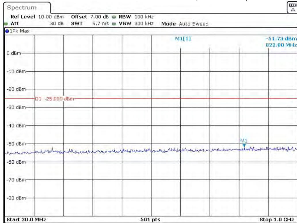
Band 38_5 MHz_Low_QPSK_RB25#0_1(30MHz-1GHz)
