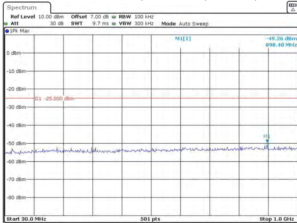
Band 38_20 MHz_Middle_QPSK_RB100#0_1(30MHz-1GHz)
