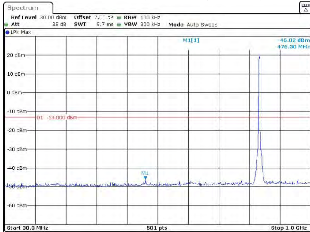
Band 5_3 MHz_Middle_QPSK_RB15#0_1(30MHz-1GHz)
