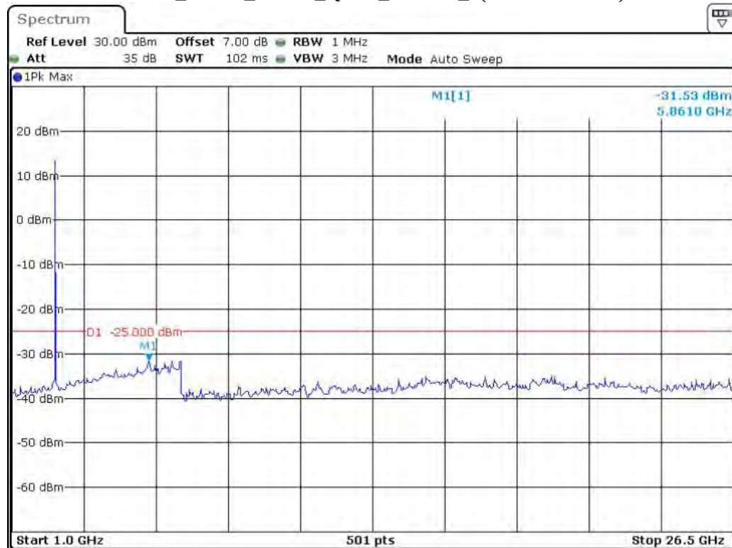
Band 7_5 MHz_Middle_QPSK_RB25#0_2(1GHz-26.5GHz)
