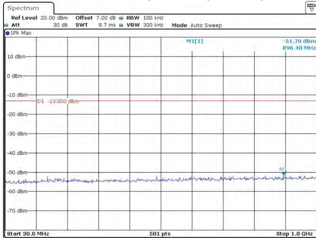
Band 4_1.4 MHz_Low_QPSK_RB6#0_1(30MHz-1GHz)
