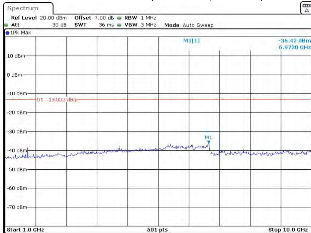
Band 5_1.4 MHz_Middle_QPSK_RB6#0_2(1GHz-10GHz)
