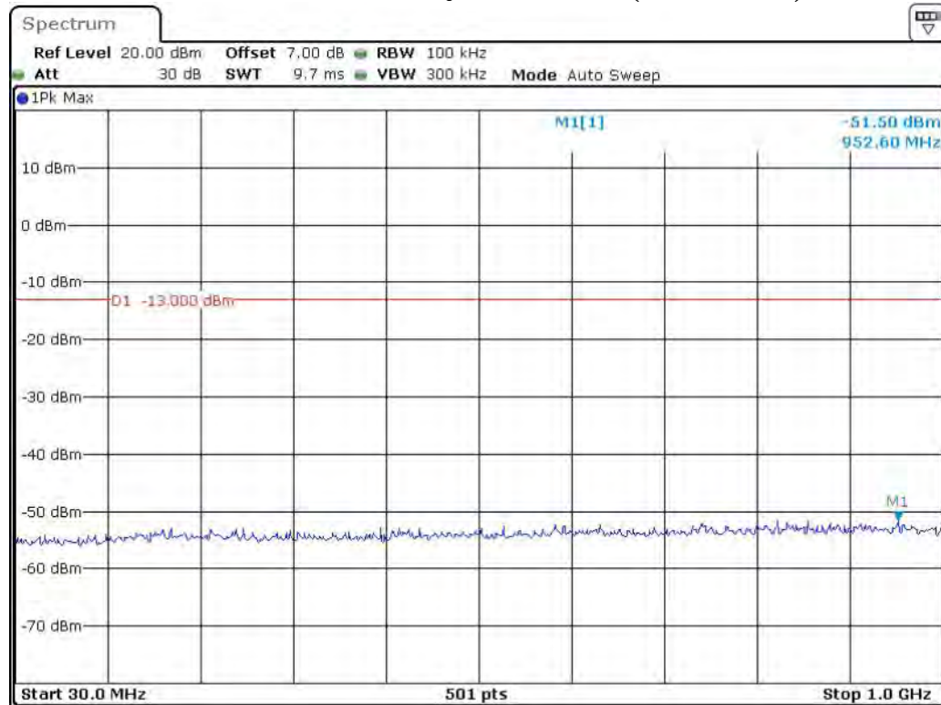
Band 2_15 MHz_Middle_QPSK_RB75#0_1(30MHz-1GHz)
