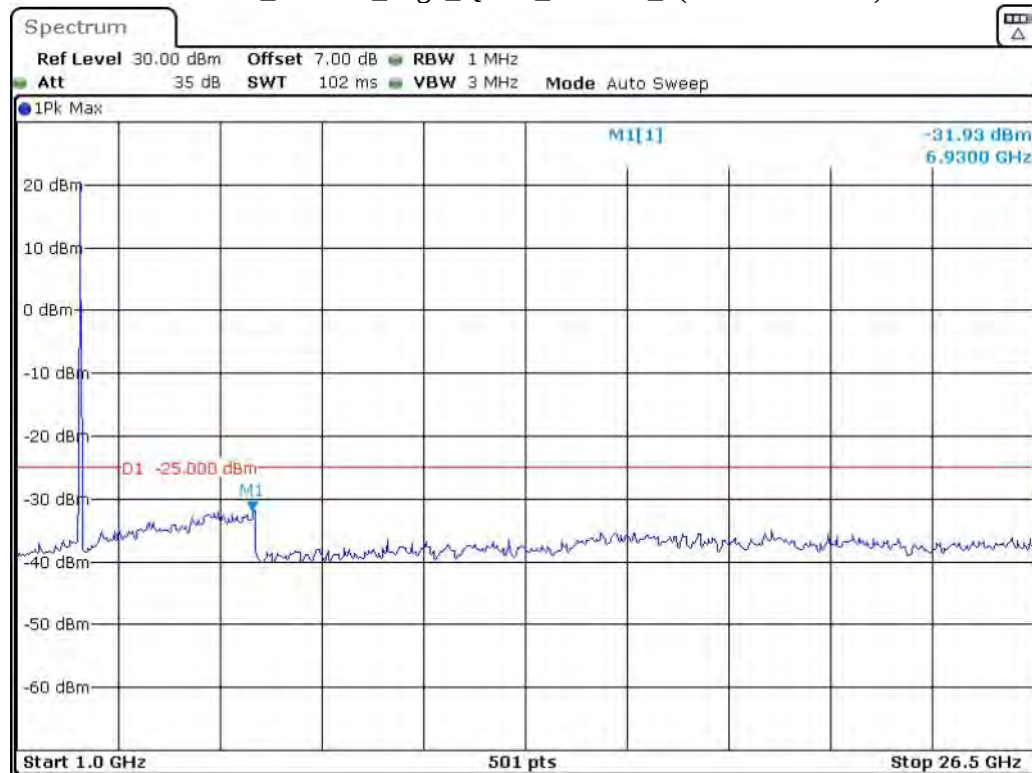
Band 38_15 MHz_High_QPSK_RB75#0_2(1GHz-26.5GHz)
