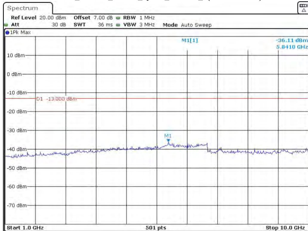
Band 5_10 MHz_Middle_QPSK_RB50#0_2(1GHz-10GHz)
