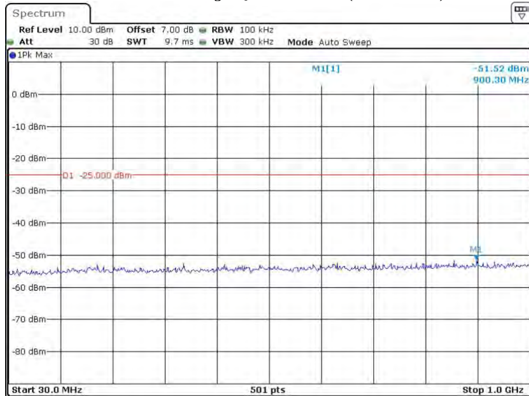
Band 7_10 MHz_High_QPSK_RB50#0_1(30MHz-1GHz)
