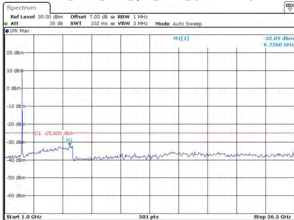
Band 7_15 MHz_Middle_QPSK_RB75#0_2(1GHz-26.5GHz)
