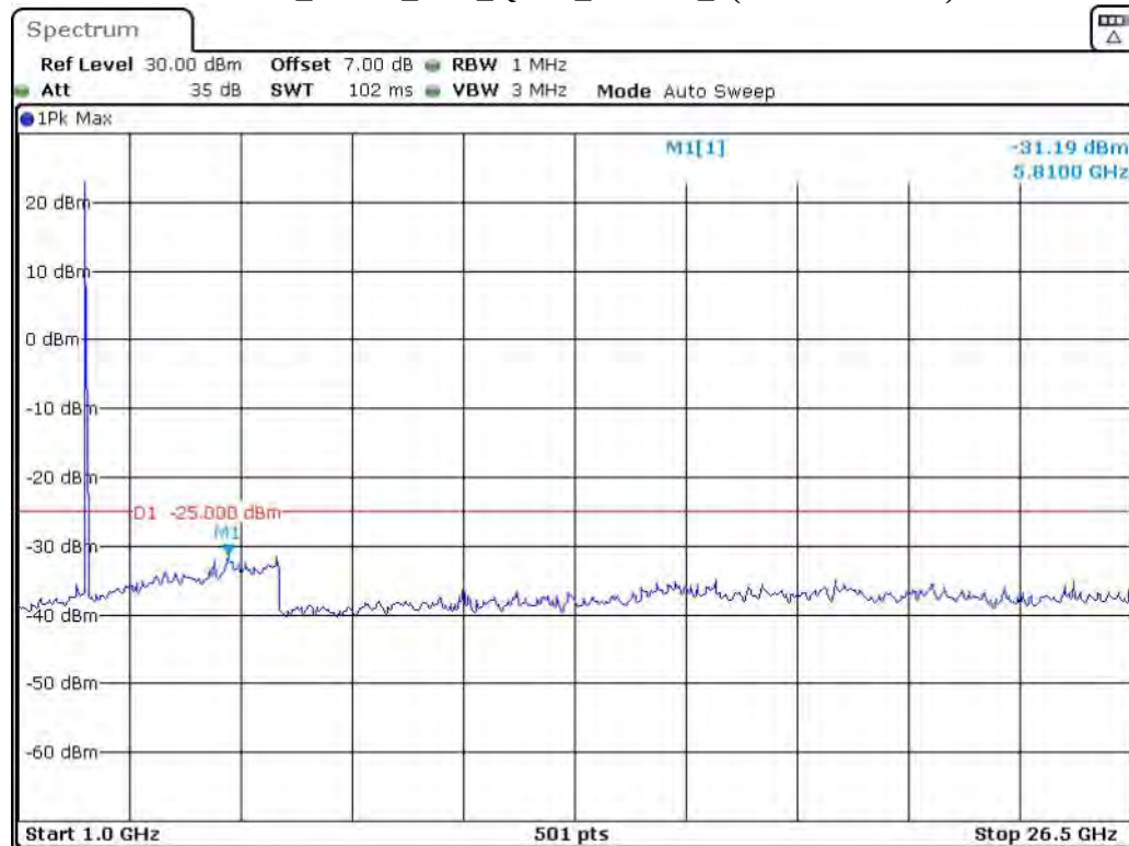
Band 38_5 MHz_Low_QPSK_RB25#0_2(1GHz-26.5GHz)
