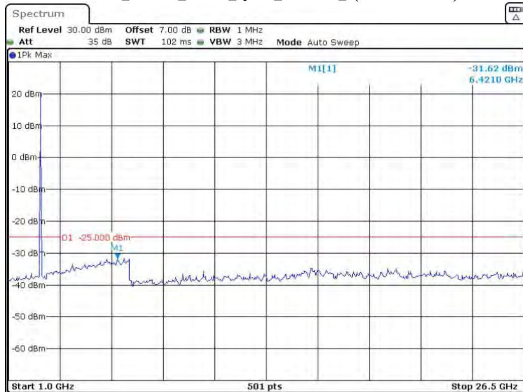
Band 38_20 MHz_Middle_QPSK_RB100#0_2(1GHz-26.5GHz)
