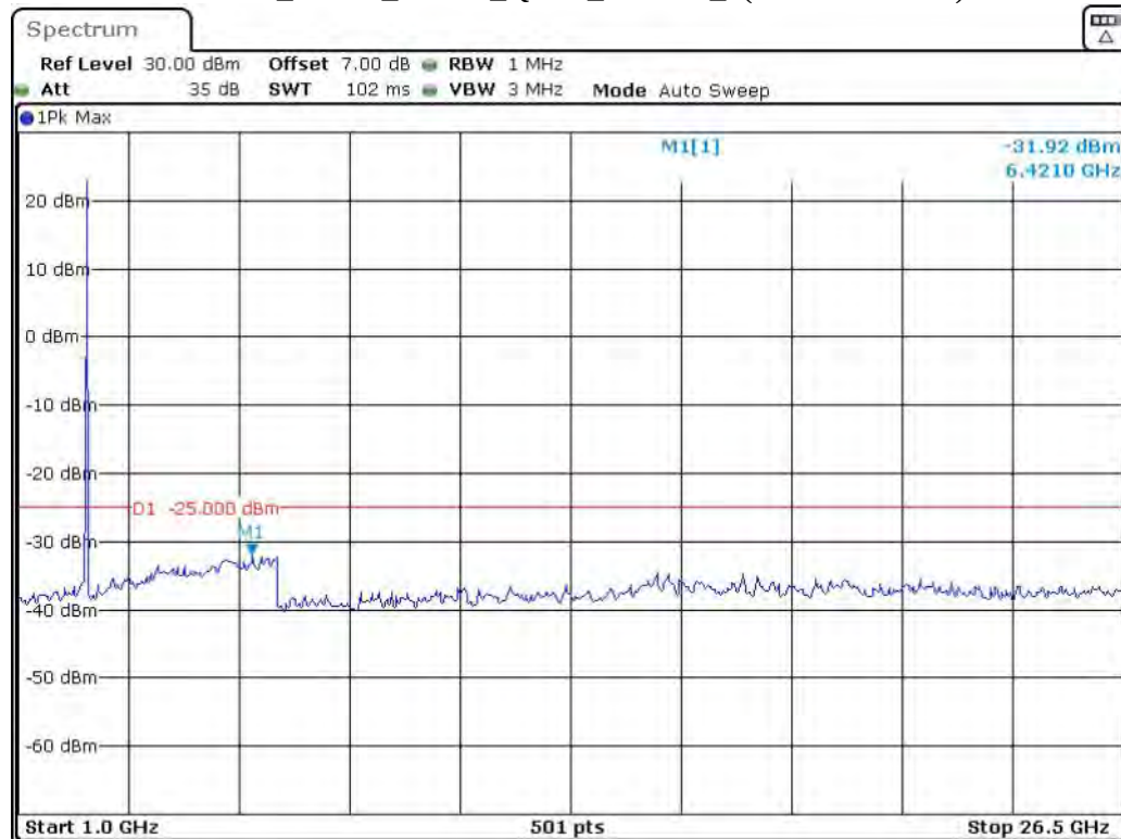
Band 38_5 MHz_Middle_QPSK_RB25#0_2(1GHz-26.5GHz)
