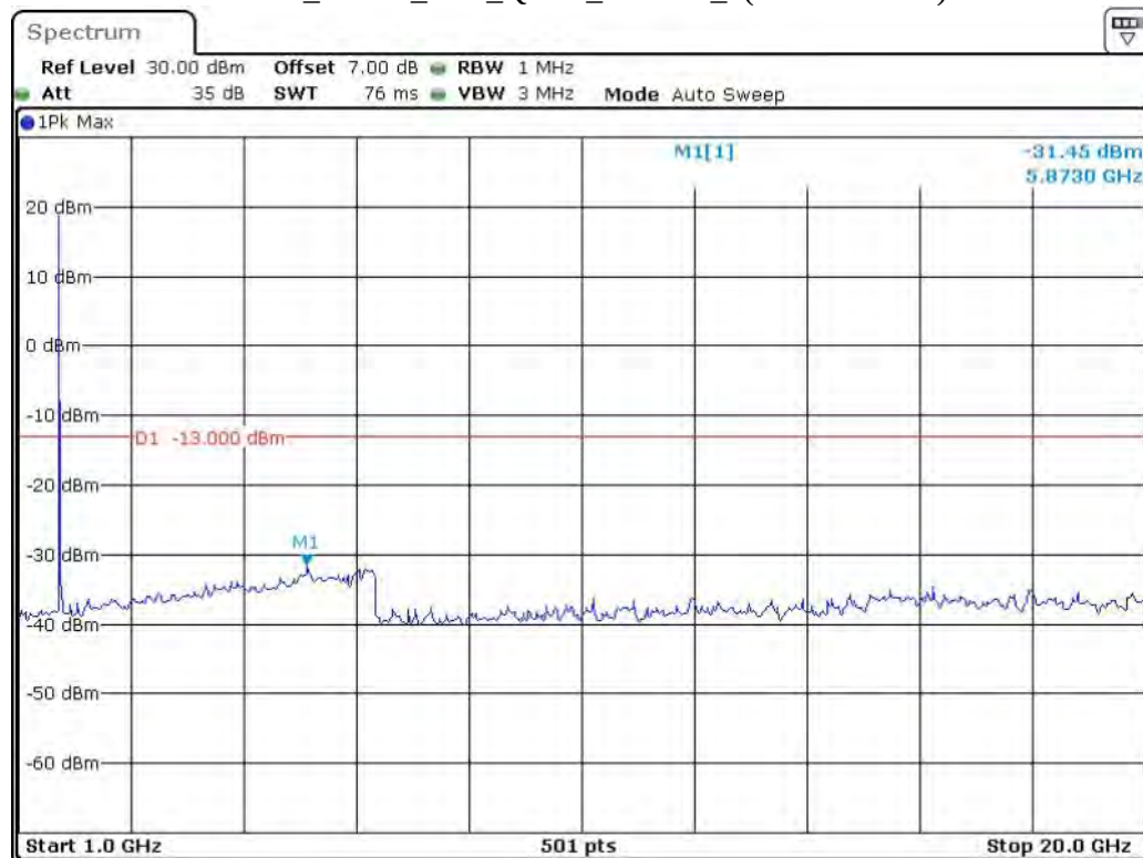
Band 4_3 MHz_Low_QPSK_RB15#0_2(1GHz-20GHz)
