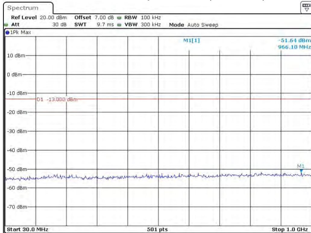
Band 4_10 MHz_Middle_QPSK_RB50#0_1(30MHz-1GHz)
