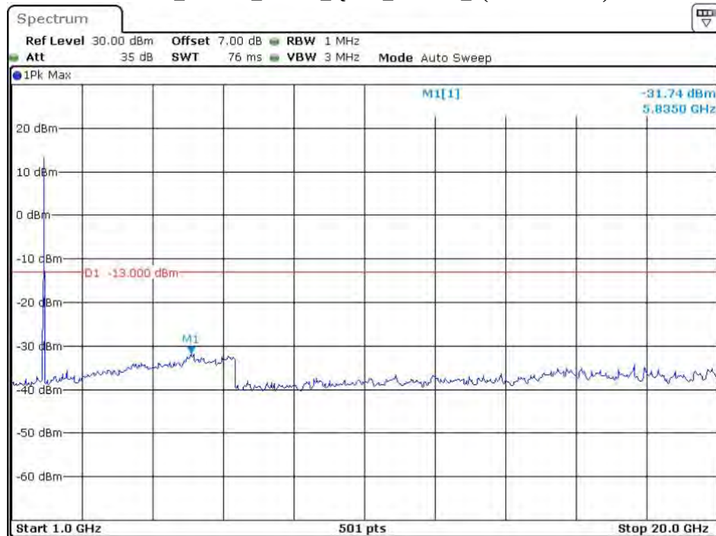
Band 2_15 MHz_Middle_QPSK_RB75#0_2(1GHz-20GHz)
