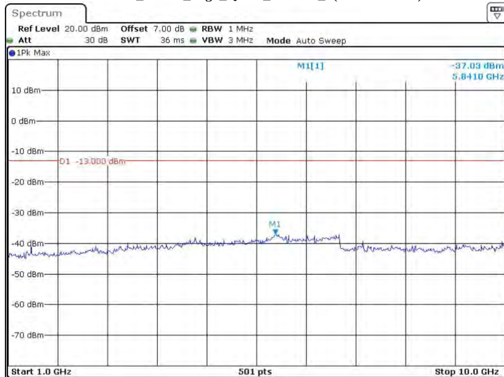
Band 17_5 MHz_High_QPSK_RB25#0_2(1GHz-10GHz)
