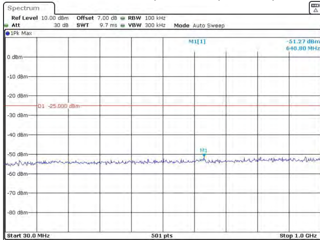
Band 38_15 MHz_Middle_QPSK_RB75#0_1(30MHz-1GHz)
