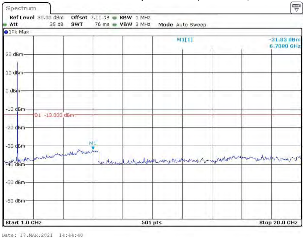
Band 2_1.4 MHz_Low_QPSK_RB6#0_2(1GHz-20GHz)
