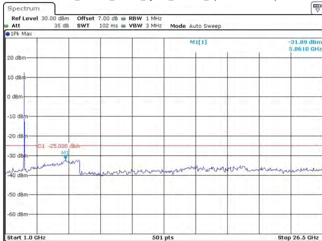
Band 7_10 MHz_Middle_QPSK_RB50#0_2(1GHz-26.5GHz)
