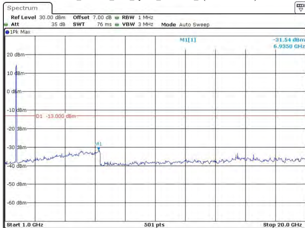
Band 4_20 MHz_Low_QPSK_RB100#0_2(1GHz-20GHz)
