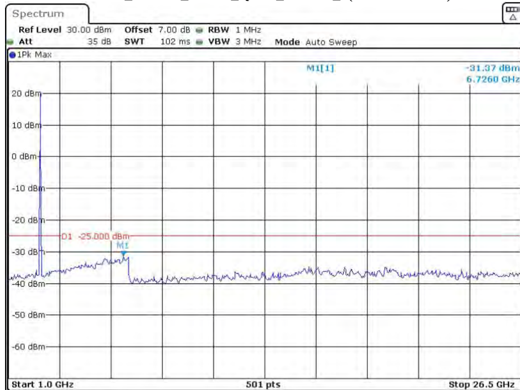
Band 38_15 MHz_Middle_QPSK_RB75#0_2(1GHz-26.5GHz)
