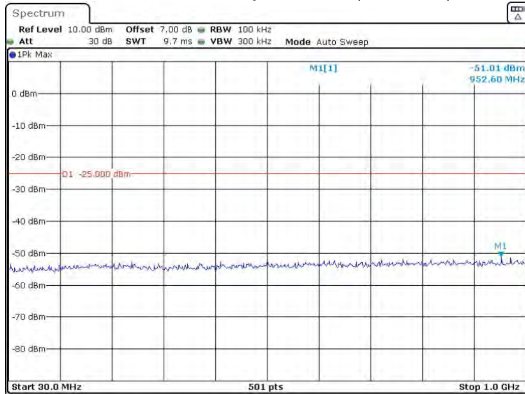
Band 38_10 MHz_Middle_QPSK_RB50#0_1(30MHz-1GHz)
