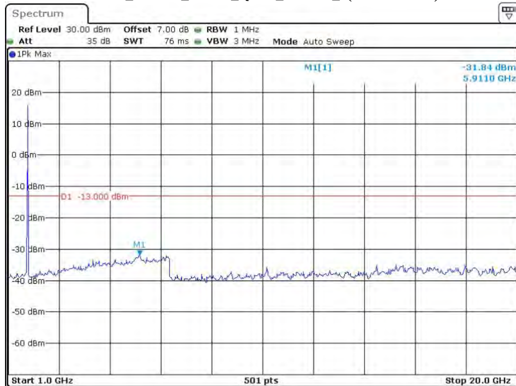
Band 4_10 MHz_Middle_QPSK_RB50#0_2(1GHz-20GHz)
