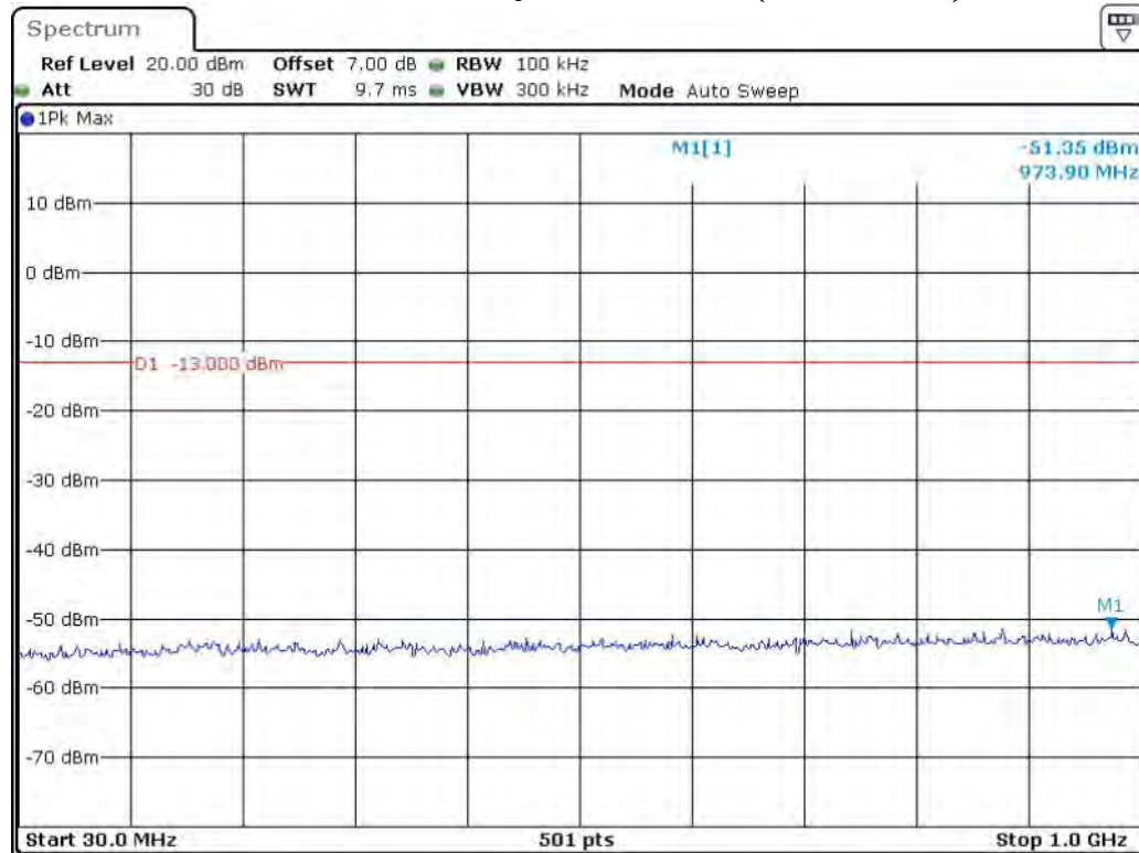
Band 4_20 MHz_Low_QPSK_RB100#0_1(30MHz-1GHz)
