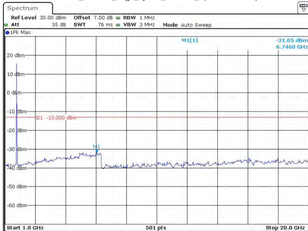
Band 4_10 MHz_High_QPSK_RB50#0_2(1GHz-20GHz)
