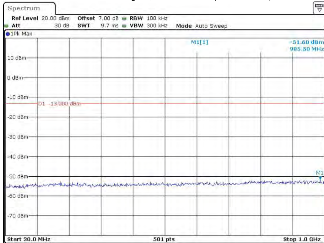
Band 4_10 MHz_High_QPSK_RB50#0_1(30MHz-1GHz)
