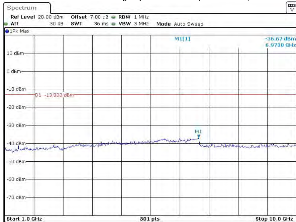
Band 17_10 MHz_High_QPSK_RB50#0_2(1GHz-10GHz)
