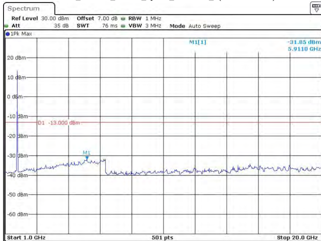
Band 4_20 MHz_Middle_QPSK_RB100#0_2(1GHz-20GHz)
