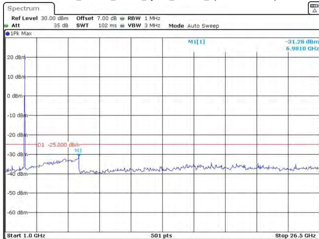
Band 38_10 MHz_Middle_QPSK_RB50#0_2(1GHz-26.5GHz)
