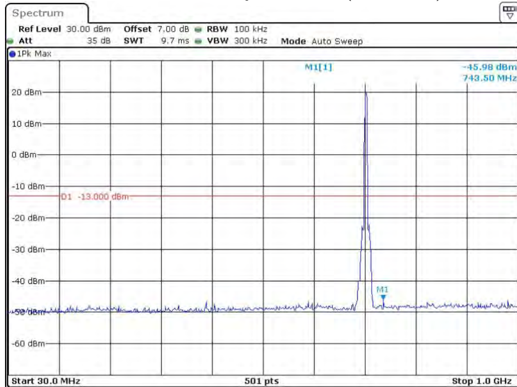
Band 17_5 MHz_Middle_QPSK_RB25#0_1(30MHz-1GHz)
