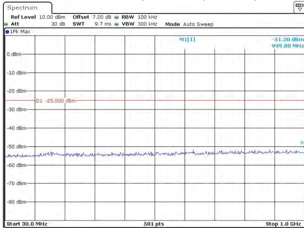
Band 7_5 MHz_Middle_QPSK_RB25#0_1(30MHz-1GHz)
