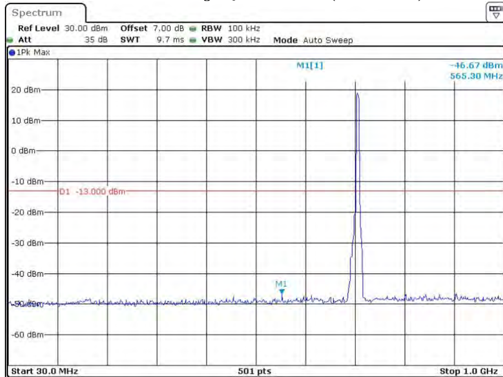
Band 17_5 MHz_High_QPSK_RB25#0_1(30MHz-1GHz)
