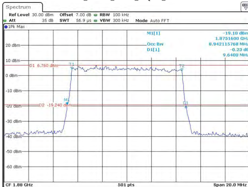
Band 2_10 MHz_Middle_16QAM_RB50#0
