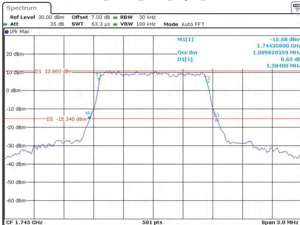
Band 66_1.4 MHz_Middle_16QAM_RB6#0
