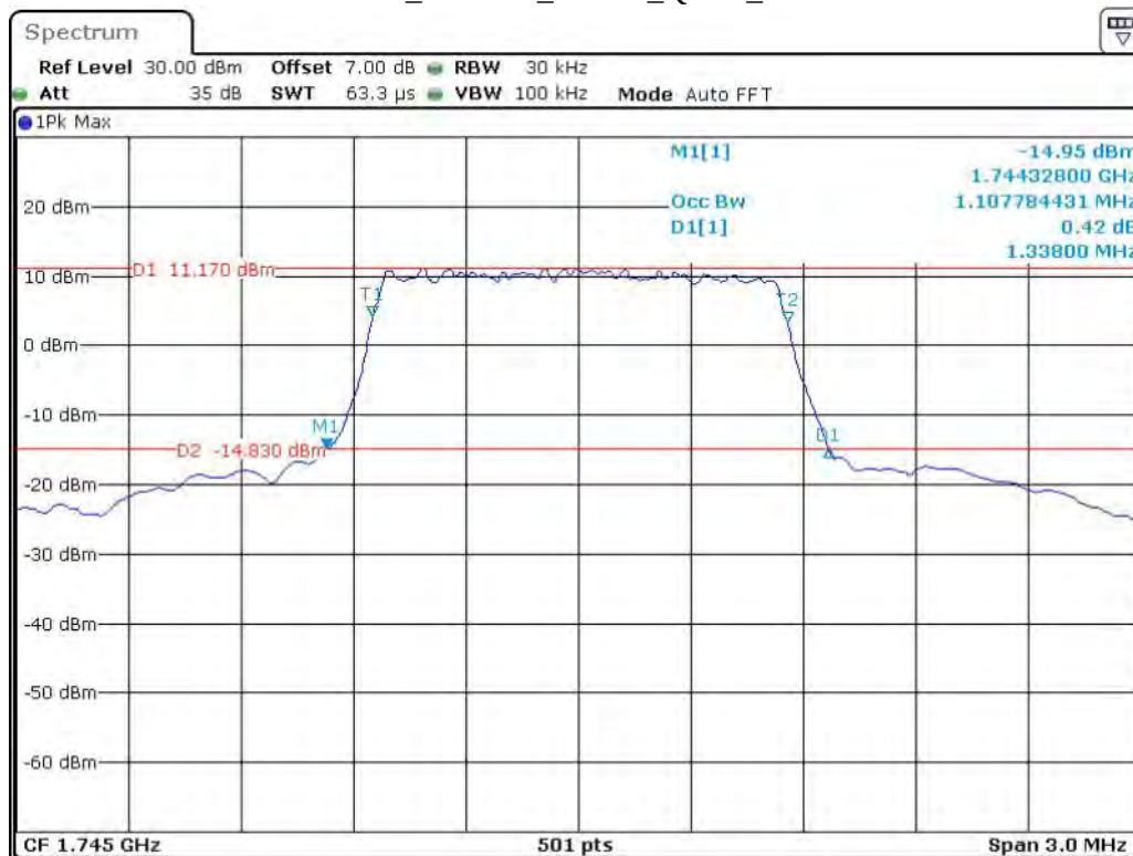
Band 66_1.4 MHz_Middle_QPSK_RB6#0
