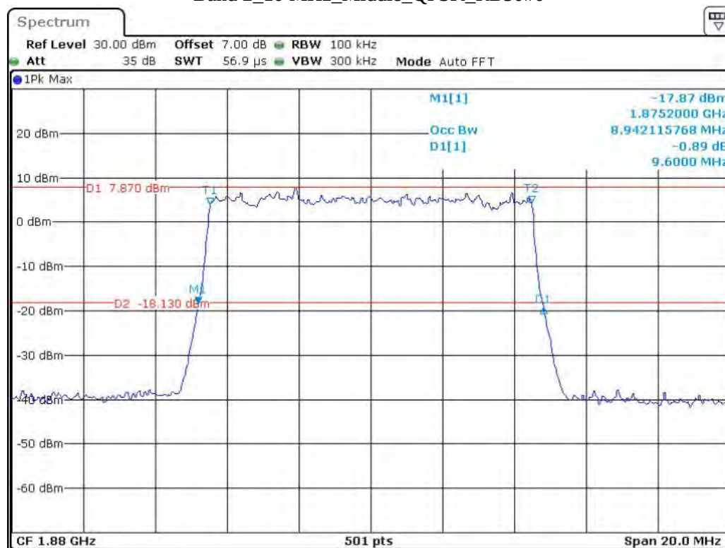
Band 2_10 MHz_Middle_QPSK_RB50#0
