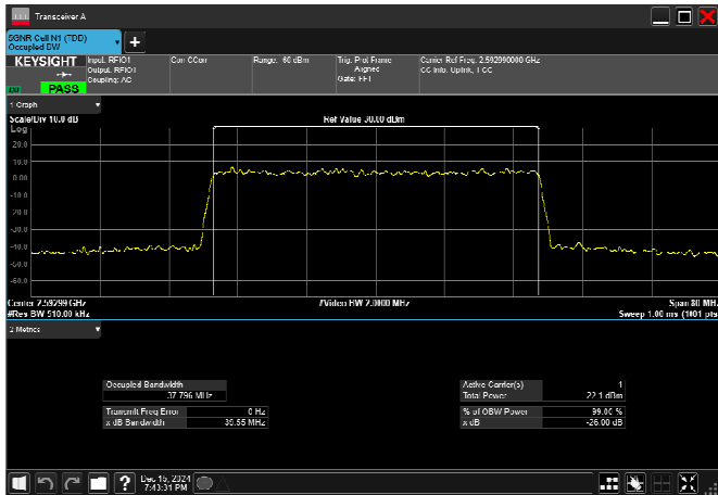
n41_40MHz_30kHz_2592.99MHz_CP-OFDM 256 QAM_RB106@0
