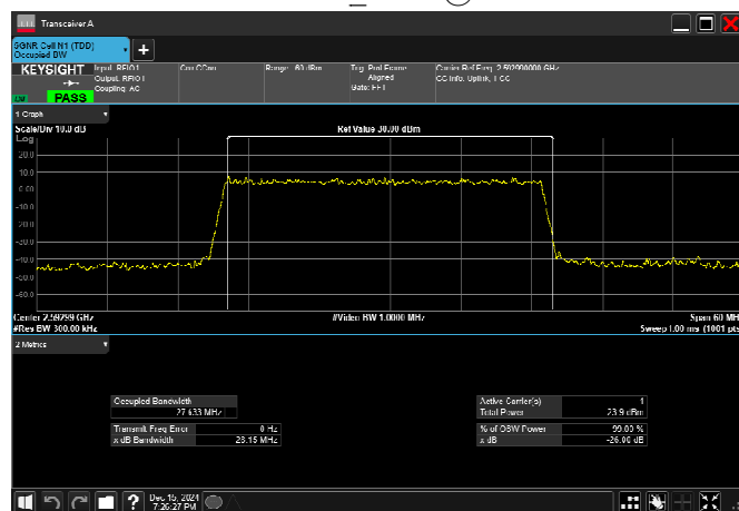
n41_30MHz_30kHz_2592.99MHz_DFT-s-OFDM 16 QAM RB75@0
