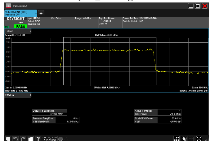
n41_50MHz_30kHz_2592.99MHz_DFT-s-OFDM 16 QAM_RB128@0
