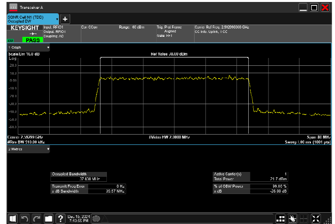
n41_50MHz_30kHz_2592.99MHz_DFT-s-OFDM \pi/2 BPSK_RB128@0
