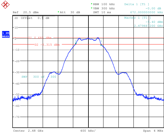
BLE_1M_High_Channel
