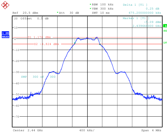
BLE_1M_Middle_Channel
