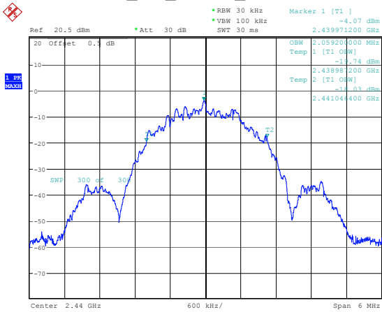
BLE_2M_Middle_Channel
