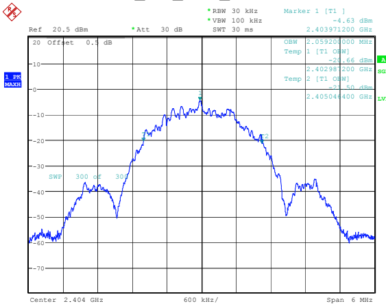
BLE_2M_Low_Channel
