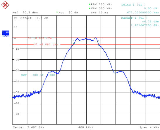
BLE_1M_Low_Channel
