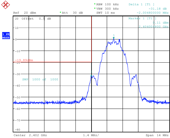
BLE_2M_Low_Channel
