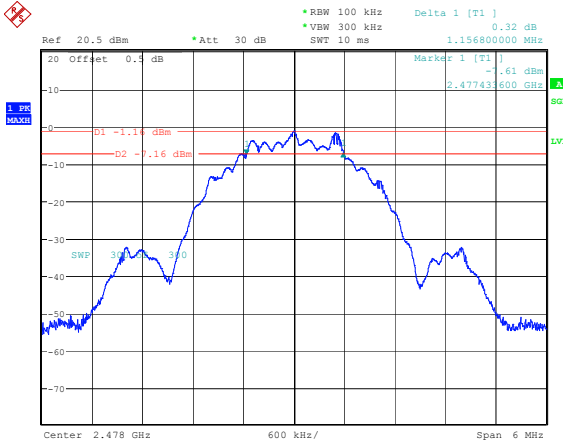
BLE_2M_High_Channel
