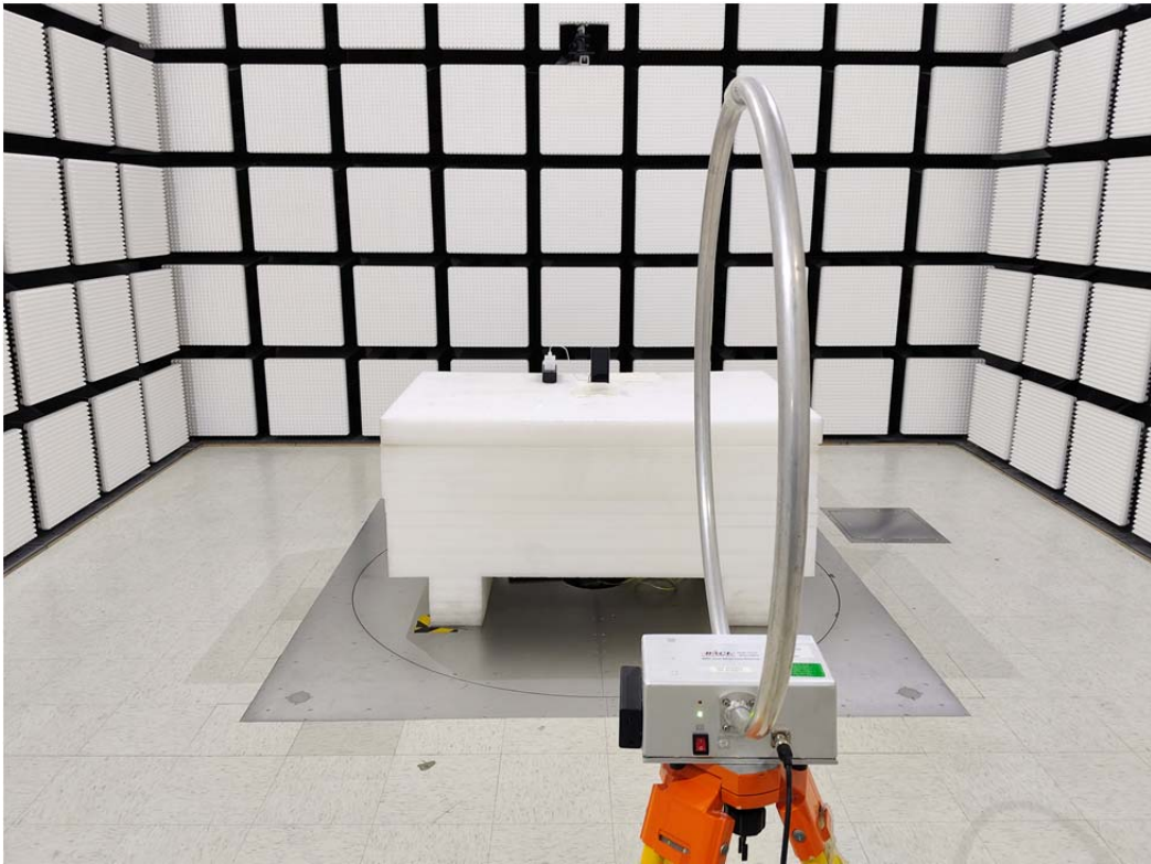
Radiated Emission 9 kHz-30 MHz Perpendicular View
