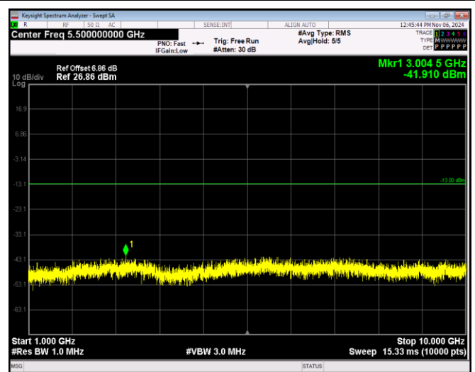
Band17-10MHz-64QAM-23800-1RB#0-Range2:1000~10000MHz
