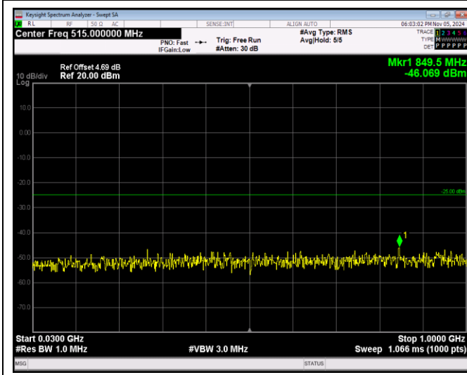
Band41-5MHz-16QAM-40065-1RB#0-Range1:30~100 OMHz
