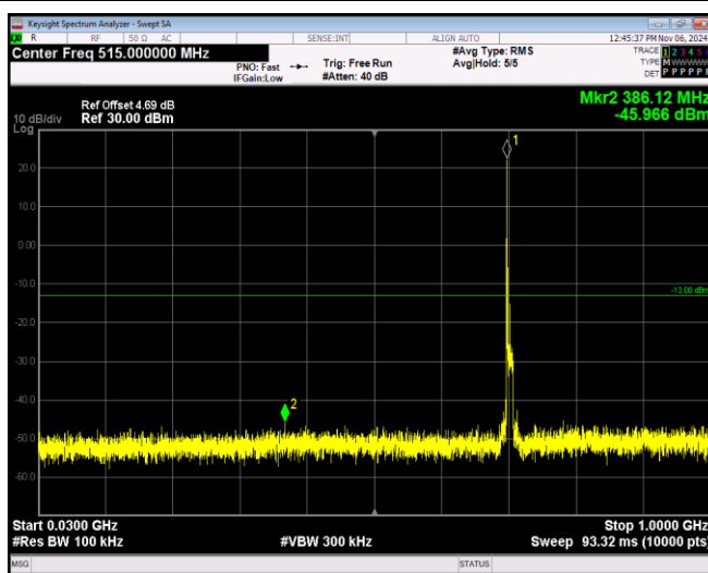
Band17-10MHz-64QAM-23800-1RB#0-Range1:30~1000MHz
