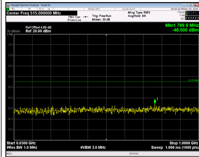
Band41-5MHz-16QAM-40065-1RB#0-Range1:30~100 OMHz
