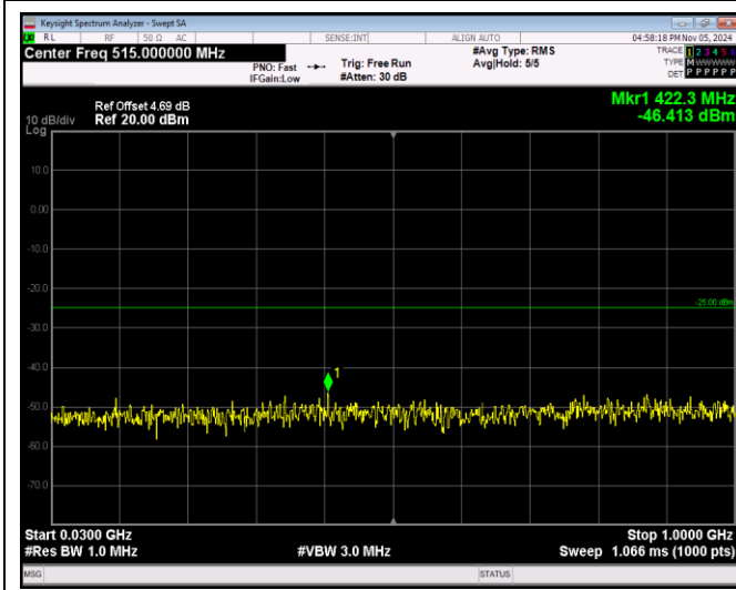
Band38-5MHz-64QAM-37775-1RB#0-Range1:30~100 OMHz
