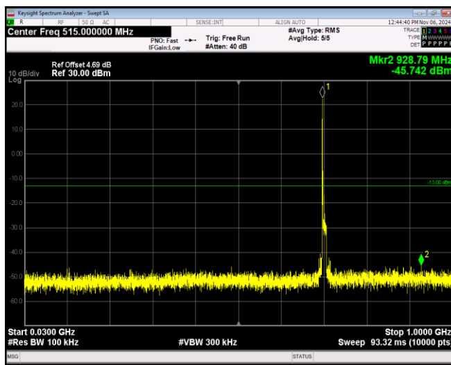
Band17-10MHz-64QAM-23790-1RB#0-Range1:30~1000MHz
