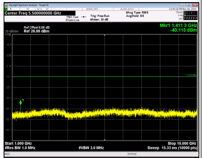
Band17-10MHz-16QAM-23800-1RB#0-Range2:1000~10000MHz
