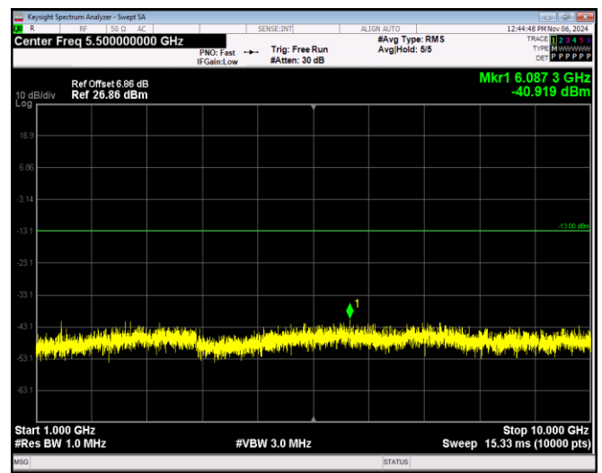
Band17-10MHz-64QAM-23790-1RB#0-Range2:1000~10000MHz
