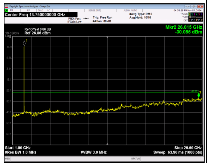
Band38-5MHz-64QAM-37775-1RB#0-Range2:1000~2 6500MHz
