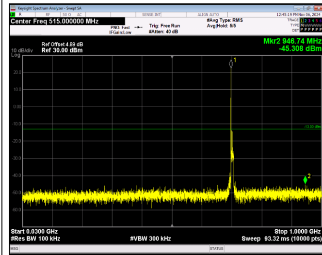
Band17-10MHz-16QAM-23800-1RB#0-Range1:30~1000MHz
