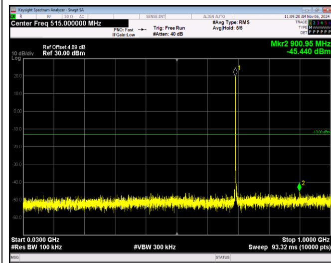
Band12-1.4MHz-64QAM-23095-1RB#0-Range1:30~1000MHz
