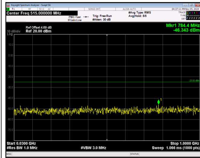
Band7-20MHz-QPSK-21100-1RB#0-Range1:30~1000 MHz
