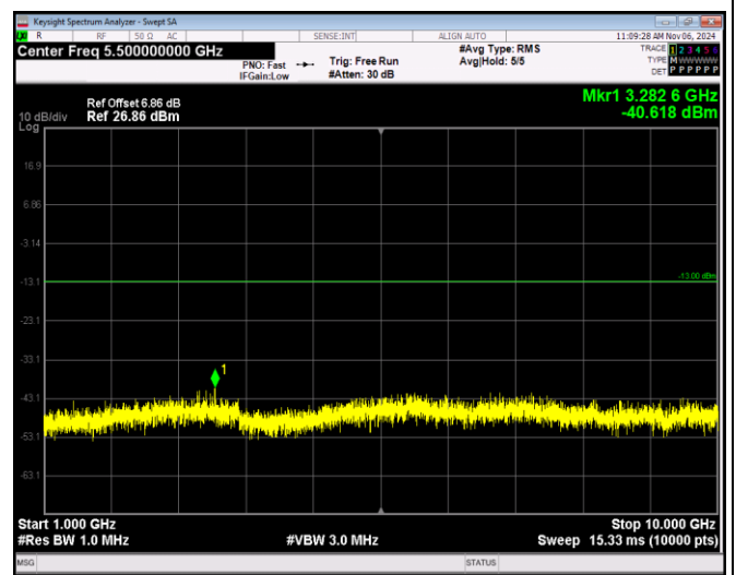
Band12-1.4MHz-64QAM-23095-1RB#0-Range2:1000~10000MHz
