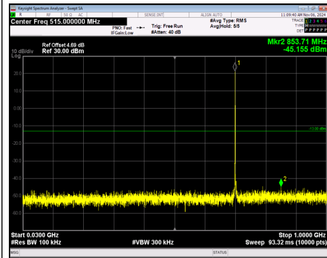
Band12-1.4MHz-QPSK-23173-1RB#0-Range1:30~1000MHz
