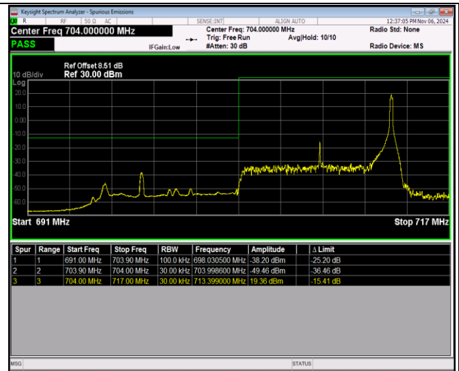
Band17-10MHz-QPSK-23800-1RB#0
