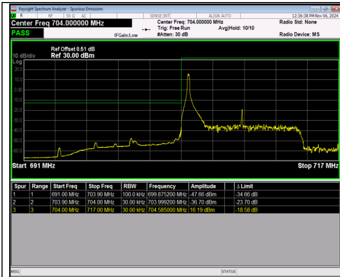
Band17-10MHz-64QAM-23780-50RB#0
