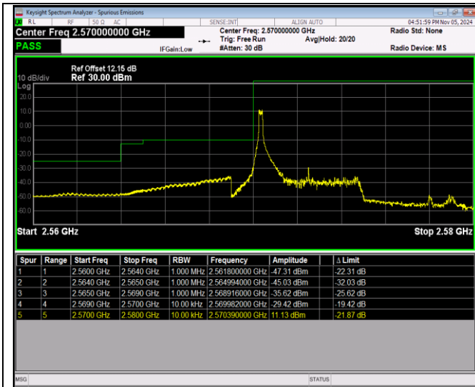
Band38-5MHz-QPSK-37775-25RB#0
