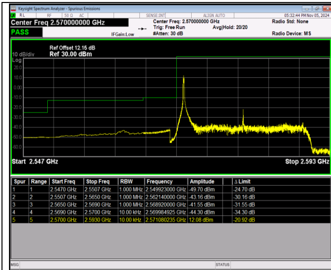
Band38-20MHz-16QAM-37850-100RB#0
