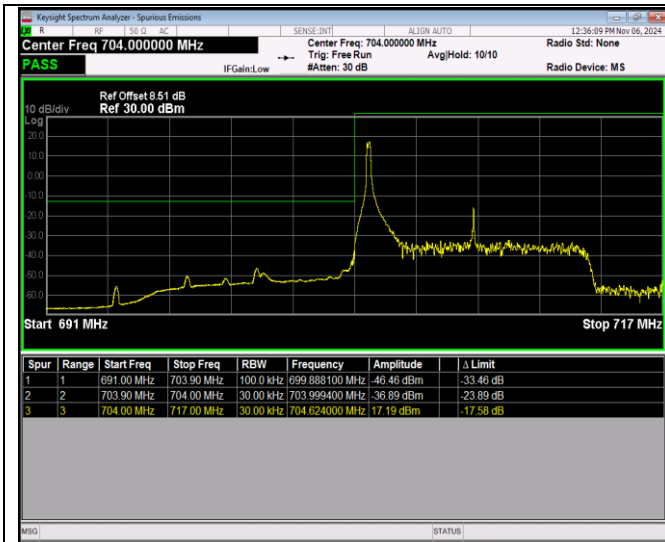
Band17-10MHz-16QAM-23780-50RB#0
