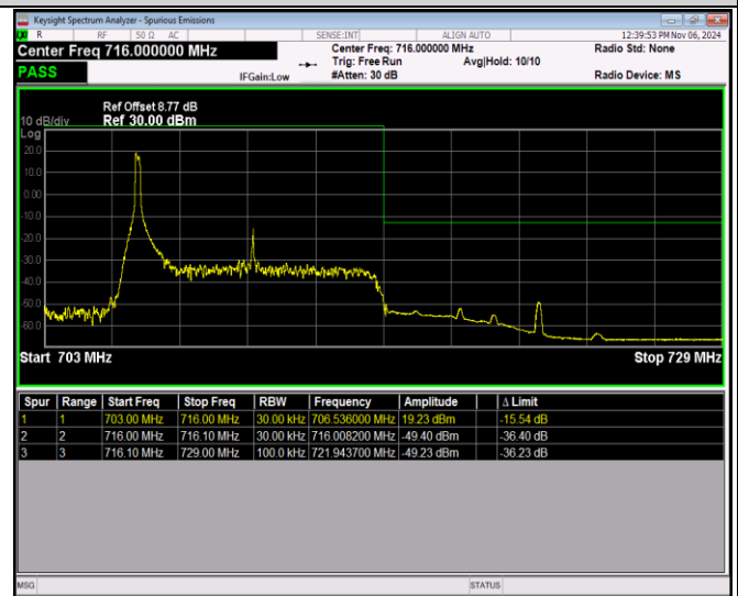
Band17-10MHz-QPSK-23800-50RB#0
