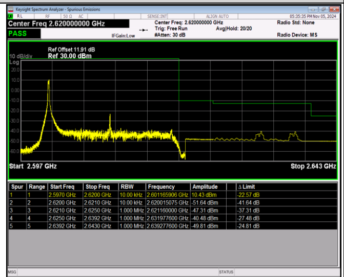
Band38-20MHz-16QAM-38150-100RB#0
