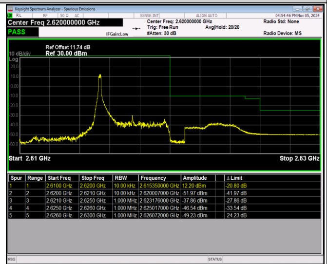
Band38-5MHz-QPSK-38225-25RB#0
