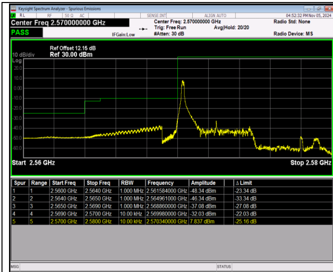
Band38-5MHz-64QAM-37775-25RB#0
