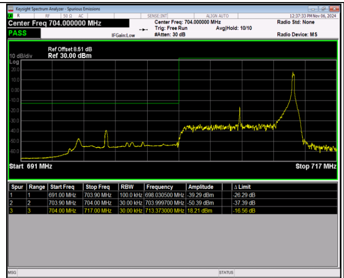
Band17-10MHz-16QAM-23800-1RB#0
