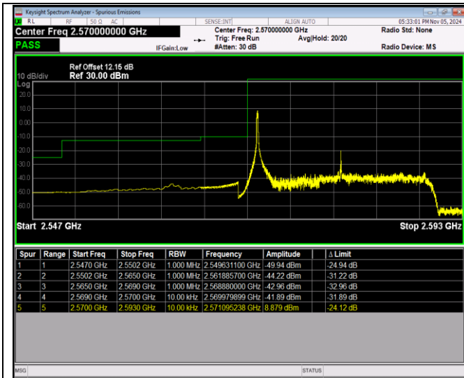
Band38-20MHz-64QAM-37850-100RB#0
