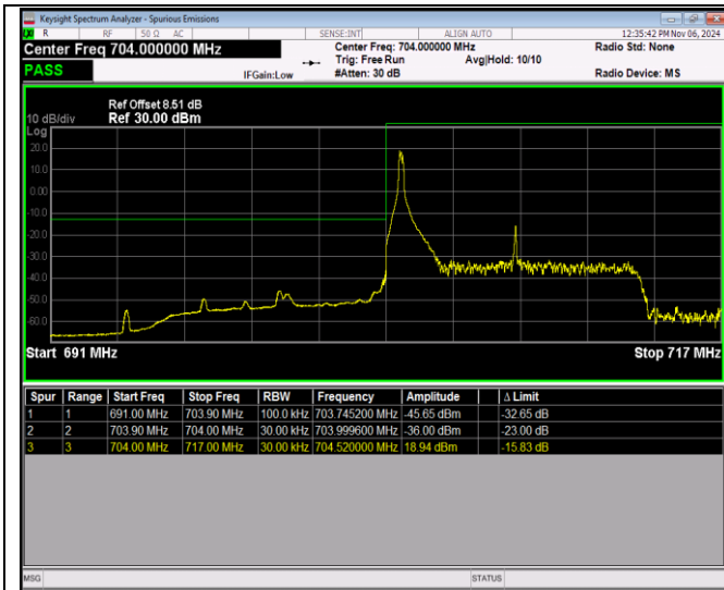
Band17-10MHz-QPSK-23780-50RB#0
