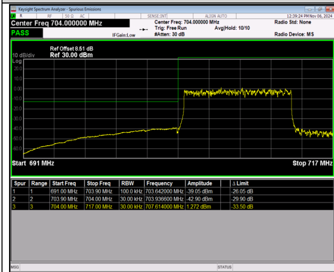
Band17-10MHz-64QAM-23800-1RB#49
