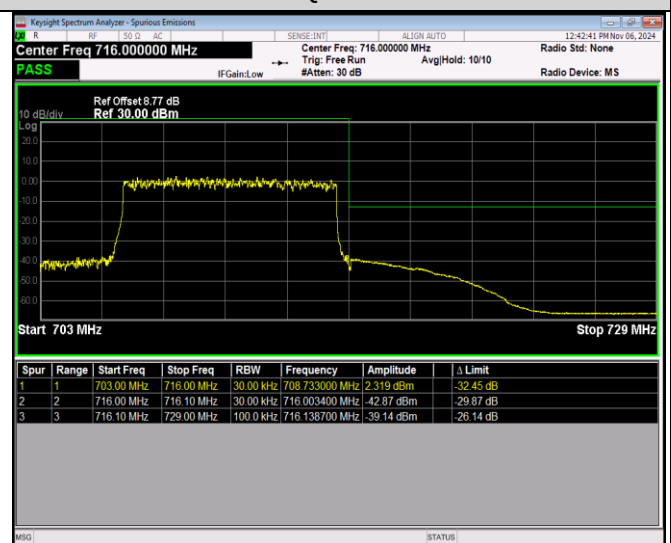
Band17-10MHz-16QAM-23780-1RB#49
