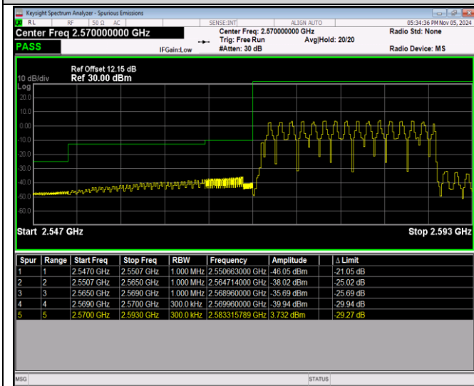
Band38-20MHz-16QAM-38150-1RB#99
