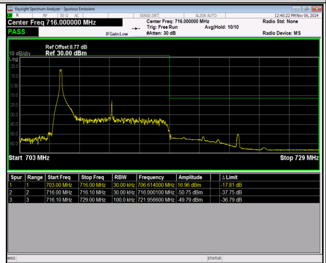
Band17-10MHz-16QAM-23800-50RB#0
