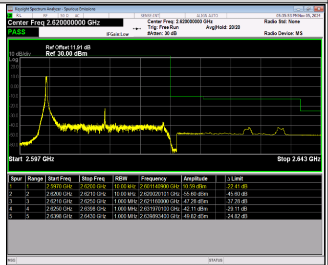
Band38-20MHz-64QAM-38150-100RB#0
