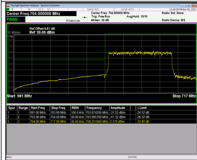
Band17-10MHz-QPSK-23800-1RB#49
