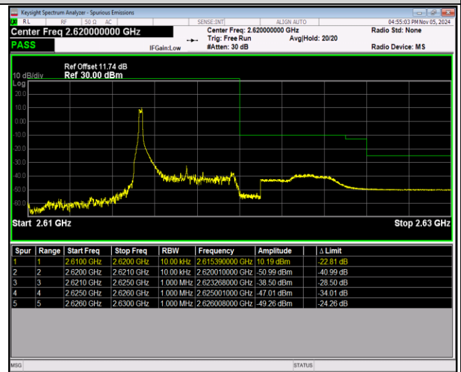
Band38-5MHz-16QAM-38225-25RB#0
