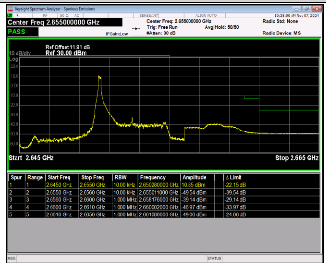
Band41-5MHz-QPSK-41215-25RB#0
