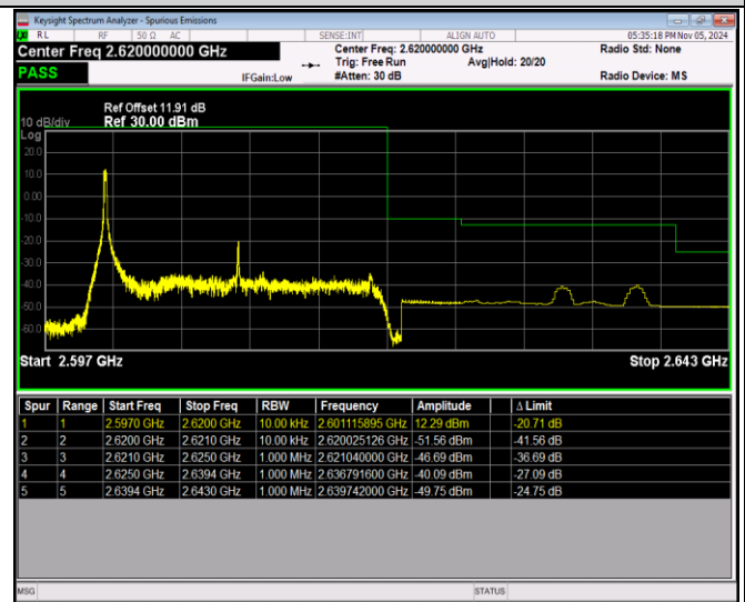
Band38-20MHz-QPSK-38150-100RB#0
