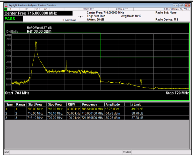
Band17-10MHz-64QAM-23800-50RB#0
