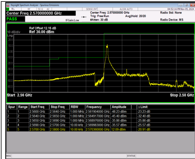
Band38-5MHz-16QAM-37775-25RB#0
