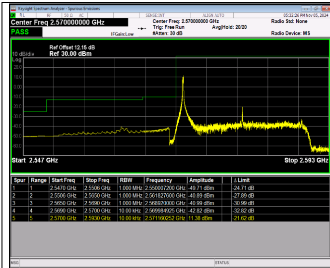
Band38-20MHz-QPSK-37850-100RB#0
