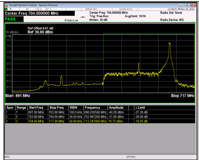
Band17-10MHz-64QAM-23800-1RB#0
