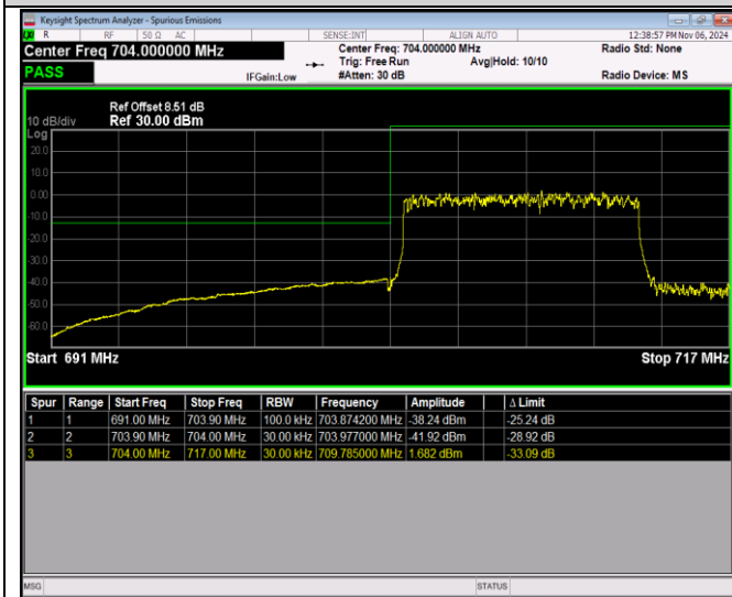
Band17-10MHz-16QAM-23800-1RB#49
