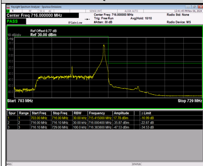
Band17-10MHz-64QAM-23780-1RB#0
