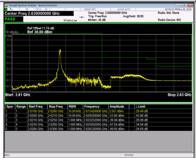
Band38-5MHz-64QAM-38225-25RB#0
