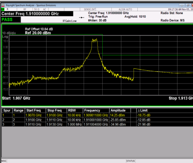
Band2-1.4MHz-QPSK-19193-1RB#5
