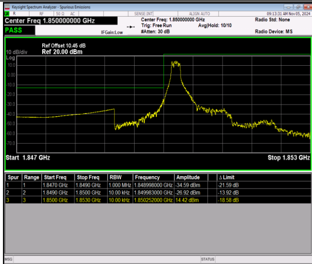
Band2-1.4MHz-QPSK-18607-6RB#0
