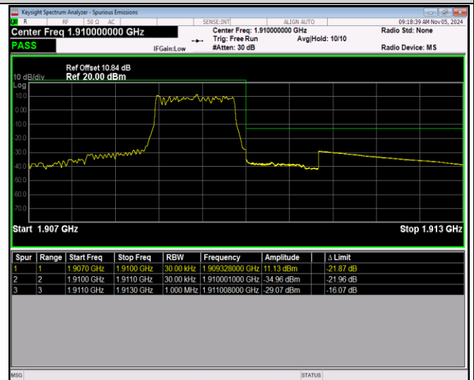
Band2-1.4MHz-QPSK-19193-6RB#0
