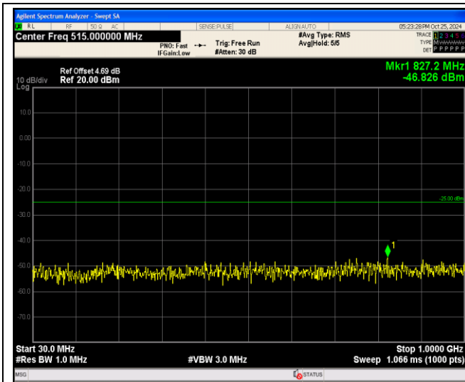
Band41-5MHz-64QAM-40640-1RB#0-Range1:30~1000MHz
