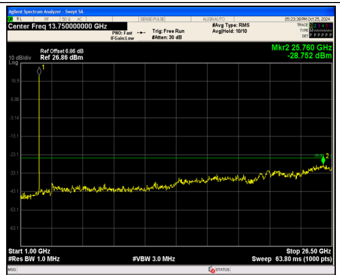
Band41-5MHz-64QAM-40640-1RB#0-Range2:1000~26500MHz
