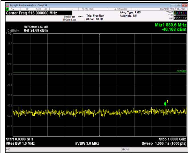
Band66-20MHz-QPSK-132322-1RB#0-Range1:30~1000MHz
