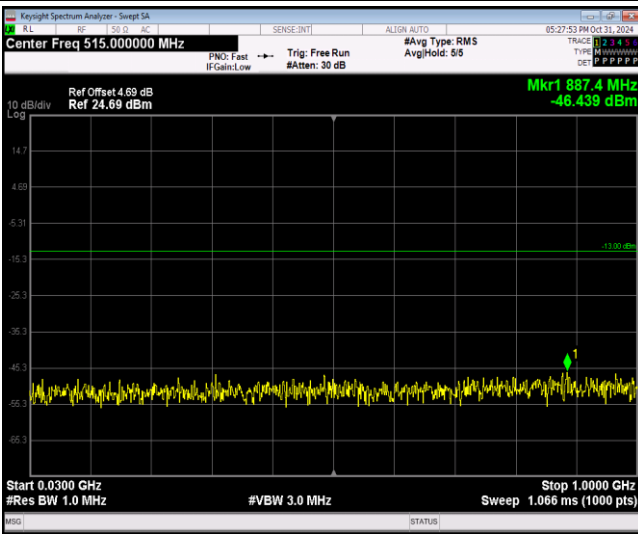
Band66-1.4MHz-QPSK-131979-1RB#0-Range1:30~1 000MHz
