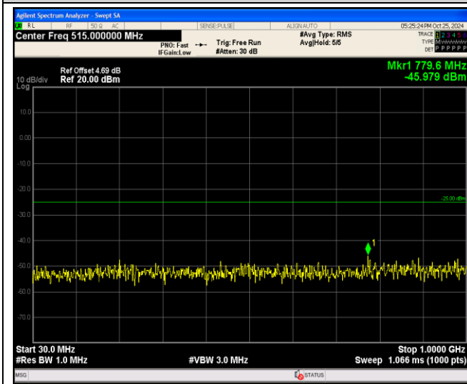
Band41-5MHz-64QAM-41215-1RB#0-Range1:30~1000MHz
