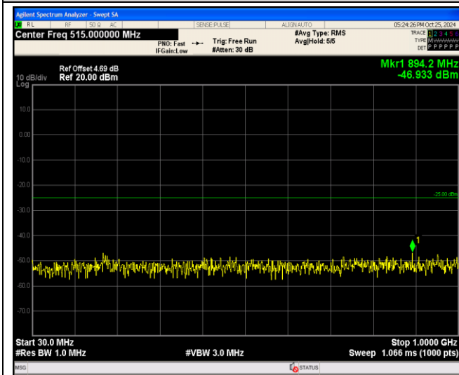
Band41-5MHz-64QAM-41215-1RB#0-Range1:30~1000MHz
