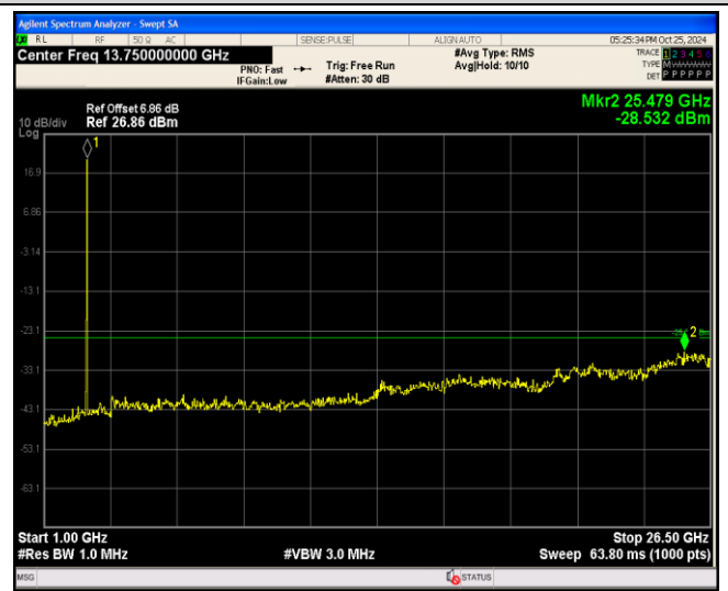
Band41-5MHz-64QAM-41215-1RB#0-Range2:1000~26500MHz
