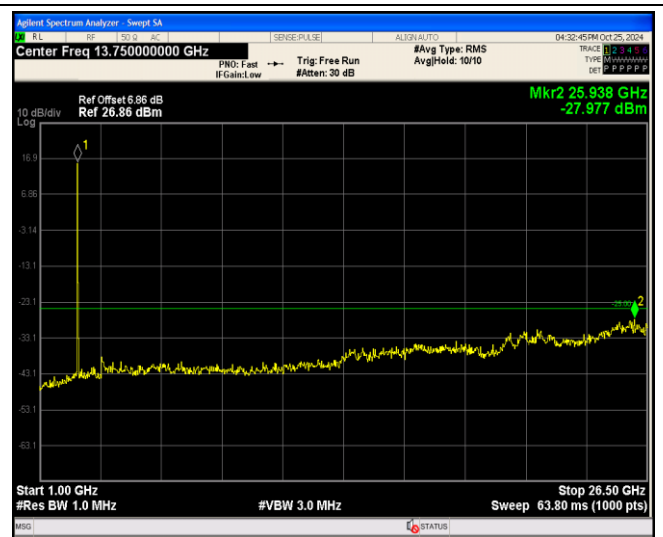
Band38-5MHz-16QAM-38225-1RB#0-Range2:1000~26500MHz
