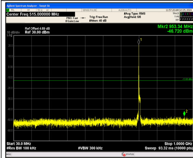
Band12-10MHz-64QAM-23130-1RB#0-Range1:30~1000MHz
