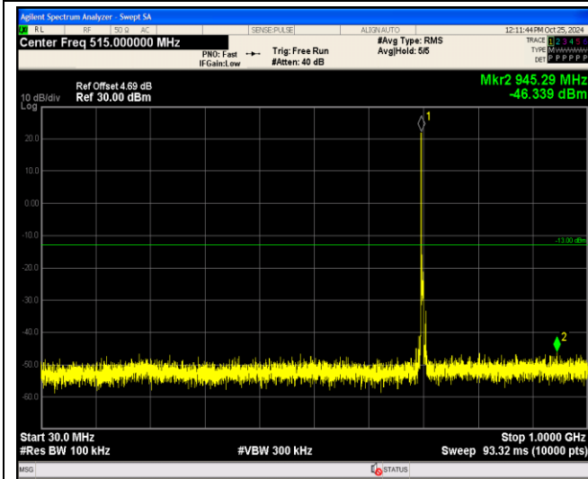
Band17-5MHz-16QAM-23790-1RB#0-Range1:30~1000MHz
