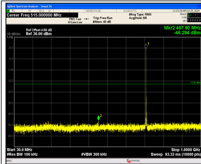
Band12-1.4MHz-64QAM-23017-1RB#0-Range1:30~1 000MHz
