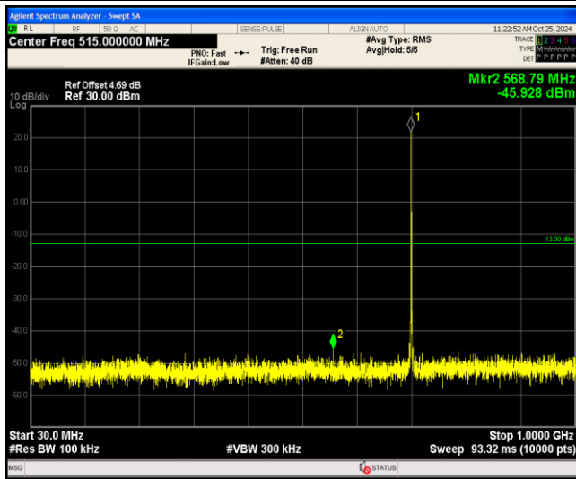
Band12-1.4MHz-64QAM-23095-1RB#0-Range1:30~1 000MHz
