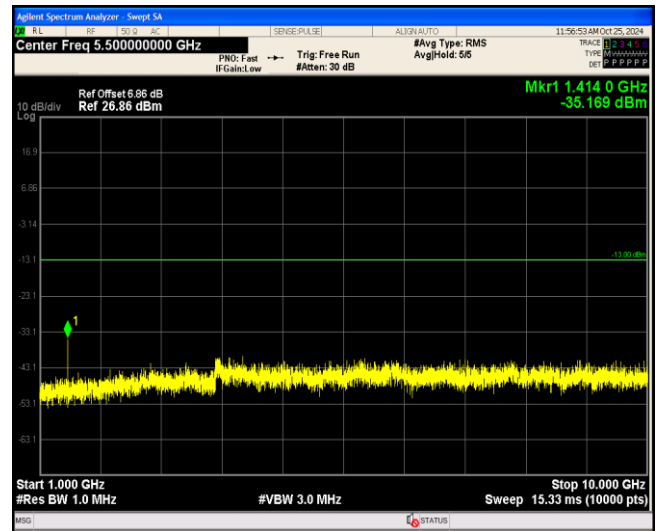
Band12-10MHz-16QAM-23060-1RB#0-Range2:1000~10000MHz
