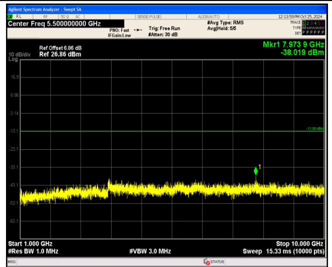
Band17-10MHz-QPSK-23780-1RB#0-Range2:1000~10000MHz
