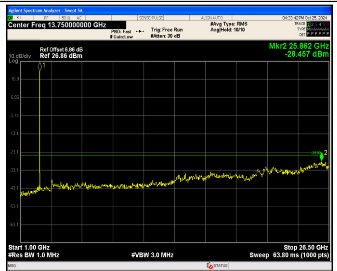
Band38-5MHz-64QAM-37775-1RB#0-Range2:1000~26500MHz
