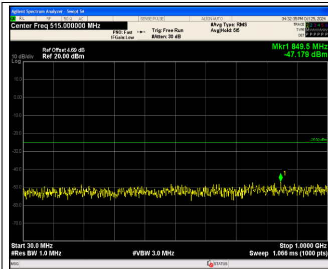
Band38-5MHz-16QAM-38225-1RB#0-Range1:30~1000MHz
