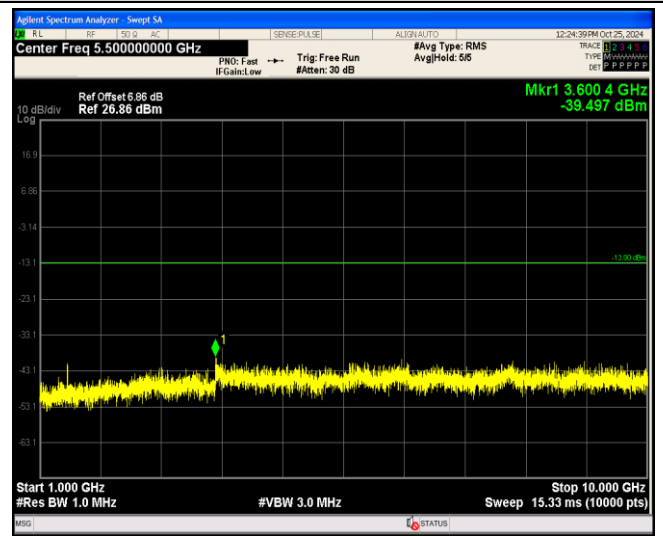
Band17-10MHz-QPSK-23780-1RB#0-Range2:1000~10000MHz
