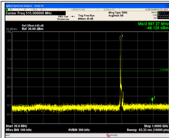
Band12-10MHz-64QAM-23095-1RB#0-Range1:30~1000MHz
