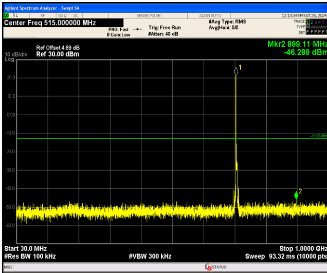
Band17-5MHz-64QAM-23755-1RB#0-Range1:30~1000MHz
