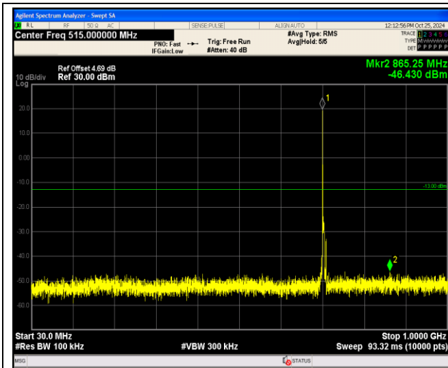
Band17-5MHz-64QAM-23825-1RB#0-Range1:30~1000MHz
