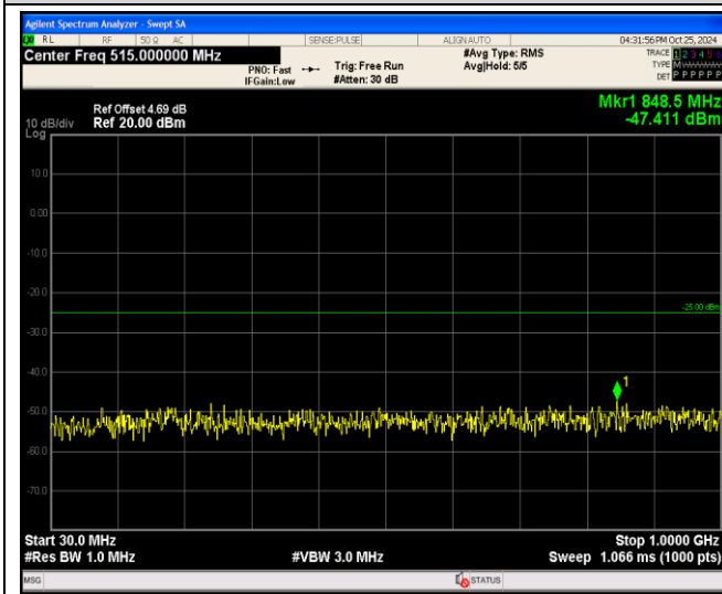
Band38-5MHz-64QAM-37775-1RB#0-Range1:30~1000MHz
