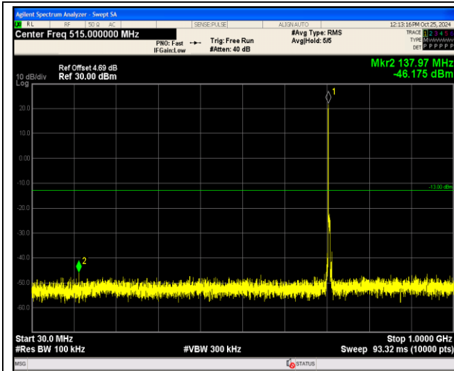
Band17-5MHz-16QAM-23755-1RB#0-Range1:30~1000MHz
