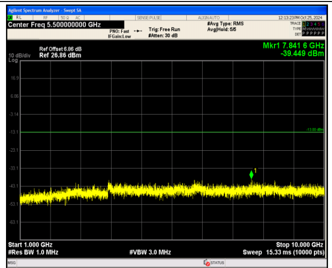
Band17-5MHz-16QAM-23755-1RB#0-Range2:1000~10000MHz
