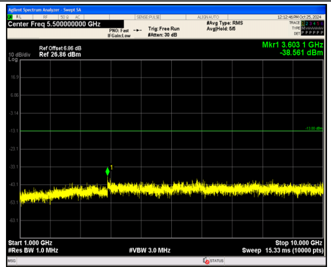
Band17-5MHz-16QAM-23790-1RB#0-Range2:1000~10000MHz
