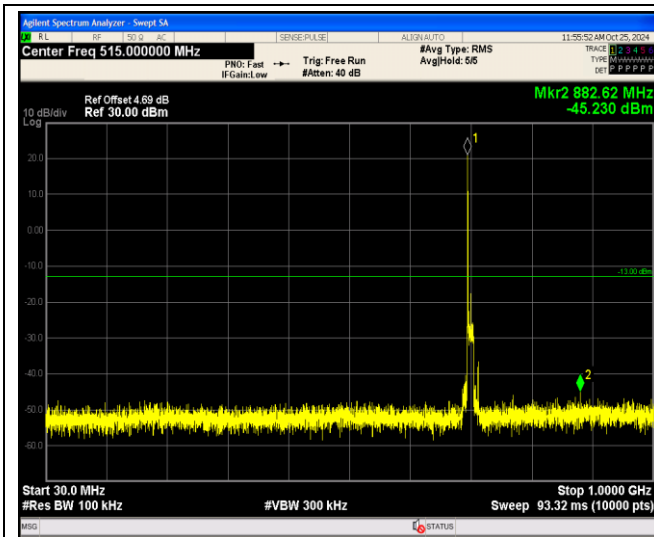
Band12-10MHz-QPSK-23130-1RB#0-Range1:30~1000MHz
