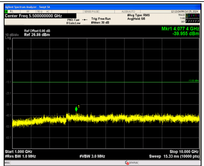
Band17-5MHz-64QAM-23825-1RB#0-Range2:1000~10000MHz
