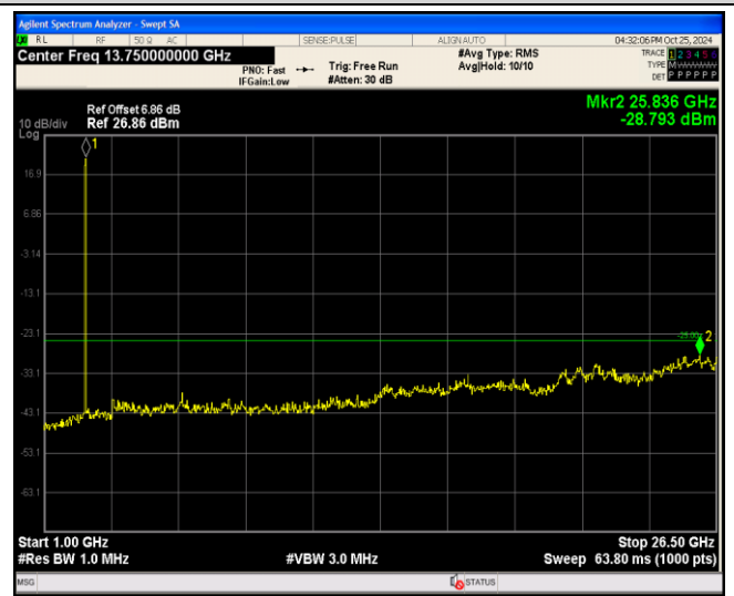
Band38-5MHz-64QAM-37775-1RB#0-Range2:1000~26500MHz
