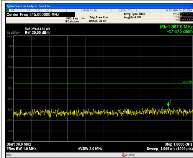
Band38-5MHz-64QAM-37775-1RB#0-Range1:30~1000MHz
