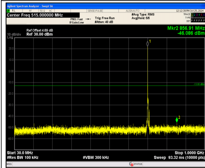
Band17-5MHz-16QAM-23790-1RB#0-Range1:30~1000MHz
