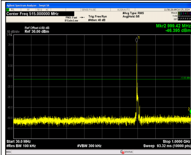
Band12-10MHz-64QAM-23130-1RB#0-Range1:30~1000MHz
