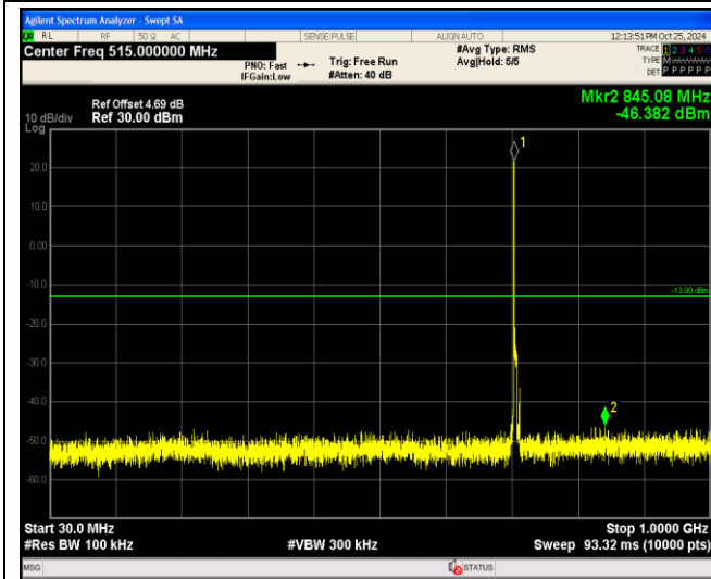
Band17-10MHz-QPSK-23780-1RB#0-Range1:30~1000MHz
