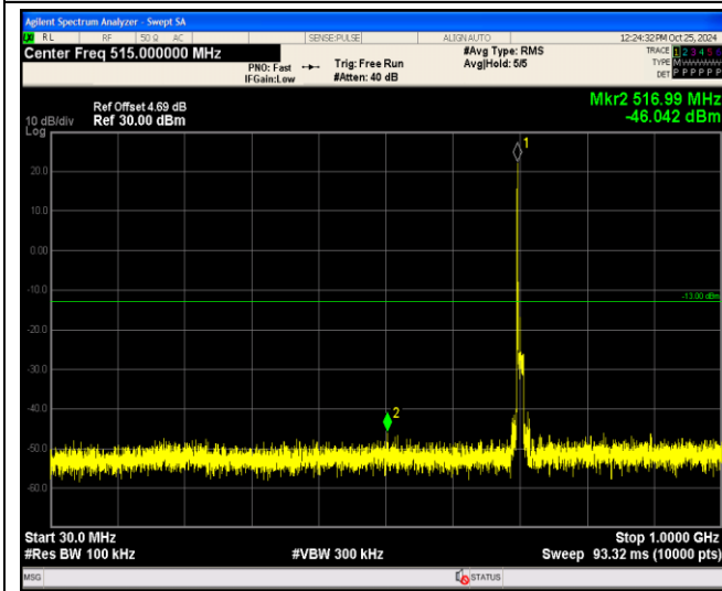
Band17-10MHz-QPSK-23780-1RB#0-Range1:30~1000MHz
