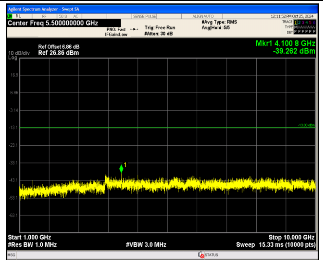
Band17-5MHz-16QAM-23790-1RB#0-Range2:1000~10000MHz
