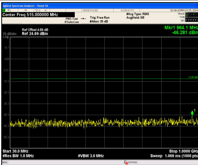
Band2-20MHz-64QAM-19100-1RB#0-Range1:30~1000MHz
