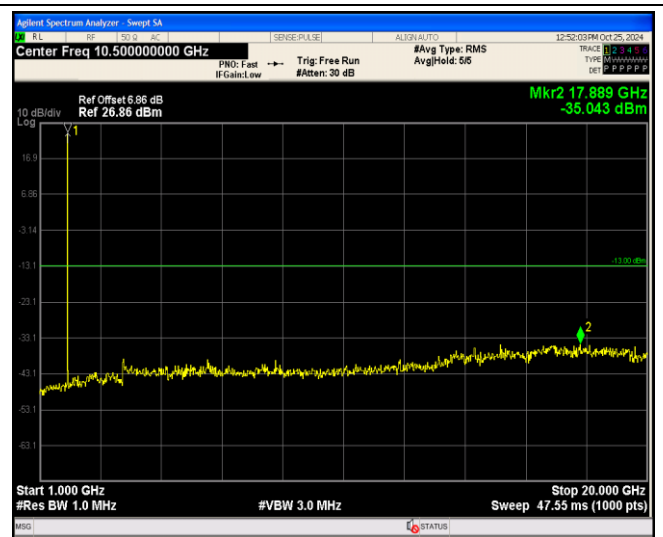
Band2-1.4MHz-64QAM-19193-1RB#0-Range2:1000~20000MHz
