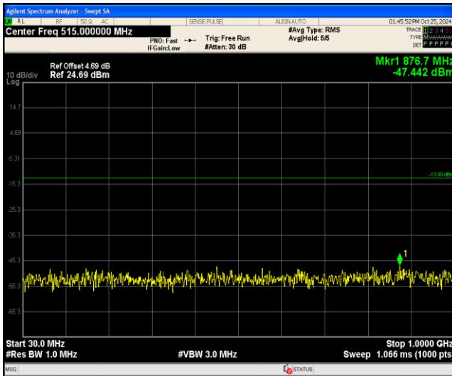
Band2-20MHz-64QAM-18900-1RB#0-Range1:30~1000MHz
