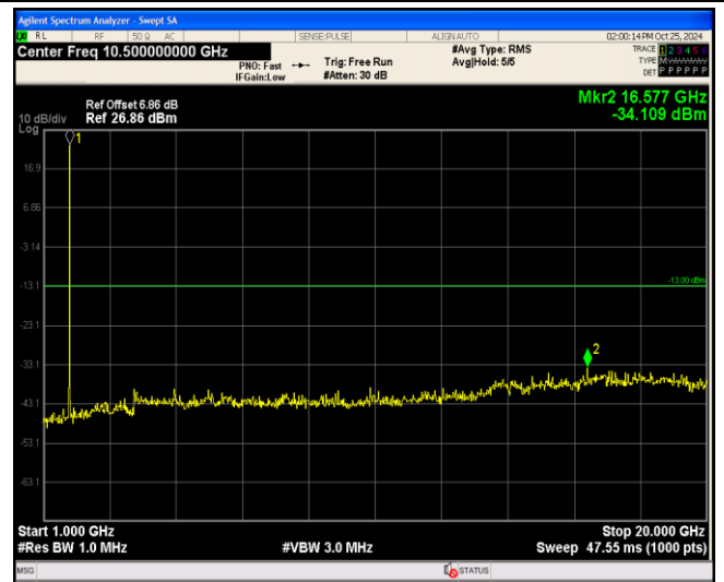
Band4-1.4MHz-64QAM-19957-1RB#0-Range2:1000~20000MHz
