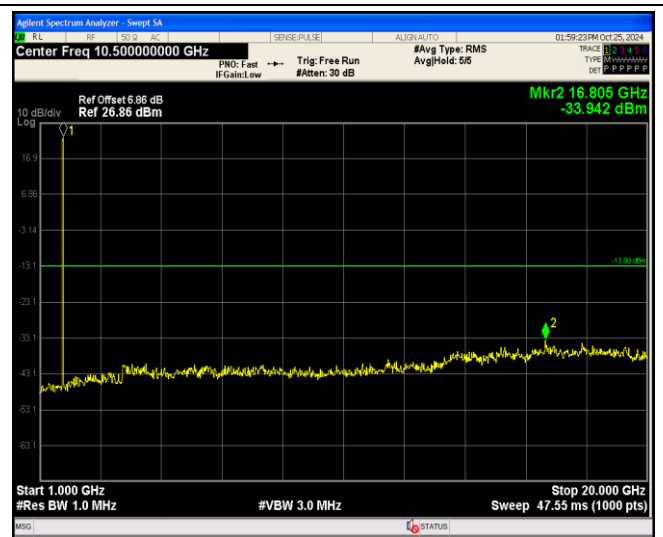
Band4-1.4MHz-16QAM-20393-1RB#0-Range2:1000~20000MHz
