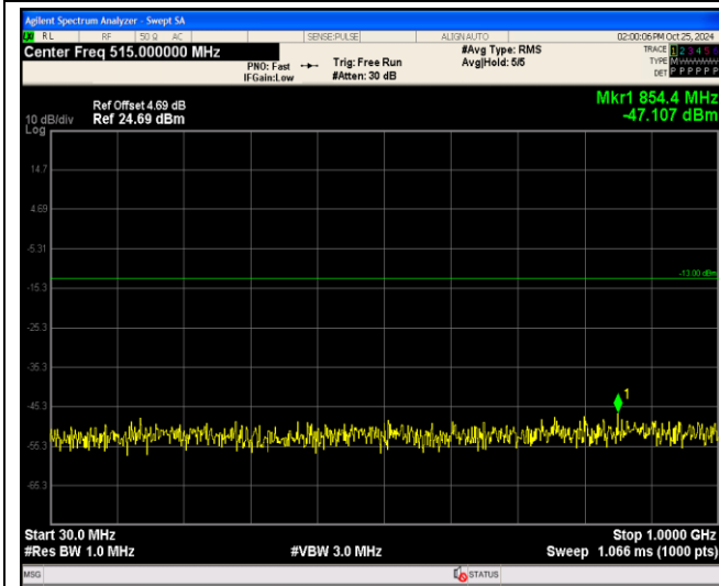
Band4-1.4MHz-64QAM-19957-1RB#0-Range1:30~1000MHz
