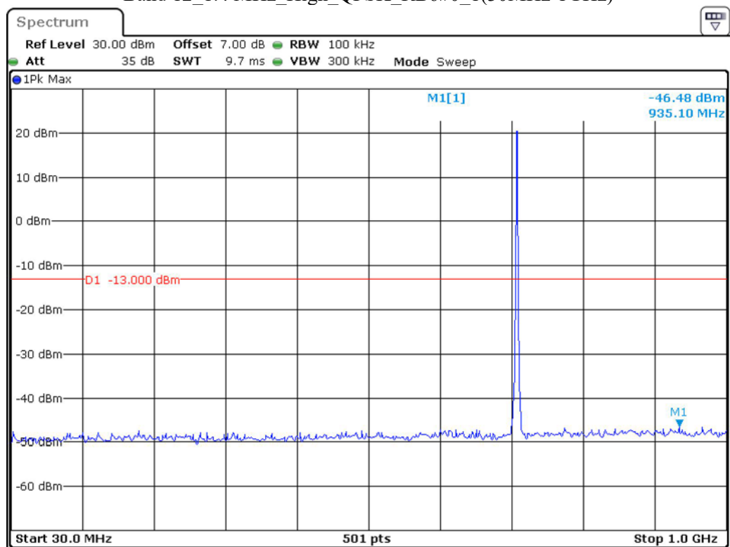
Band 12_1.4 MHz_High_QPSK_RB6#0_1(30MHz-1GHz)
