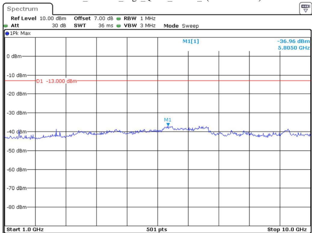
Band 12 1.4 MHz High QPSK RB6#0 2(1GHz-10GHz)
