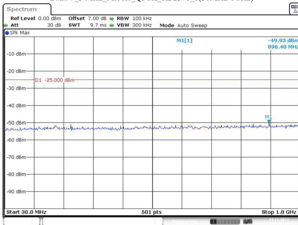
Band 7_5 MHz_Middle_QPSK_RB25#0_1(30MHz-1GHz)
