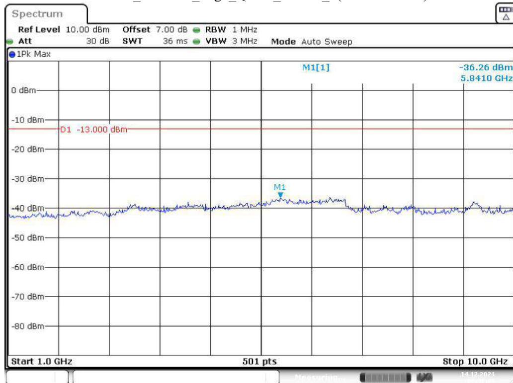
Band 5_1.4 MHz_High_QPSK_RB6#0_2(1GHz-10GHz)
