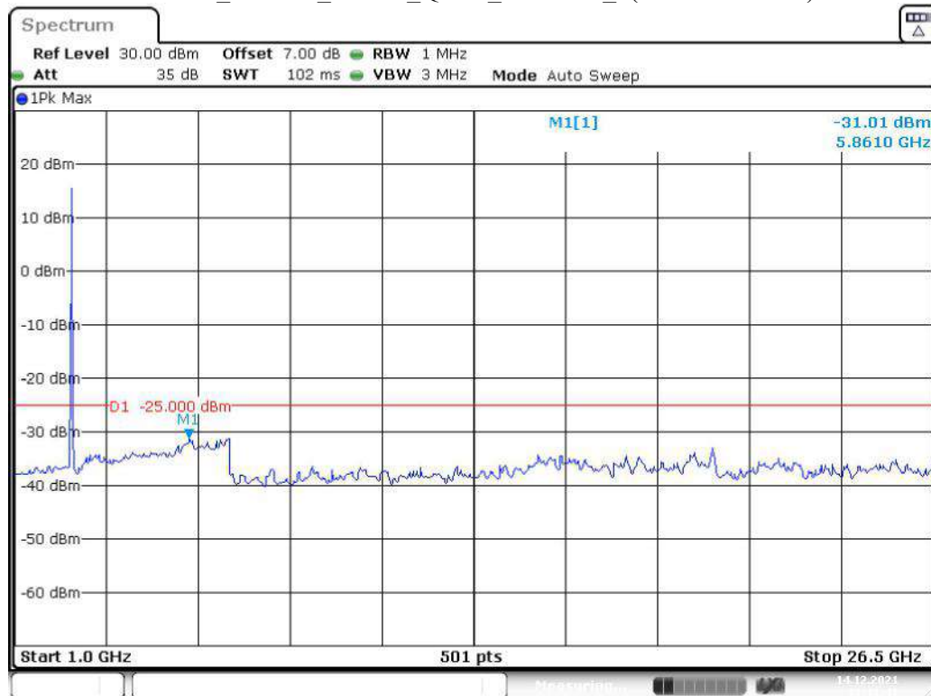
Band 41_20 MHz_Middle_QPSK_RB100#0_2(1GHz-26.5GHz)
