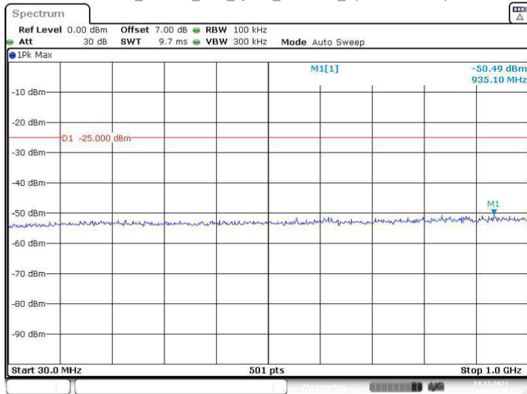
Band 38_20 MHz_Low_QPSK_RB100#0_1(30MHz-1GHz)
