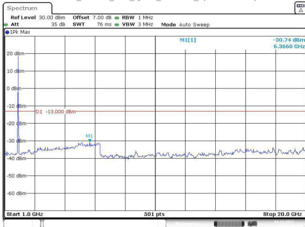
Band 2_20 MHz_Low_QPSK_RB100#0_2(1GHz-20GHz)
