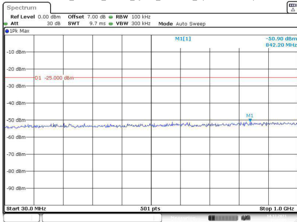
Band 7_20 MHz_Middle_QPSK_RB100#0_1(30MHz-1GHz)
