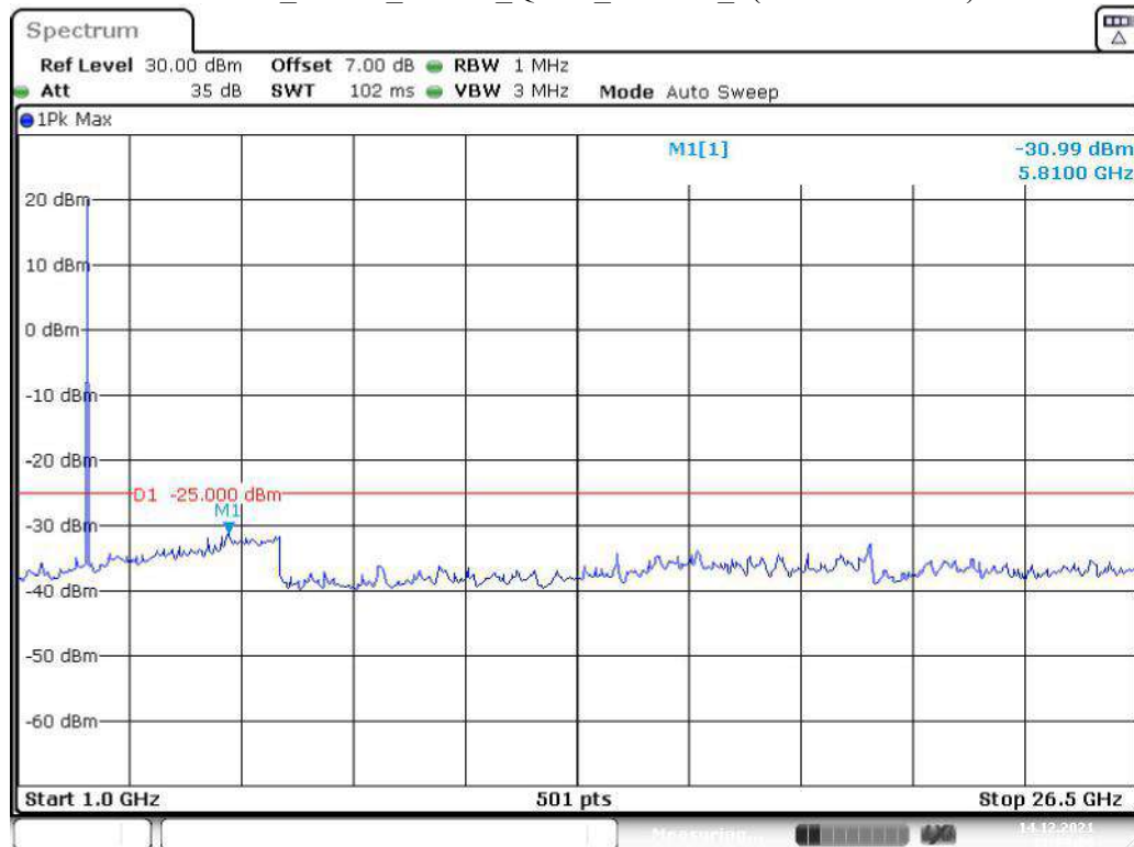
Band 41_5 MHz_Middle_QPSK_RB25#0_2(1GHz-26.5GHz)
