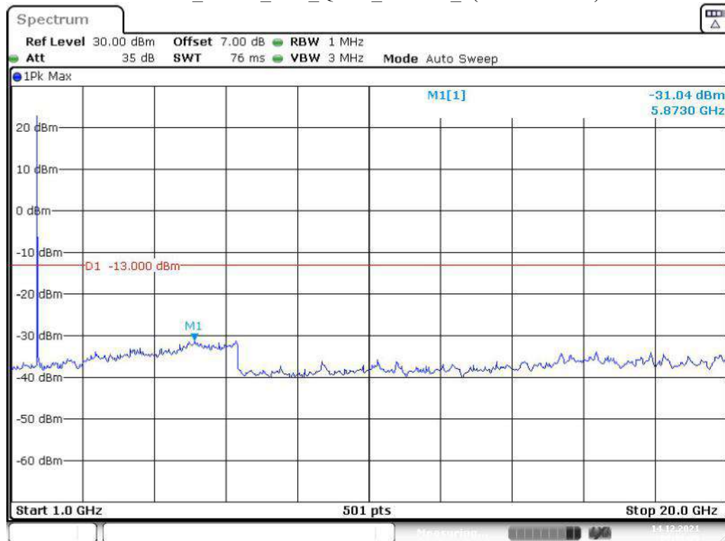
Band 4_3 MHz_Low_QPSK_RB15#0_2(1GHz-20GHz)
