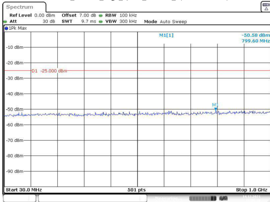
Band 41_10 MHz_High_QPSK_RB50#0_1(30MHz-1GHz)
