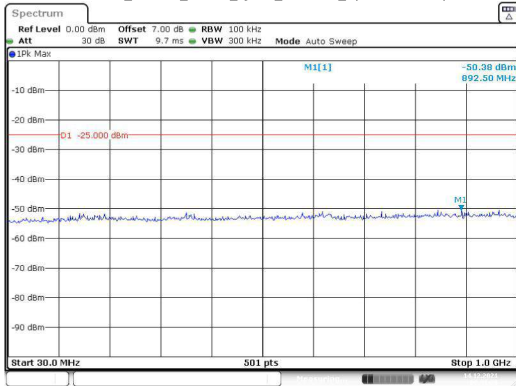
Band 38_20 MHz_Middle_QPSK_RB100#0_1(30MHz-1GHz)
