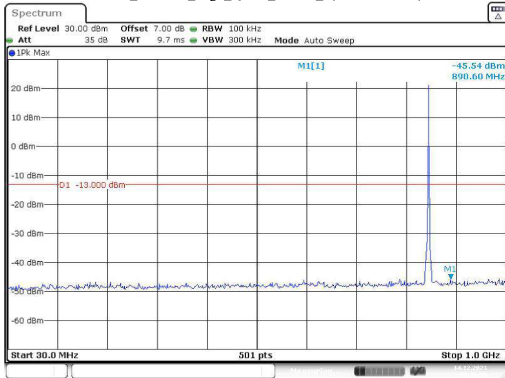
Band 5_1.4 MHz_High_QPSK_RB6#0_1(30MHz-1GHz)
