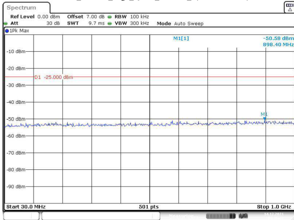
Band 38_10 MHz_High_QPSK_RB50#0_1(30MHz-1GHz)
