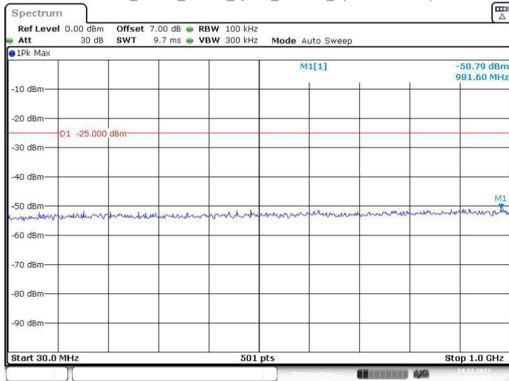
Band 38_5 MHz_Middle_QPSK_RB25#0_1(30MHz-1GHz)
