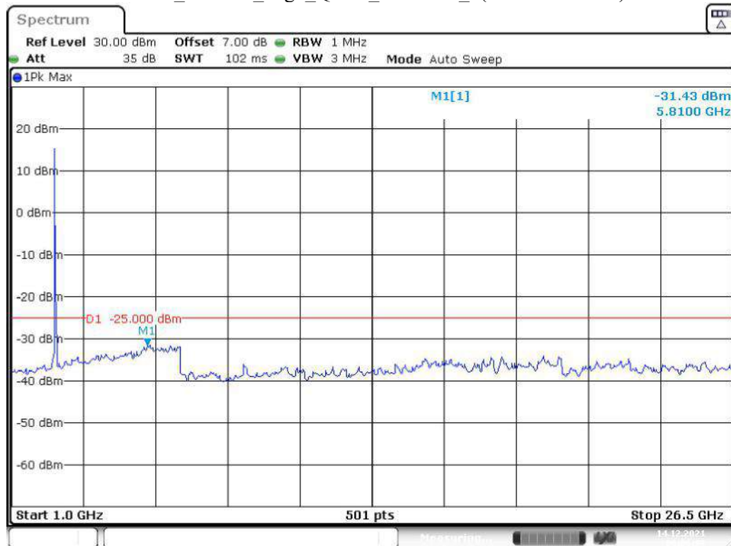
Band 7_20 MHz_High_QPSK_RB100#0_2(1GHz-26.5GHz)
