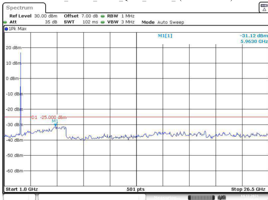
Band 41_15 MHz_Middle_QPSK_RB75#0_2(1GHz-26.5GHz)
