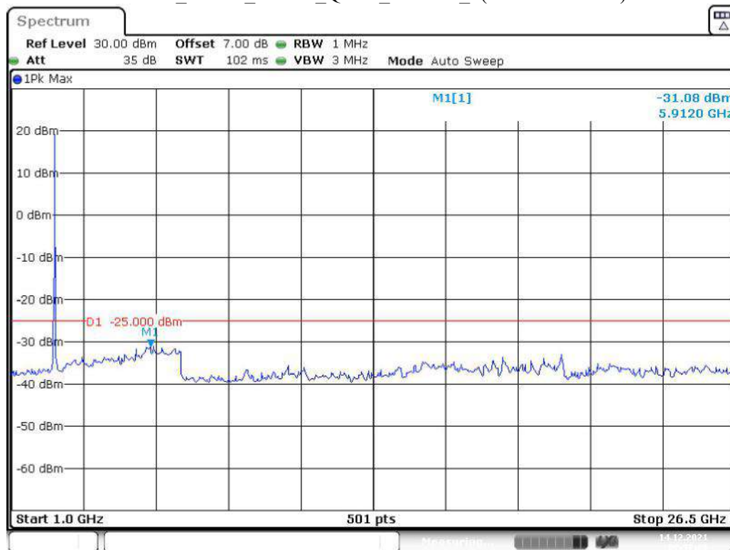
Band 7_5 MHz_Middle_QPSK_RB25#0_2(1GHz-26.5GHz)
