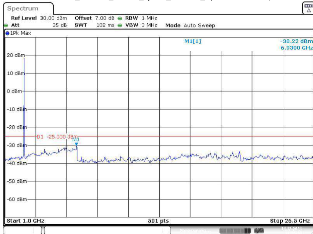
Band 41_10 MHz_Middle_QPSK_RB50#0_2(1GHz-26.5GHz)
