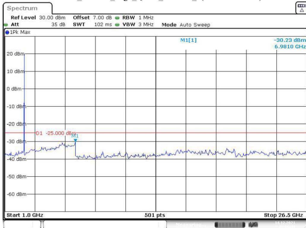
Band 41_10 MHz_High_QPSK_RB50#0_2(1GHz-26.5GHz)
