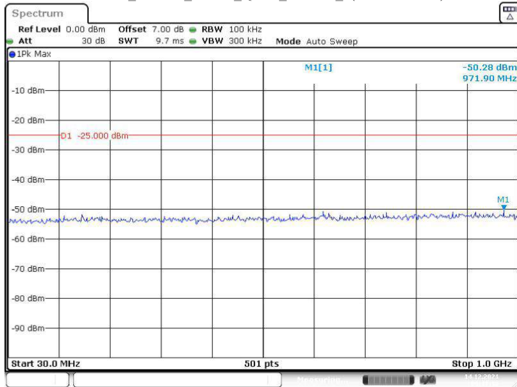
Band 38_15 MHz_Middle_QPSK_RB75#0_1(30MHz-1GHz)
