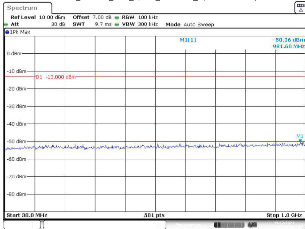
Band 2_20 MHz_Low_QPSK_RB100#0_1(30MHz-1GHz)
