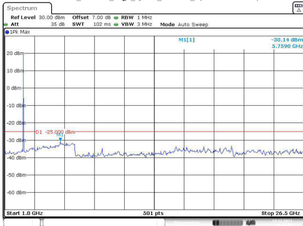
Band 38_10 MHz_High_QPSK_RB50#0_2(1GHz-26.5GHz)
