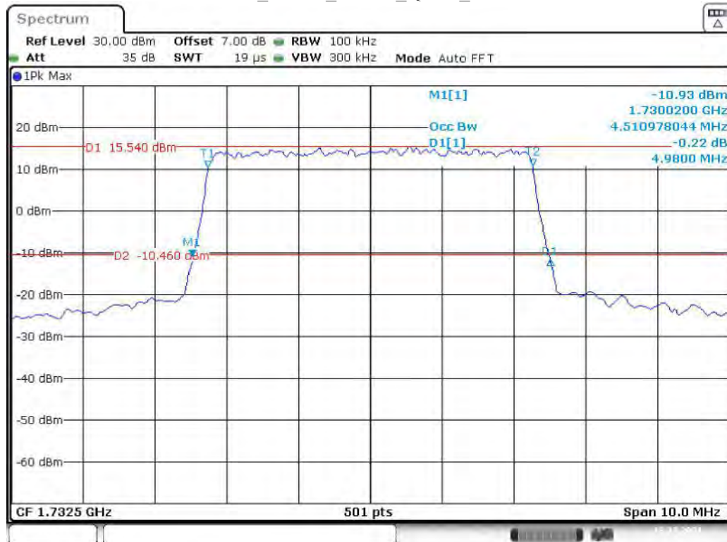
Band 4_5 MHz_Middle_QPSK_RB25#0
