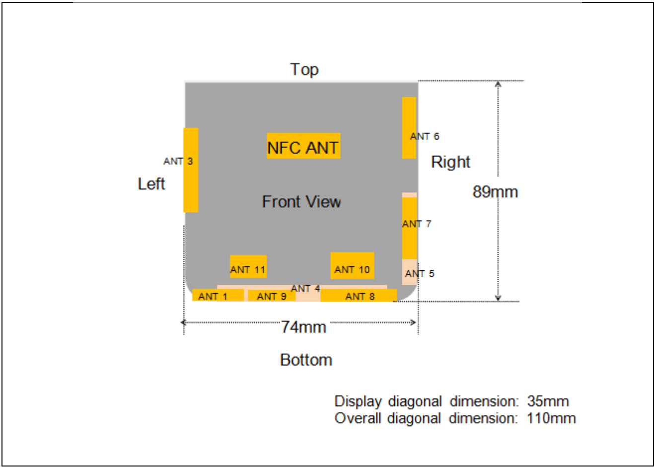
Fig.14.2 EUT Closed Mode Antenna Locations
