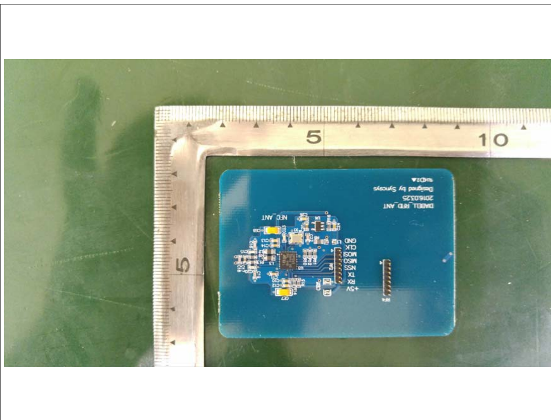
View of RFID PCB (Top)
