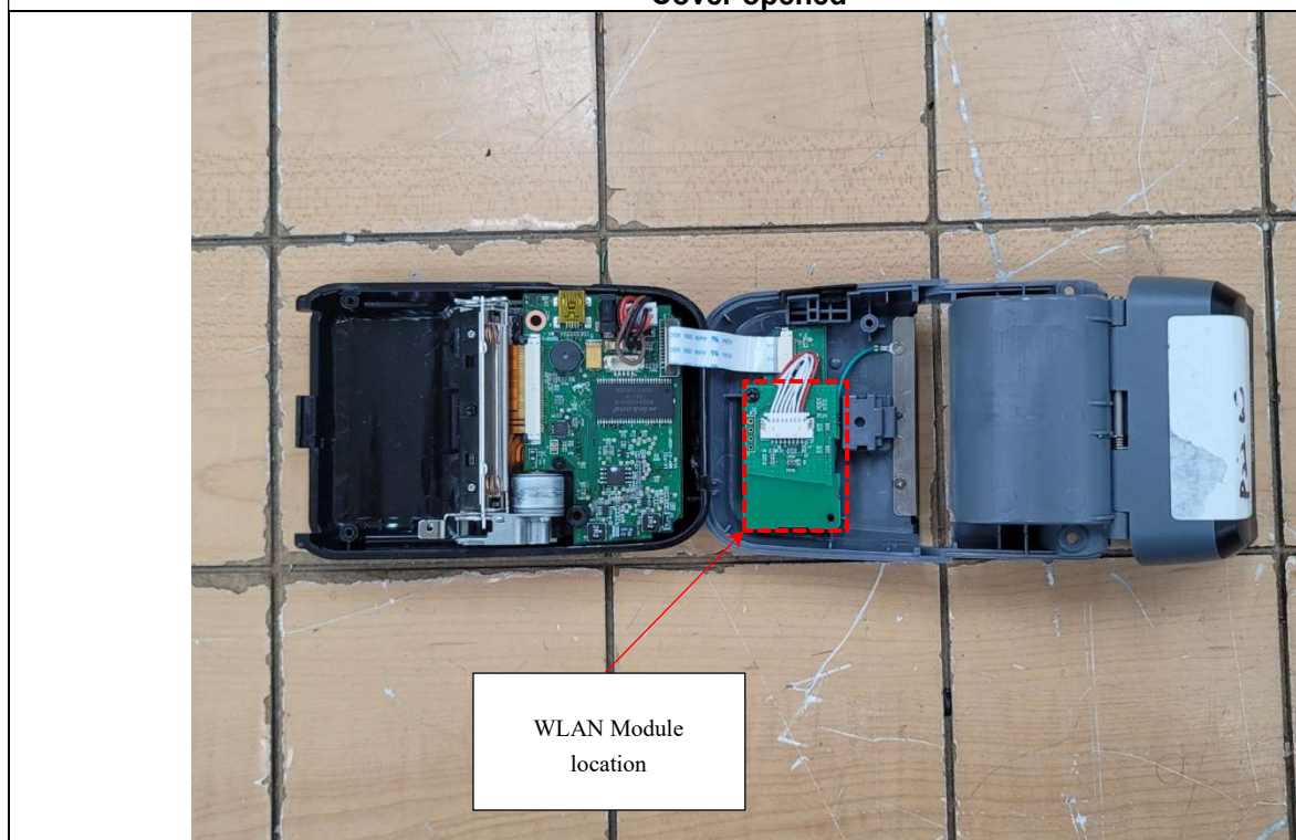
Cover opened
