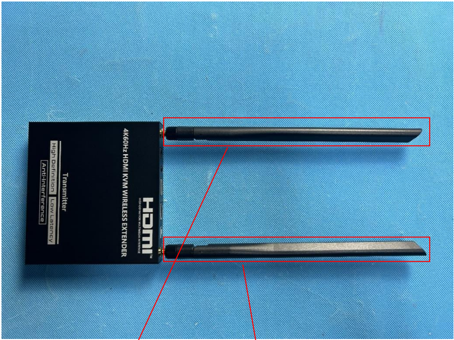
WIFI 2 Antenna
