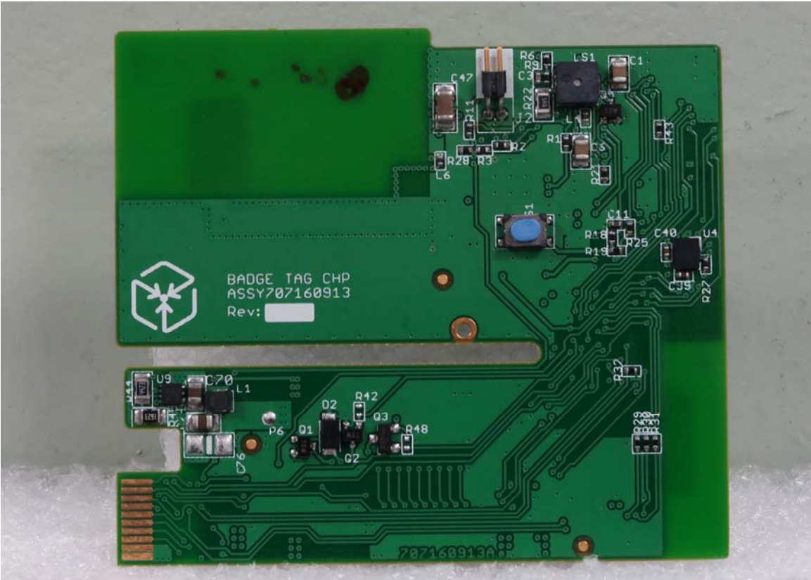
PCB Front
