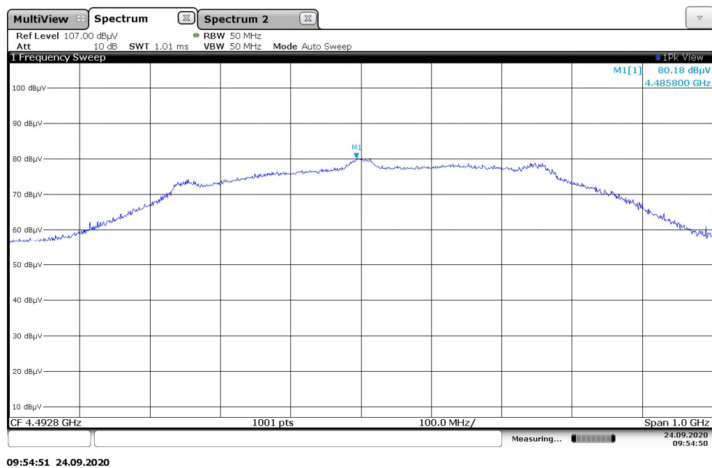
Figure 7.4.2-2: Peak Power Plot – Channel 3
