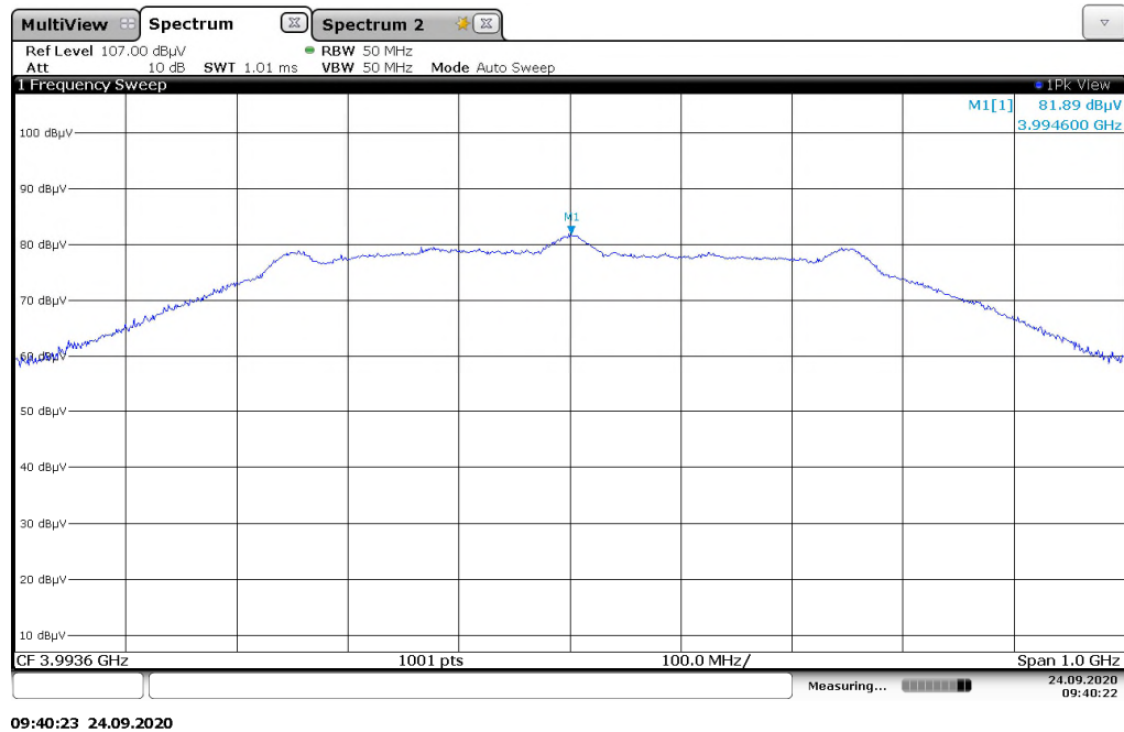
Figure 7.4.2-1: Peak Power Plot – Channel 2
