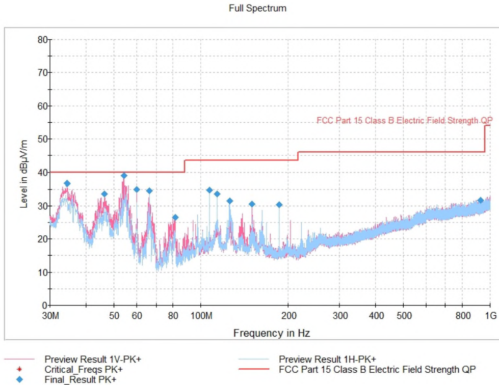
Figure 7.6.2-2: Emission Profile 30MHz-1GHz – Channel 3
