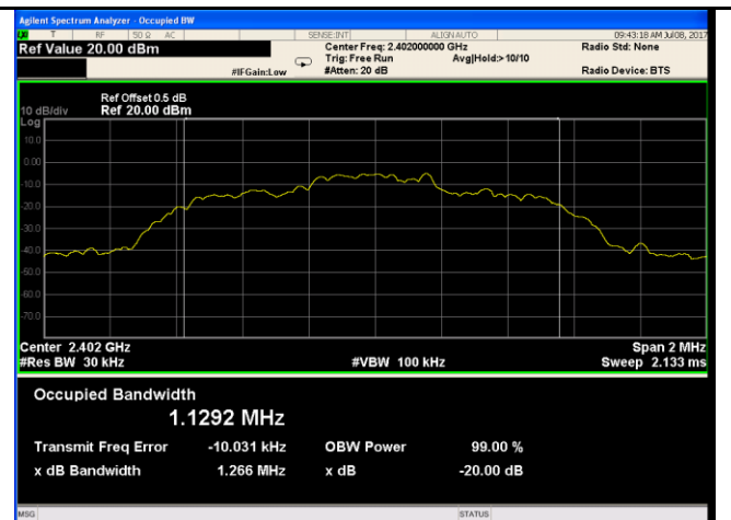
\pi/4 DPSK - Low Channel
