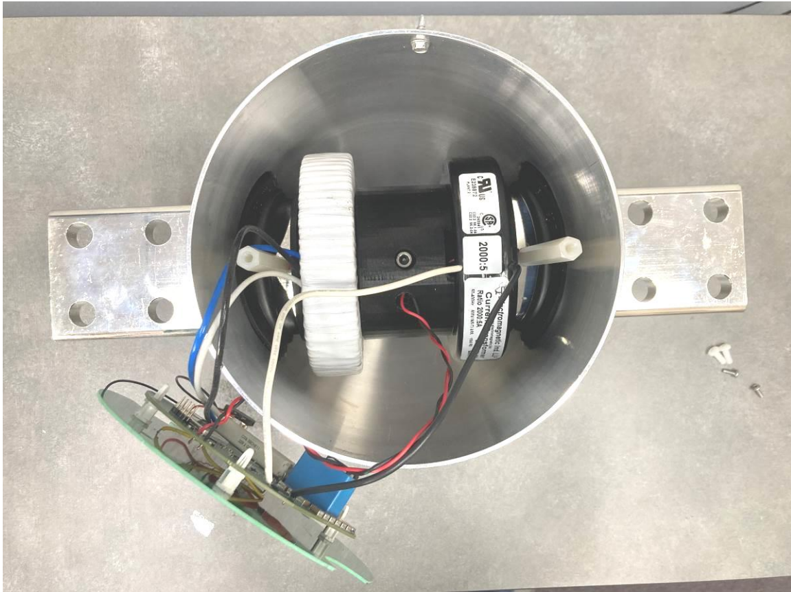
Figure 12. Inside the case
