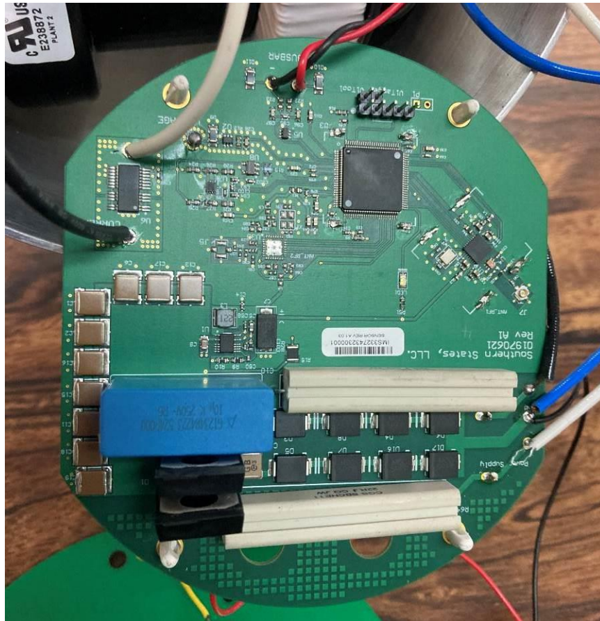
Figure 9. PCB Board 2 (Sensor board), Component side with Shielding Removed from Transmitter circuitry
