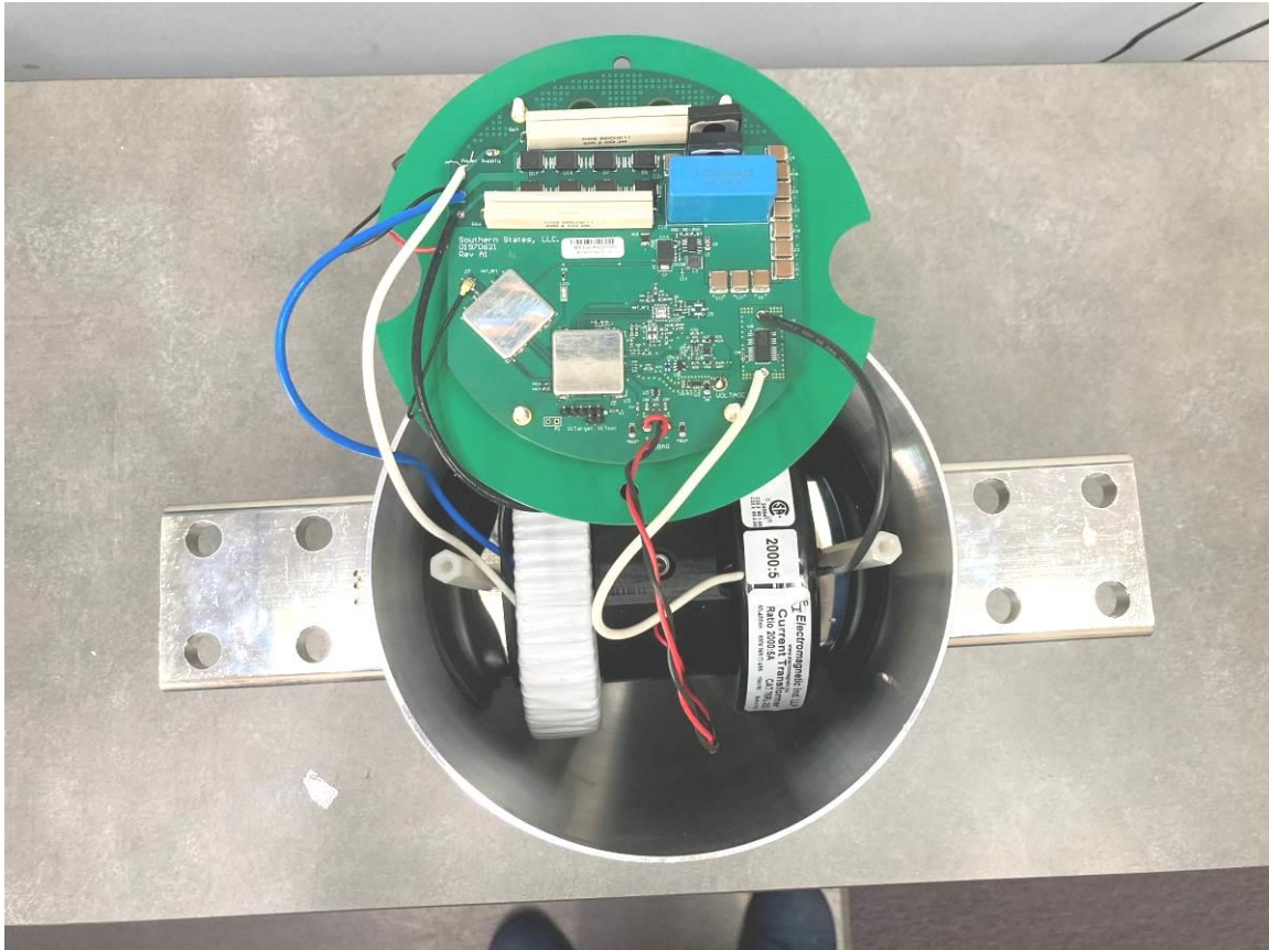
Figure 3. Zoomed Out view of PCB assembly unmounted
