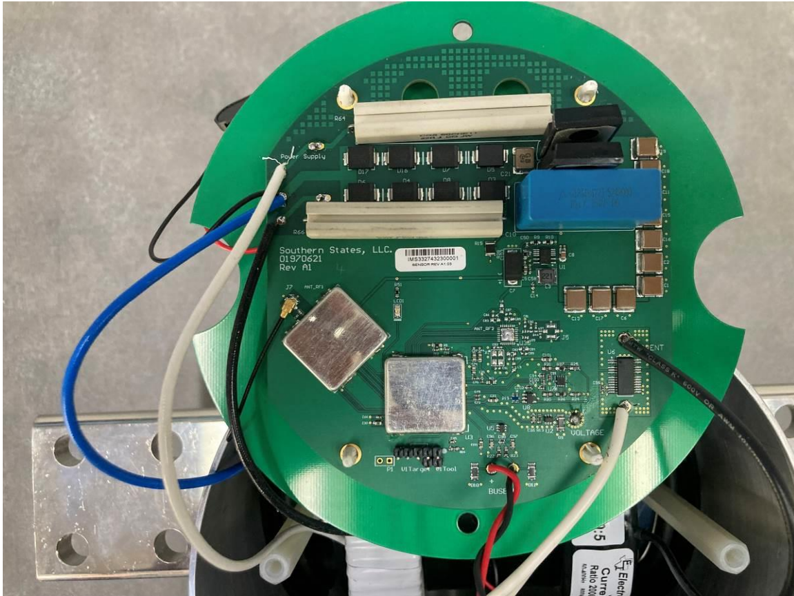
Figure 2. PCB assembly unmounted
