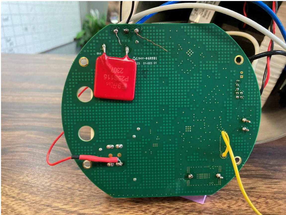
Figure 7. PCB Board 2 (Sensor board), Solder side
