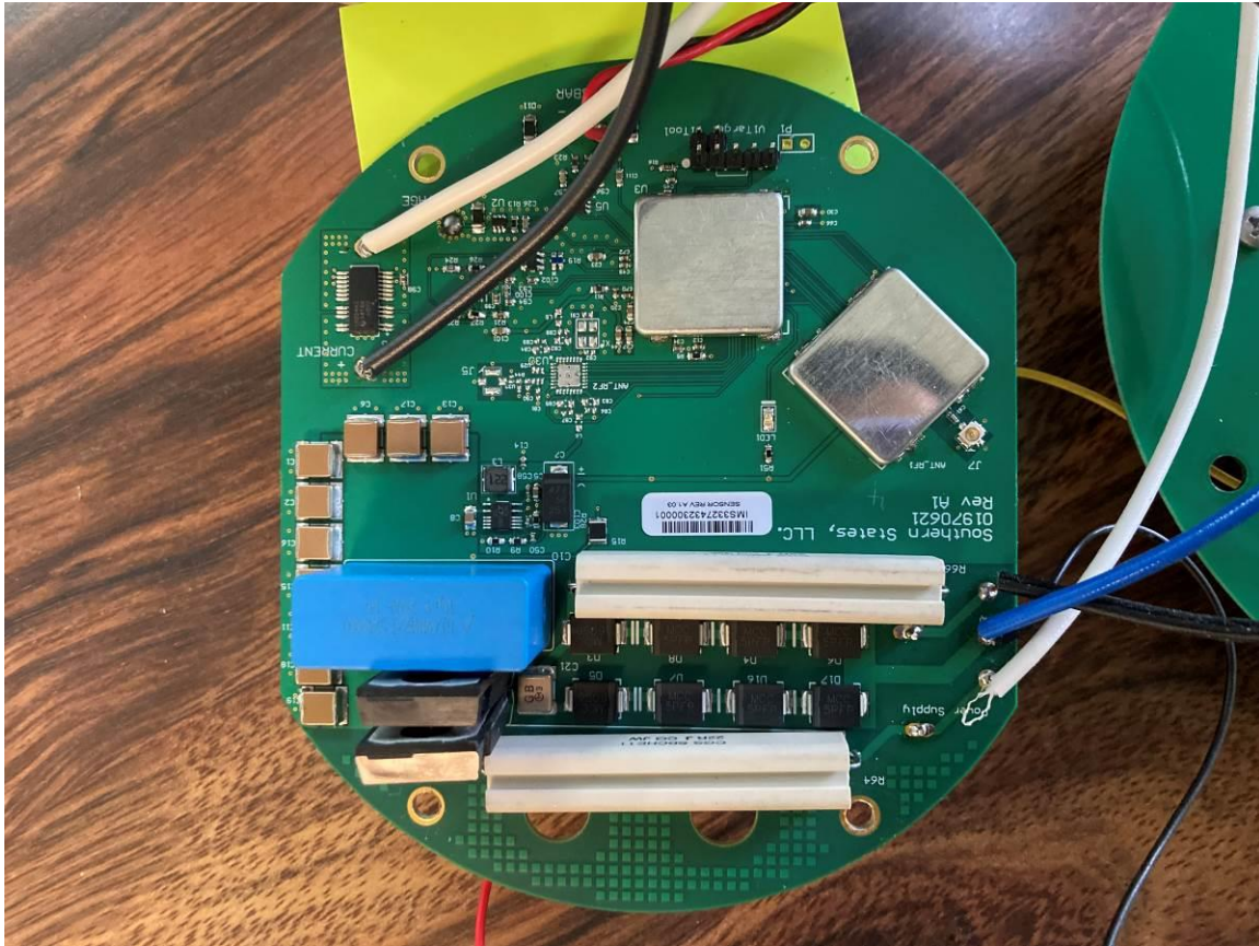
Figure 8. PCB Board 2 (Sensor board), Component side
