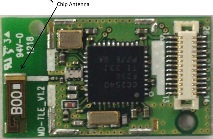
Chip Antenna
