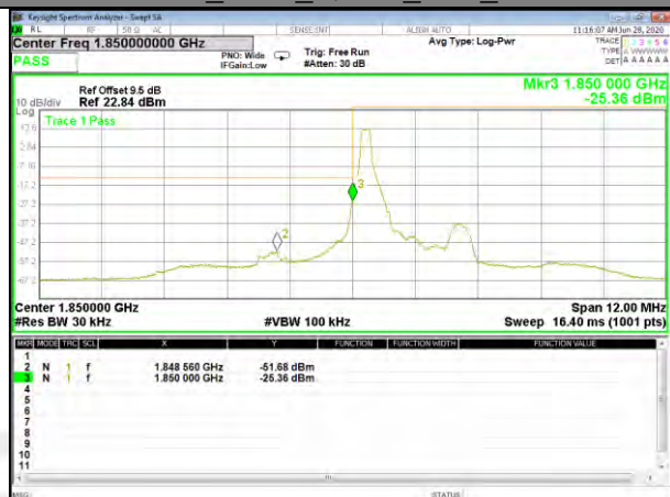
Band2_1.4M_QPSK_Low_Full-RB
