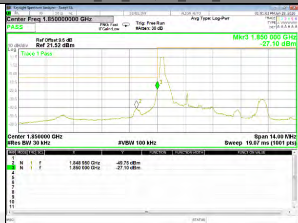
Band2_3M_16QAM_Low_Full-RB
