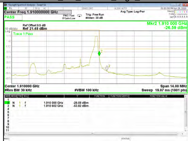
Band2_3M_16QAM_High_1-RB
