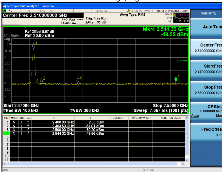
GFSK: Band Edge, Right Side
