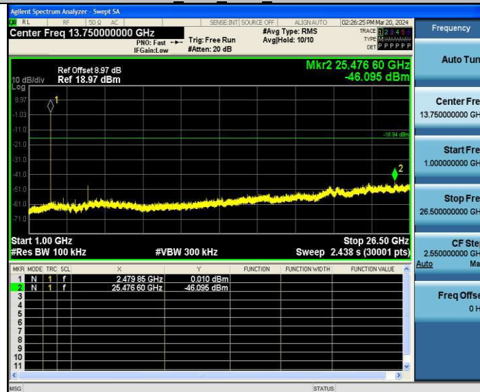
3DH5_Ant2_2480_0~Reference
