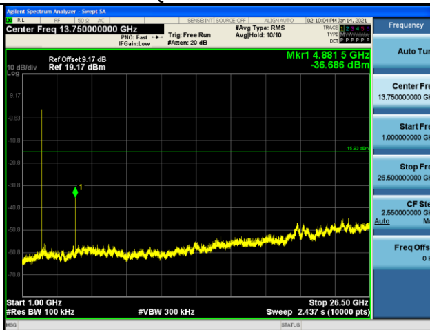
4/π-DQPSK on Channel 39
