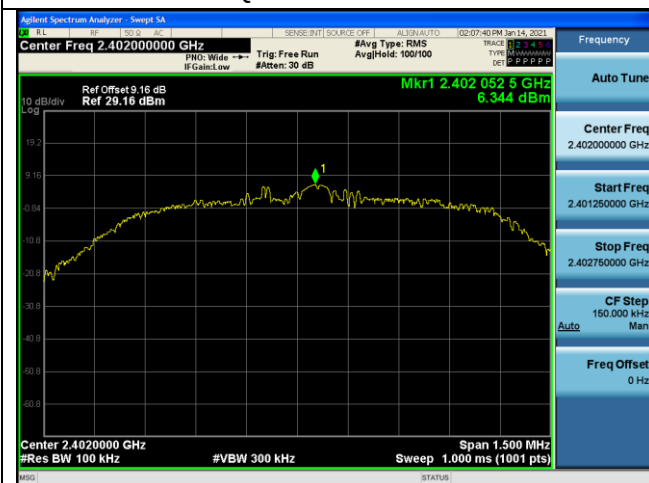
4/π-DQPSK on Channel 00
