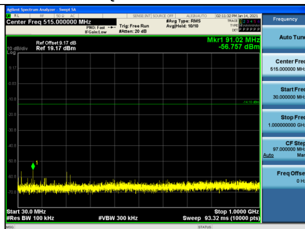
4/π-DQPSK on Channel 78
