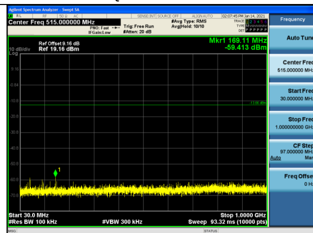
4/π-DQPSK on Channel 00
