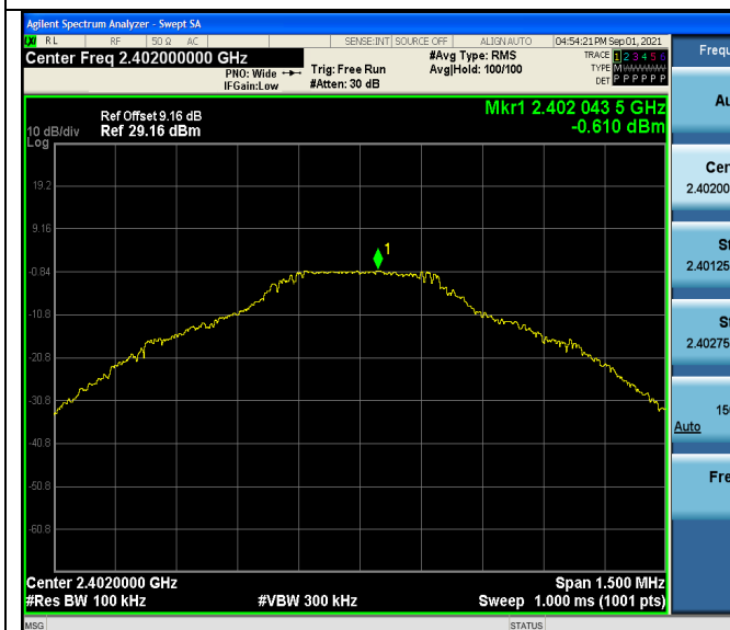
GFSK on Channel 00
