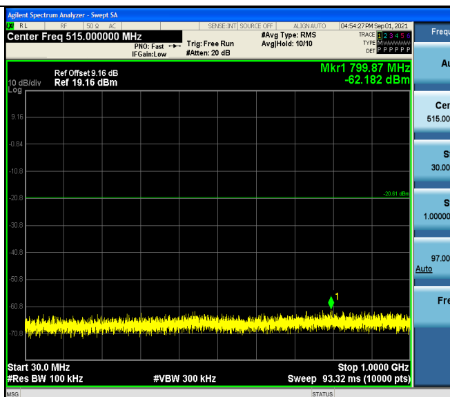
GFSK on Channel 39
