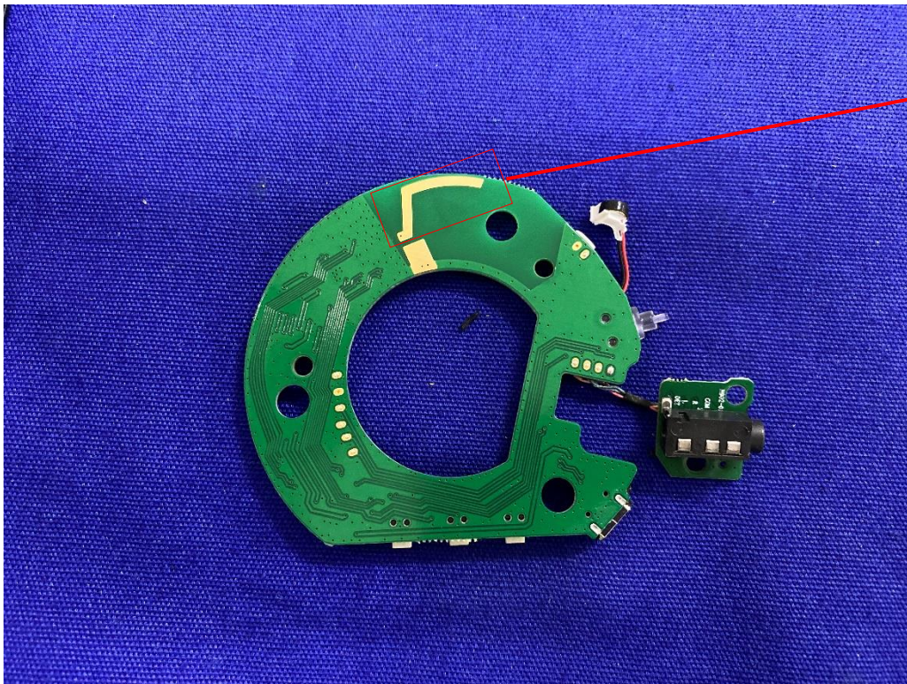
Bluetooth Antenna
